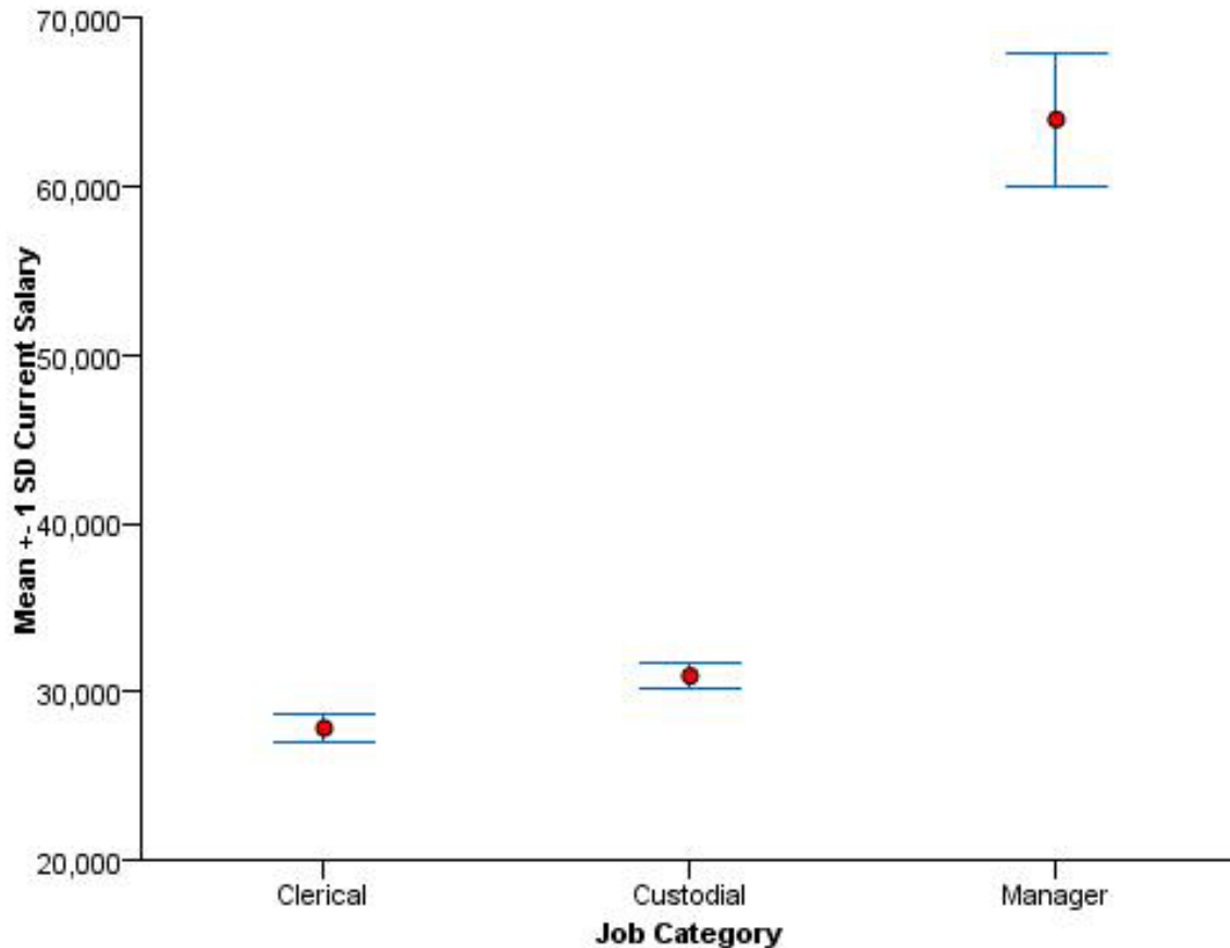
Figure 398. Error bar chart
