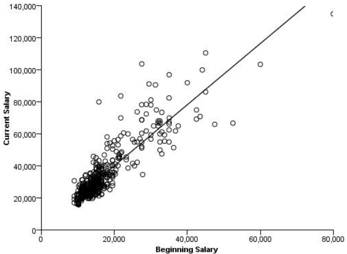
Figure 430. Simple scatterplot with fit line
