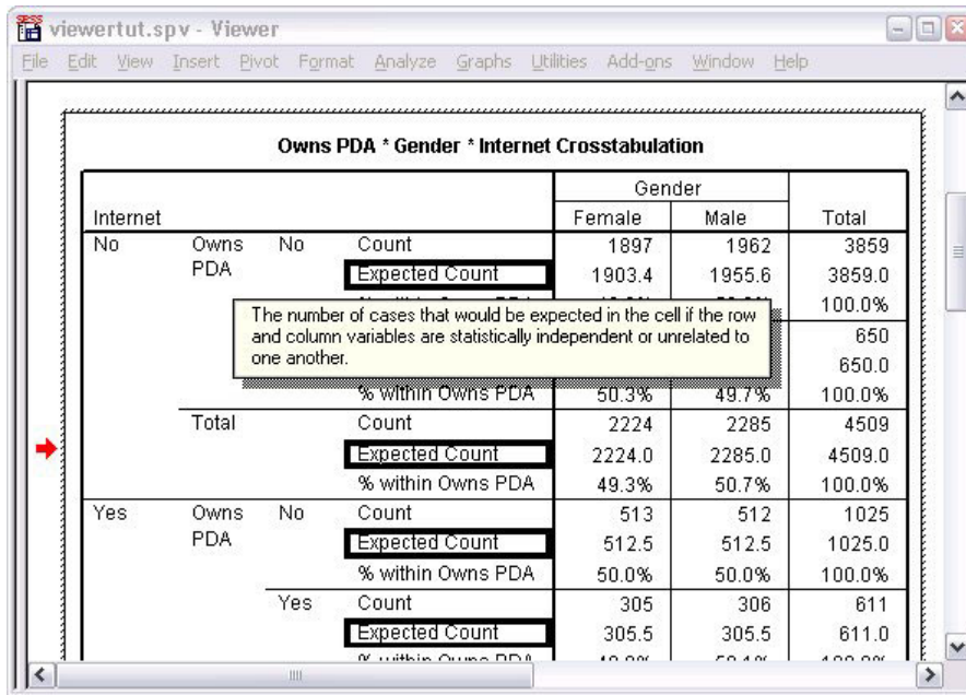
Figure 37. Pop-up definition
