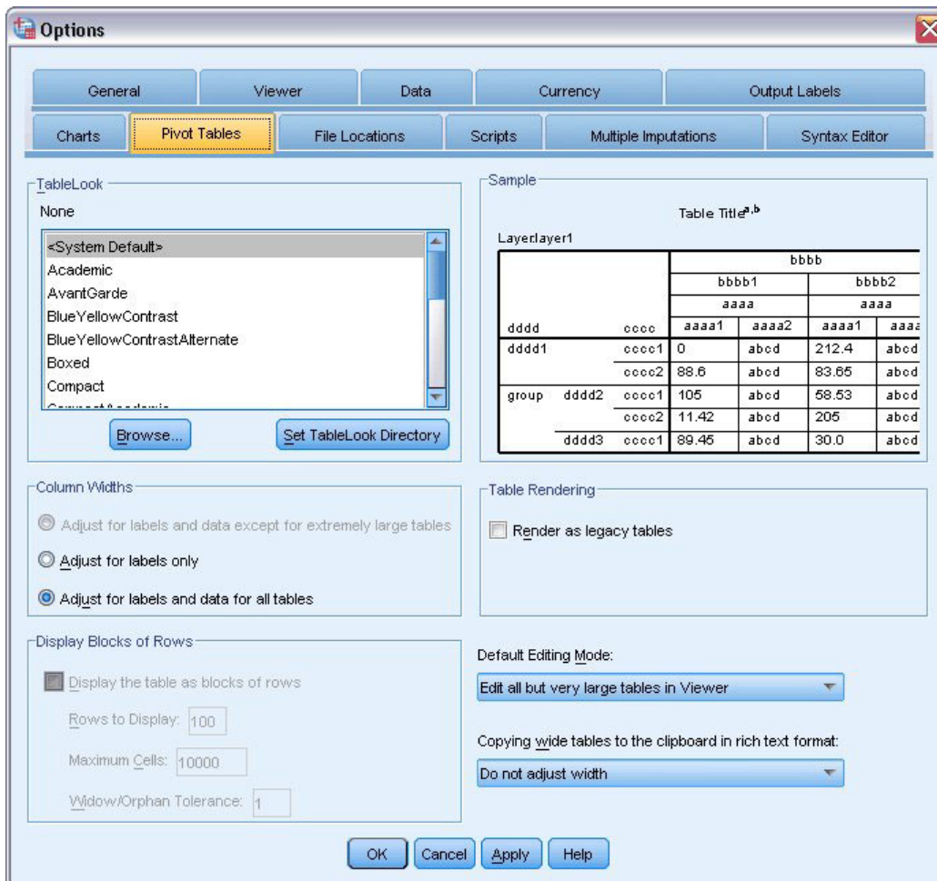
Figure 49. Options dialog box
