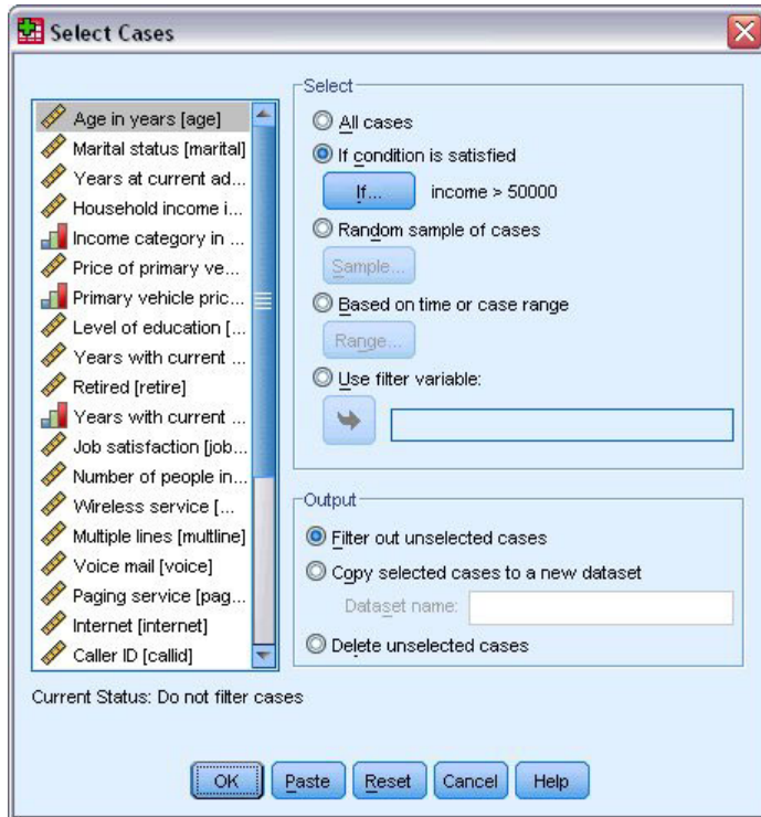
Figure 82. Select Cases dialog box
