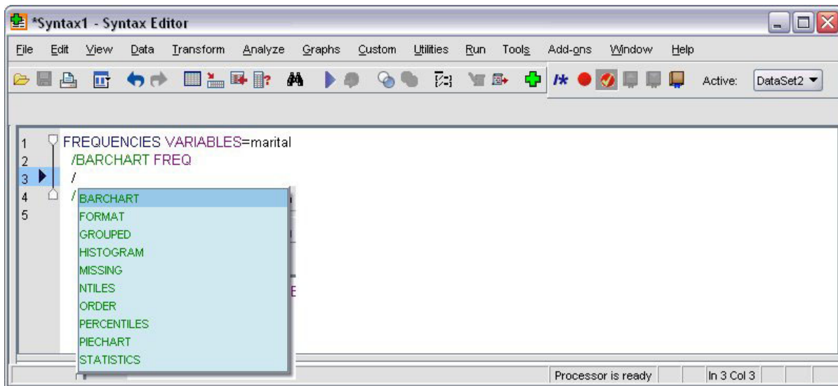
Figure 69. Auto-completion control displaying subcommands
