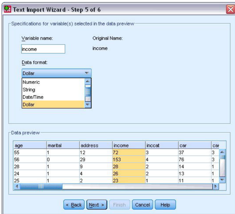
Figure 16. Change the data type
