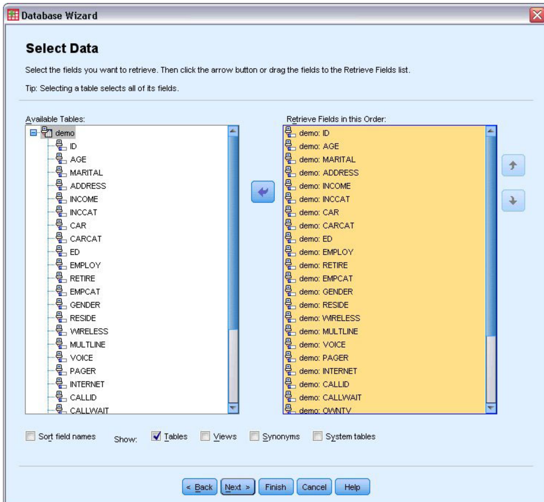
Figure 13. Select Data step
