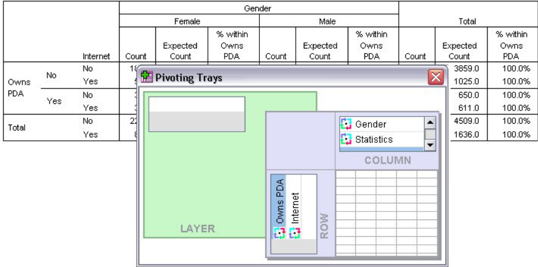
Figure 39. Swap rows
