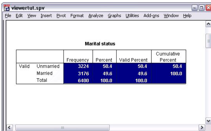
Figure 48. Custom TableLook
