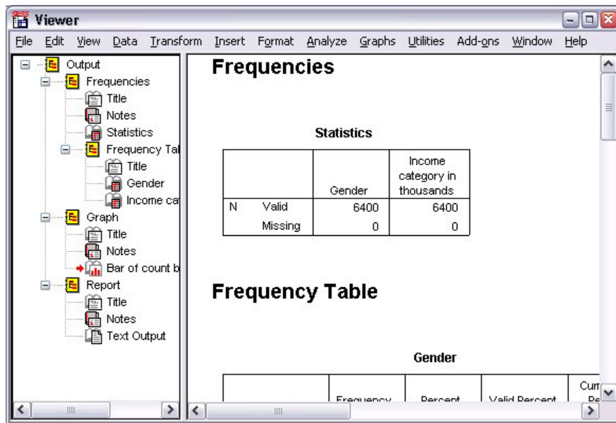
Figure 54. Viewer
