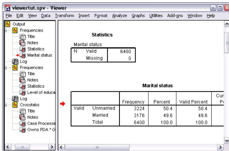
Figure 35. Viewer
