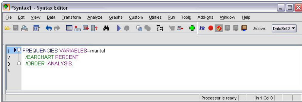
Figure 68. Frequencies syntax
