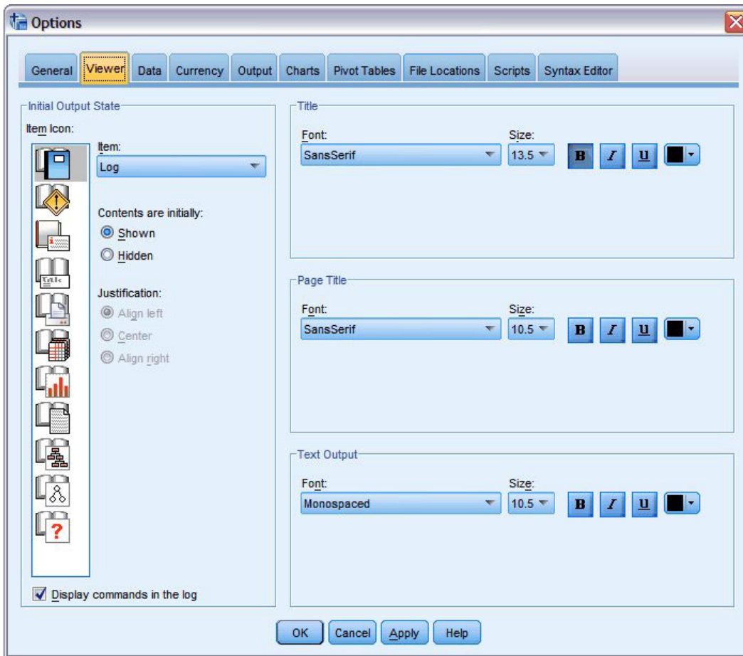
Figure 50. Viewer options
