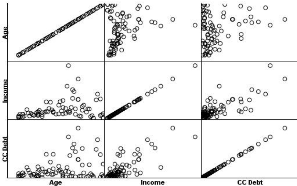
Figure 436. Scatterplot Matrix
