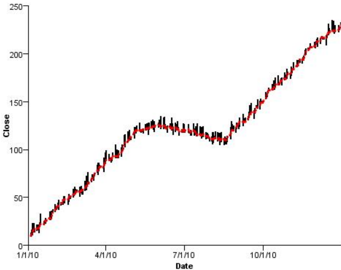
Figure 424. High-low-close chart
