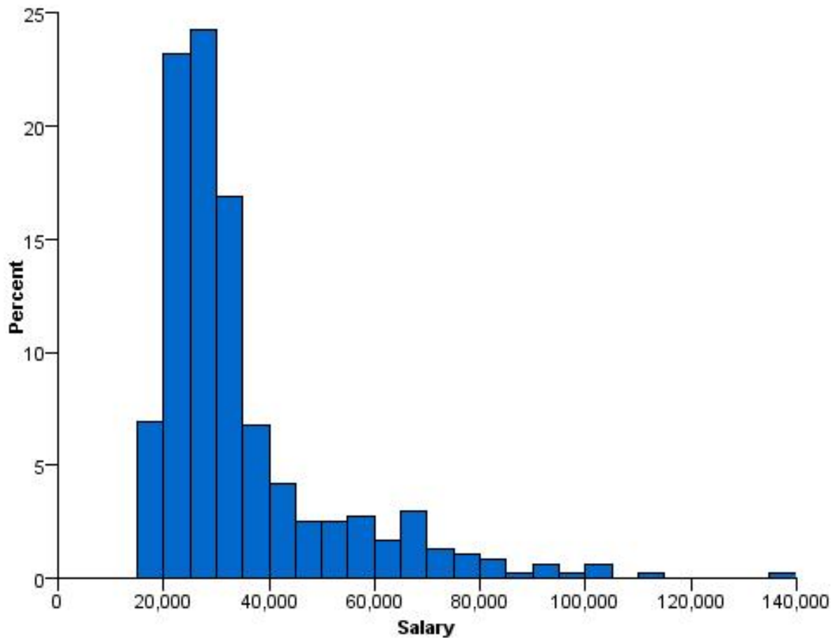
Figure 406. Percentage histogram
