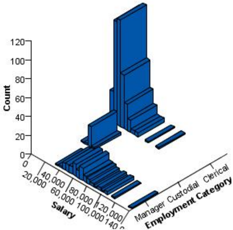
Figure 418. 3-D histogram
