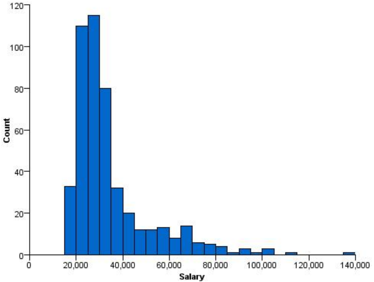
Figure 400. Histogram
