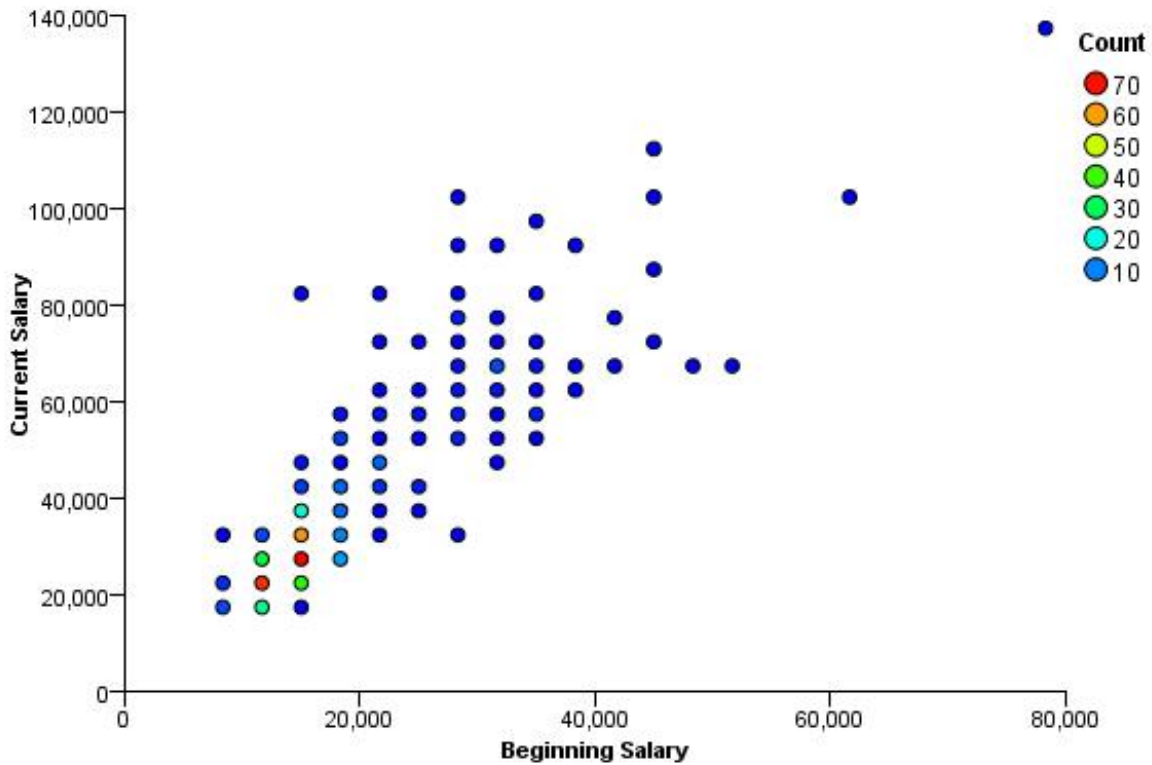
Figure 440. Binned scatterplot
