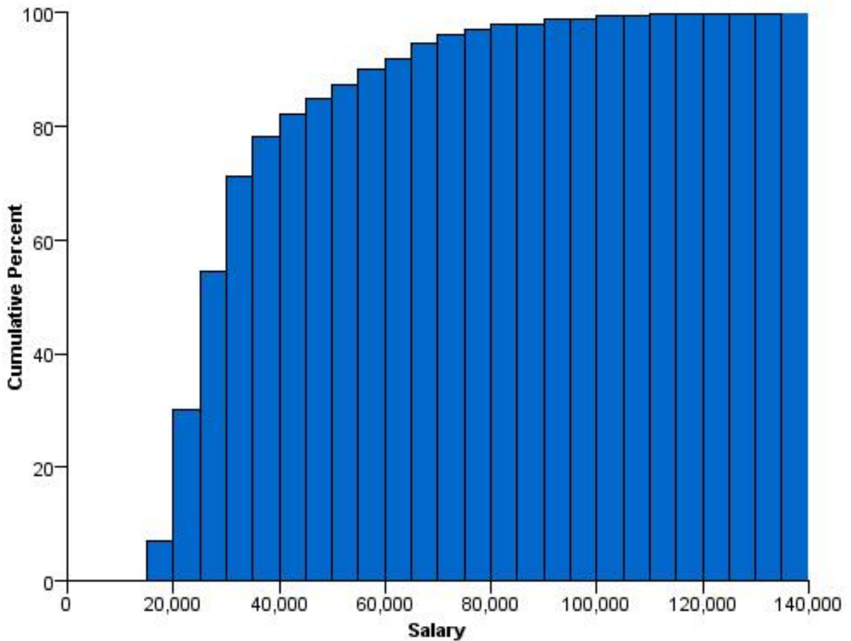
Figure 416. Cumulative histogram
