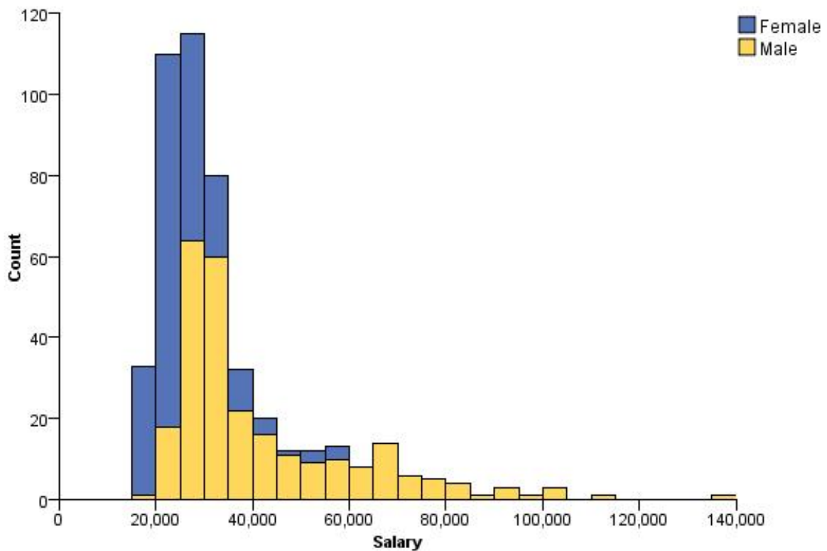
Figure 410. Stacked histogram
