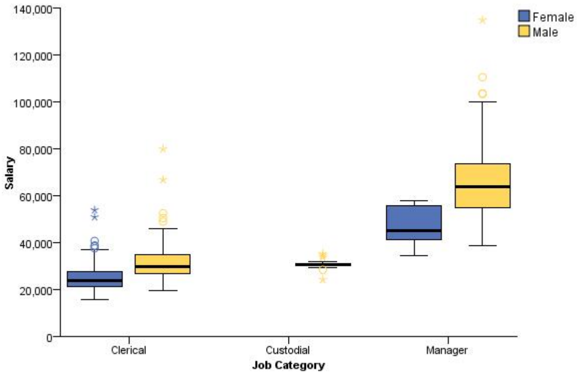
Figure 487. Clustered boxplot
