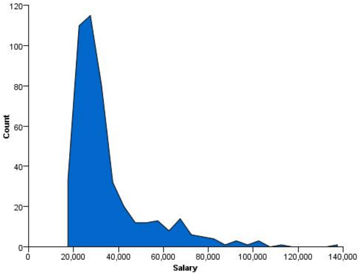
Figure 408. Frequency polygon
