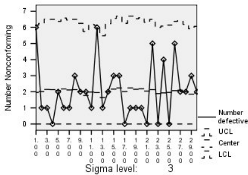
Figure 94. A np chart
