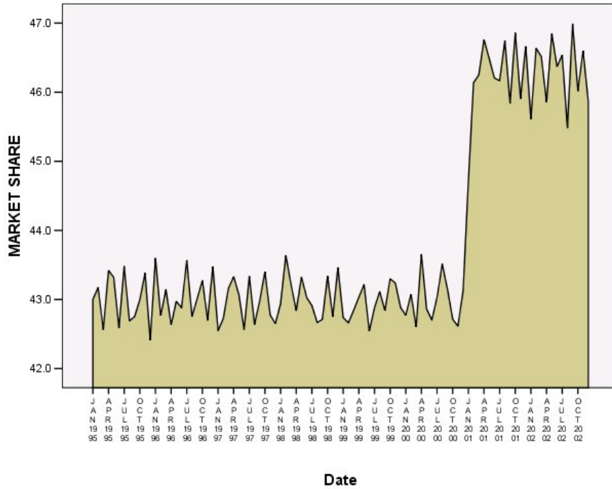
Figure 99. FORMAT=BOTTOM
