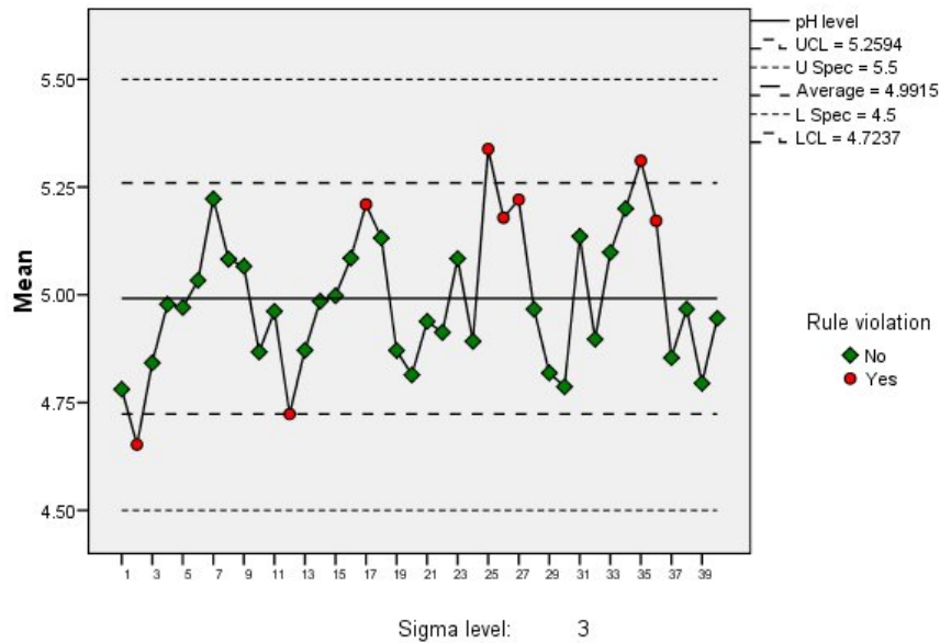
Figure 88. X-bar chart
