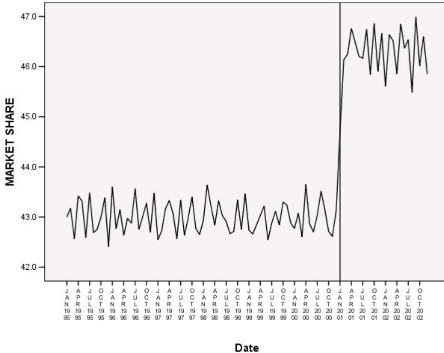
Figure 102. MARK=Y 2001 M 1
