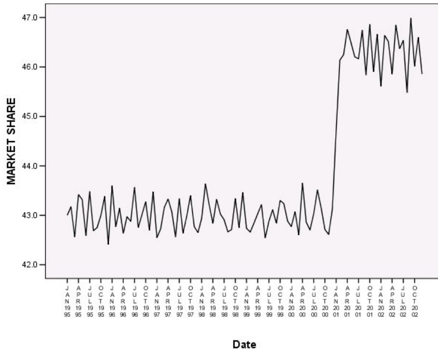
Figure 98. TSPLLOT VARIABLES=SHARE
