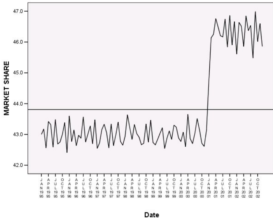
Figure 100. FORMAT=REFERENCE
