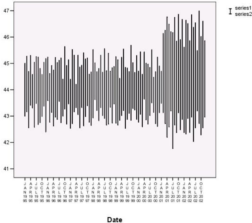
Figure 101. FORMAT=HILO
