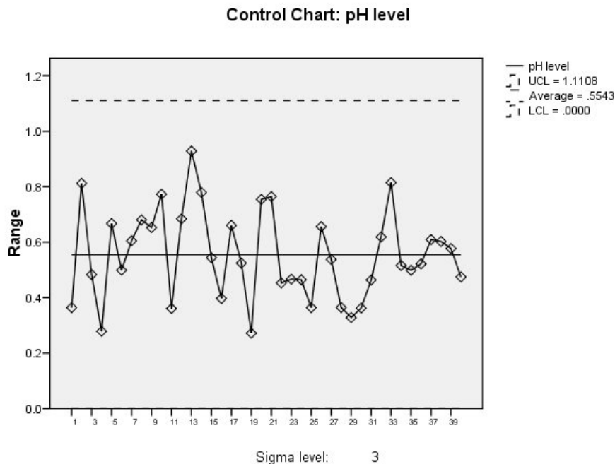
Figure 89. R chart
