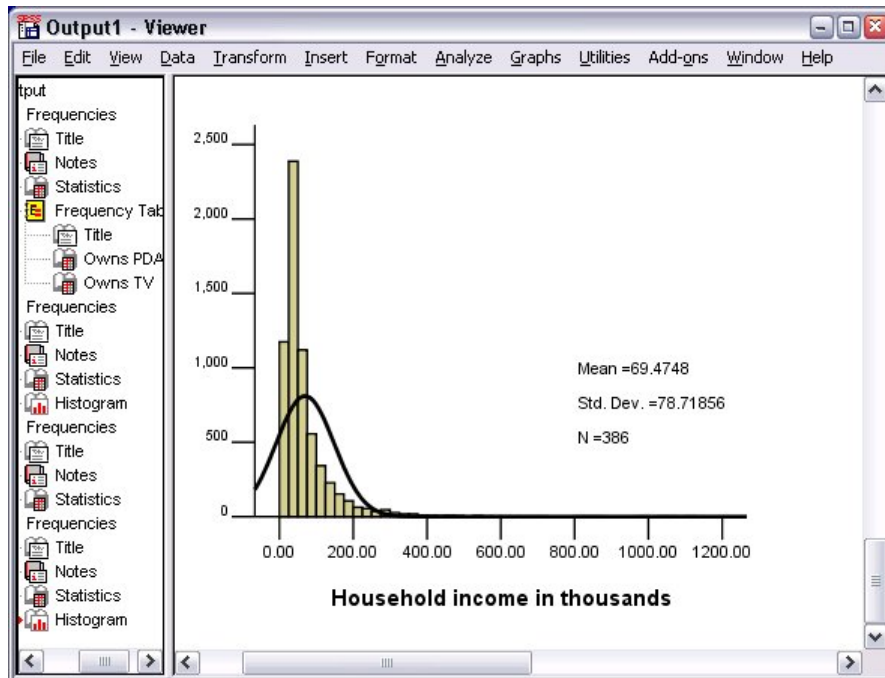
Figure 31. Histogramme
