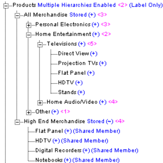
Figure 1 Aggregate storage Outline Displaying the Alternate Hierarchy High End Merchandise on the Product Dimension of ASOsamp Sample
