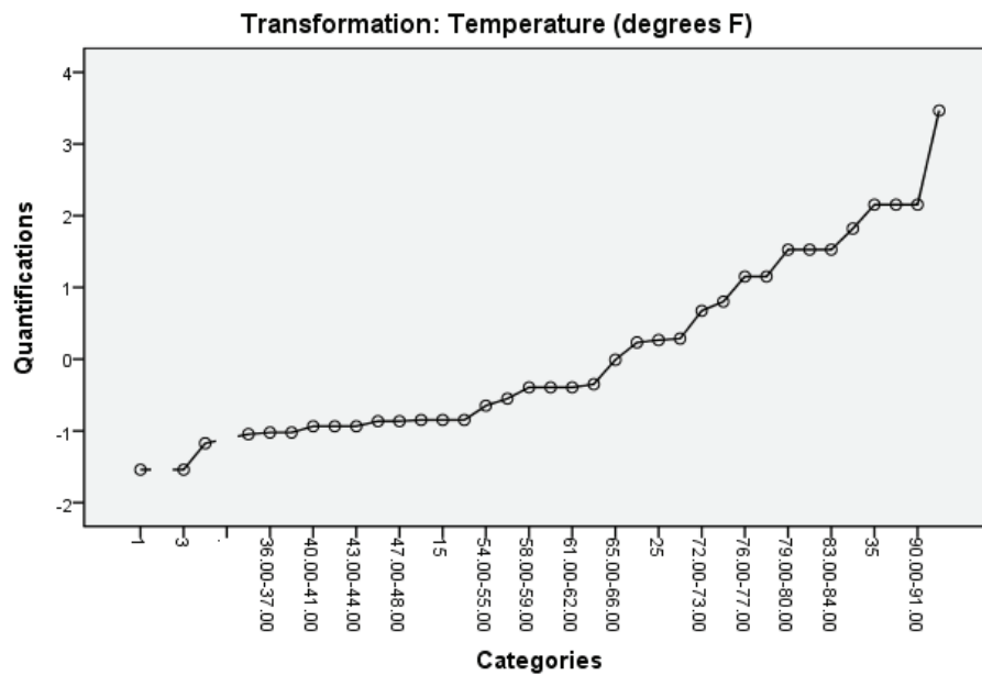
Figure 9-42 Transformation plot of Temperature (ordinal)
