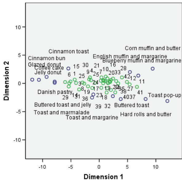
Figure 15-22
