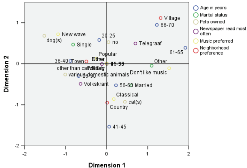
Figure 11-32 Centroids labeled by variables (age nominal)
