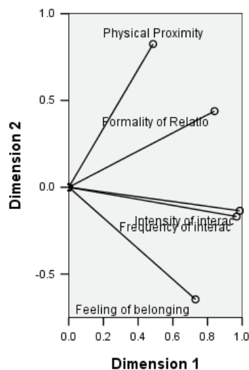
Figure 10-13 Component loadings
