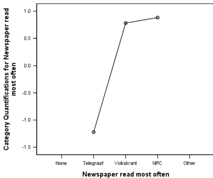
Figure 11-19 Transformation plot for Newspaper read most often (nominal)
