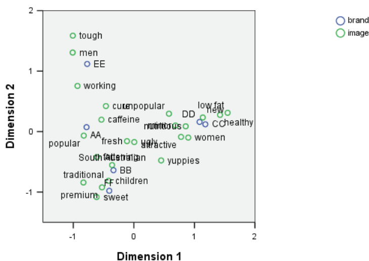
Figure 12-13
