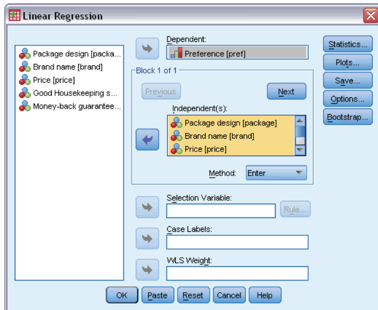
Figure 9-1
