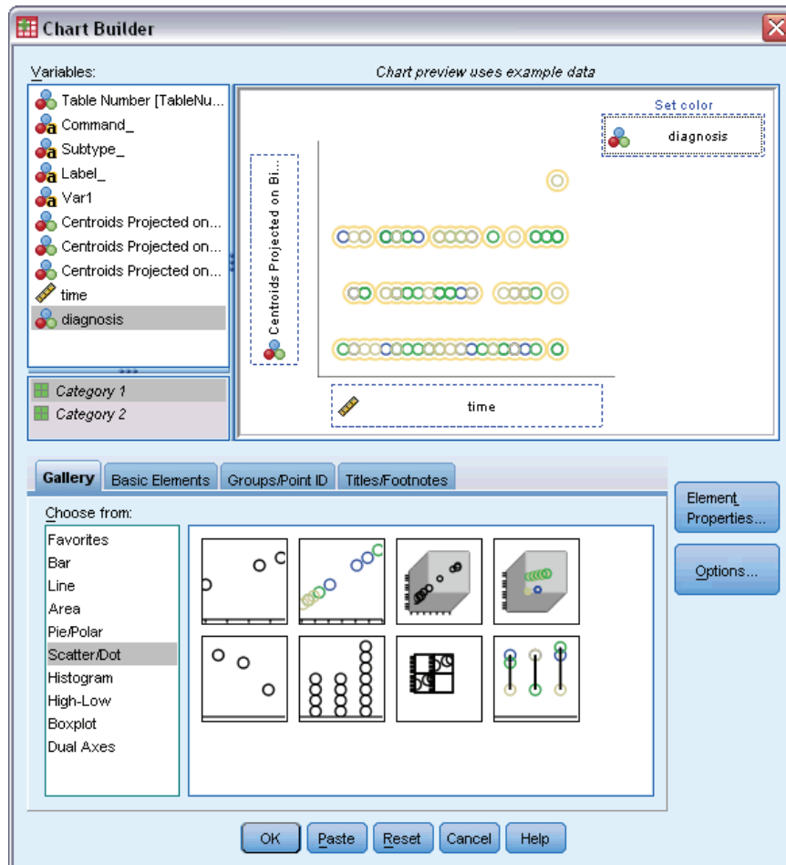
Figure 10-53 Chart Builder
