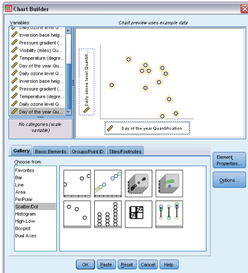
Figure 9-56 Chart Builder
