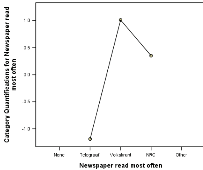
Figure 11-30 Transformation plot for Newspaper read most often (age nominal)
