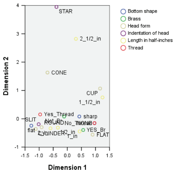
Figure 13-8 Category quantifications
