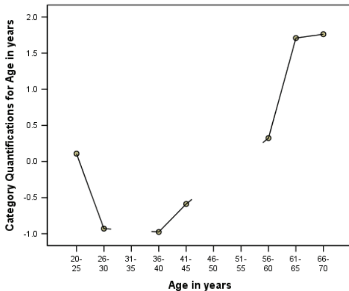
Figure 11-28 Transformation plot for Age in years (nominal)
