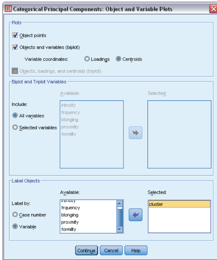
Figure 10-5 Object and Variable Plots dialog box
