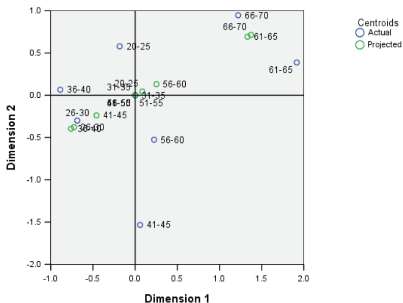
Figure 11-31
