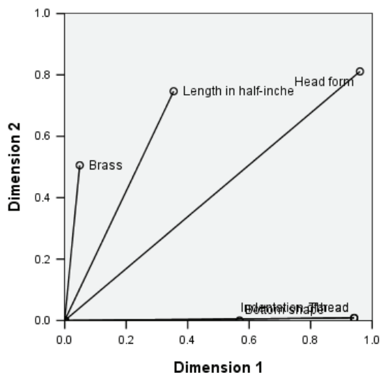
Figure 13-16 Discrimination measures
