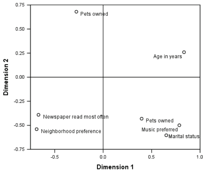
Figure 11-17 Component loadings
