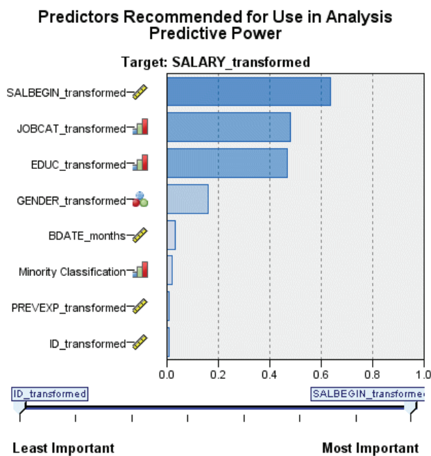
Figure 4-17 Predictive Power
