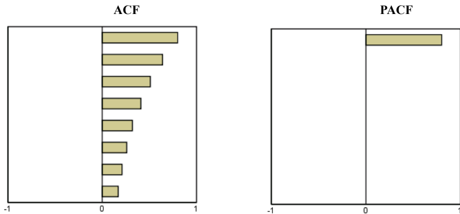
ARIMA(1,0,0), \phi > 0
