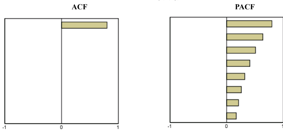
ARIMA(0,0,1), \theta < 0
