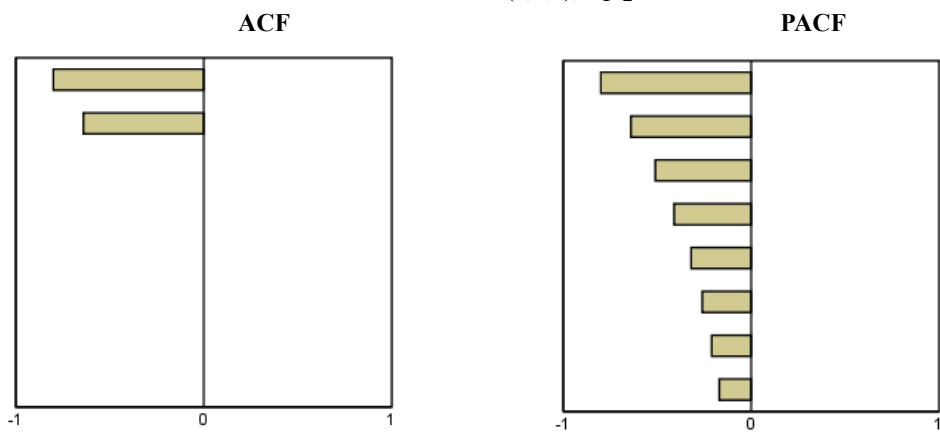
ARIMA(0,0,2), \theta_1\theta_2 > 0
