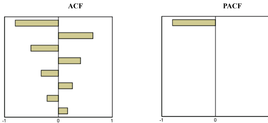
ARIMA(1,0,0), \phi < 0
