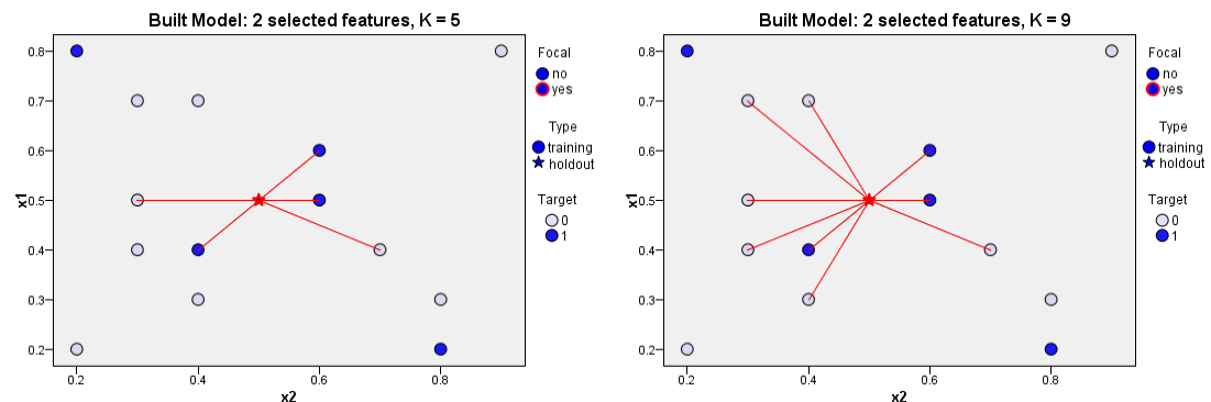
Figure 121-1 The effects of changing k on classification
