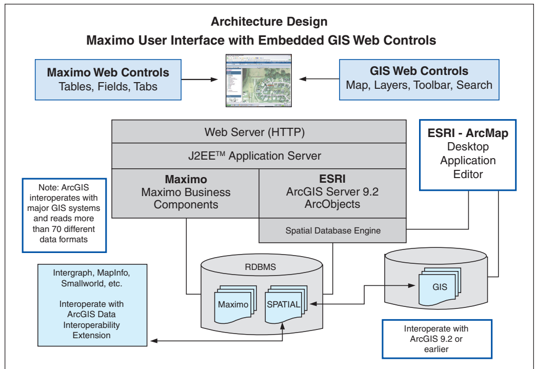
Figure 8: Maximo Spatial Asset Management architecture
