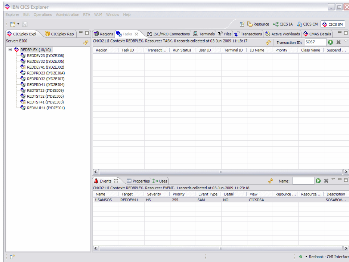
Figure 16-1 SOS Condition
