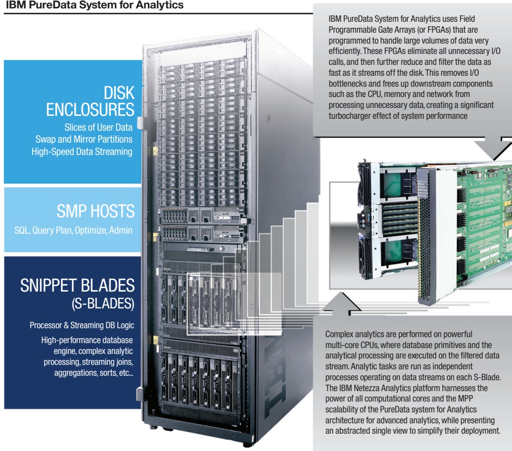
Figure 1: IBM PureData System for Analytics
