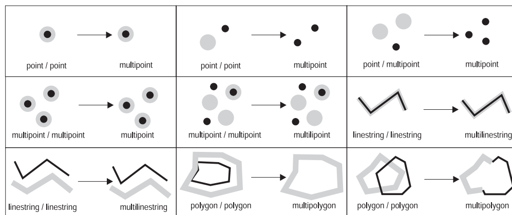
Figure 55. ST_Union
