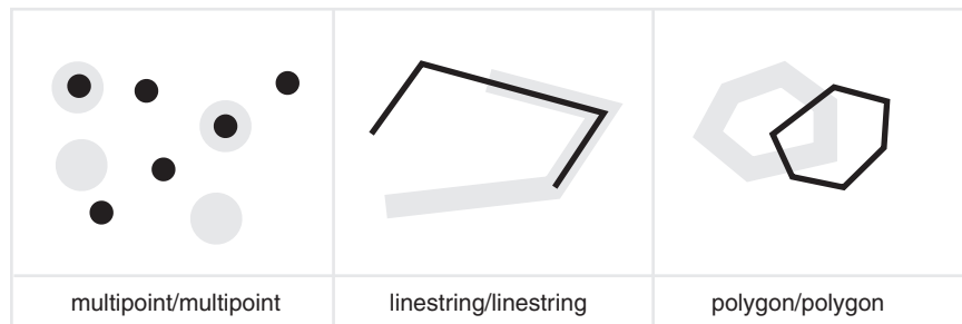
Figure 47. ST_Overlaps
