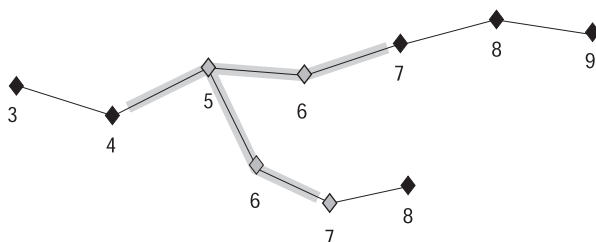
Figure 56. LocateBetween
