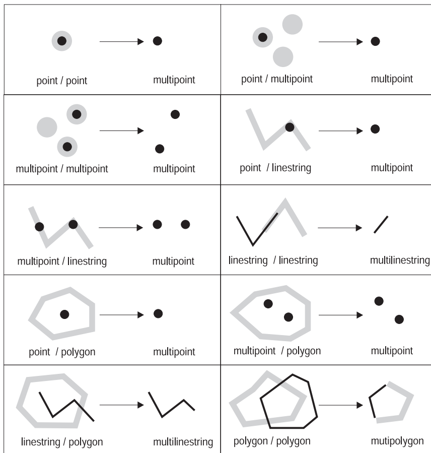
Figure 54. ST_Intersection
