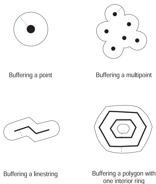
Figure 51. ST_Buffer
