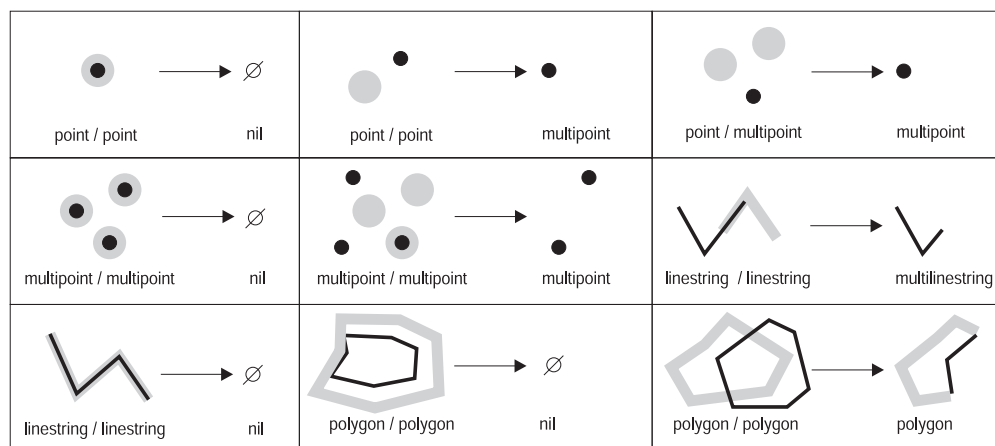
Figure 53. ST_Difference
