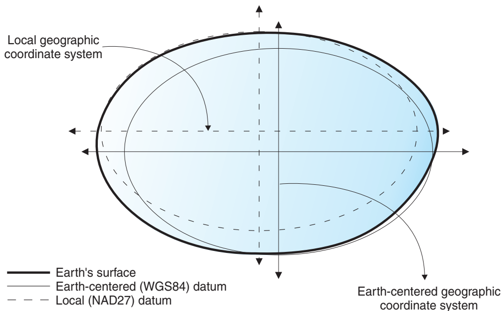
Figure 11. Datum alignments
