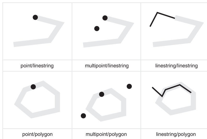
Figure 48. ST_Touches
