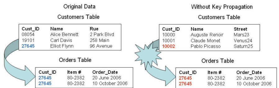
Figure 2. Without a Key Propagation capability, critical data relationships would be severed.
