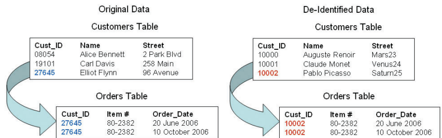
Figure 1. Optim's Key Propagation capability ensures referential integrity, even when data is masked.
