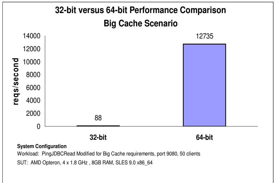
Figure 1: Leveraging a large heap for performance
