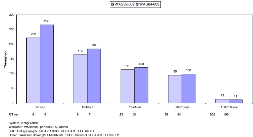
Figure 3: Web services security performance – POWER
