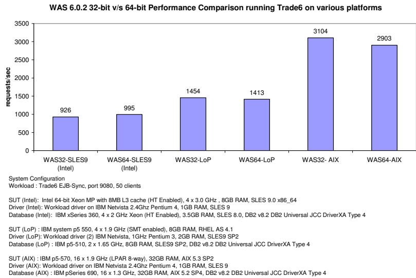
Figure 11: POWER vs. x86-64 performance
