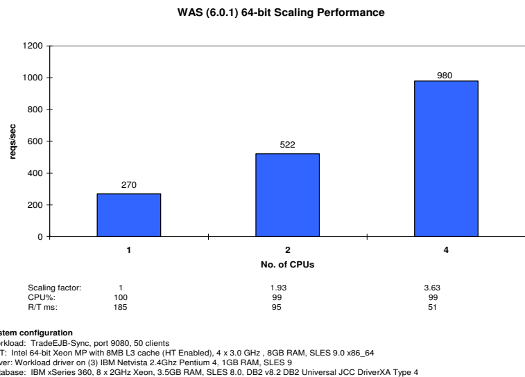
Figure 10: WAS Vertical scalability on x86-64
