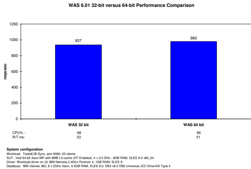
Figure 7: Trade6 64-bit performance on x86-64
