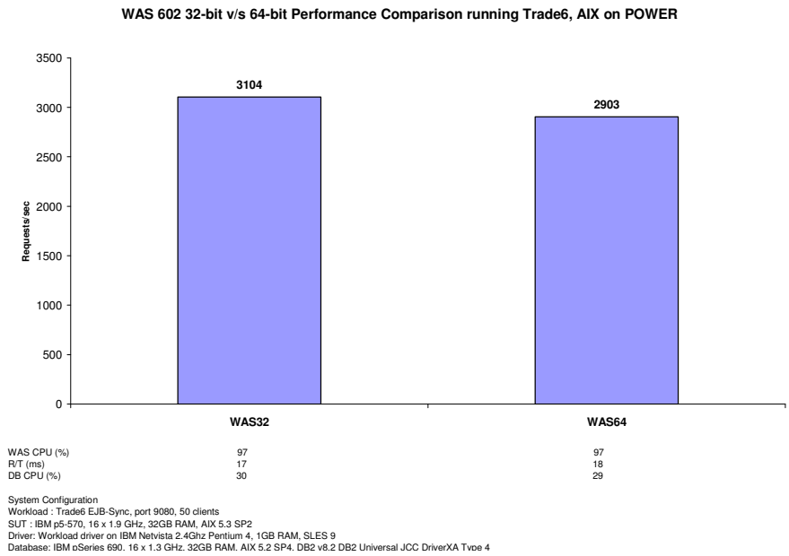
Figure 6: Trade6 64-bit performance on AIX on POWER
