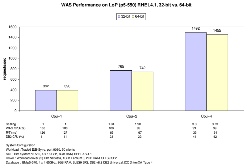
Figure 8: WAS Vertical Scalability on Linux on POWER
