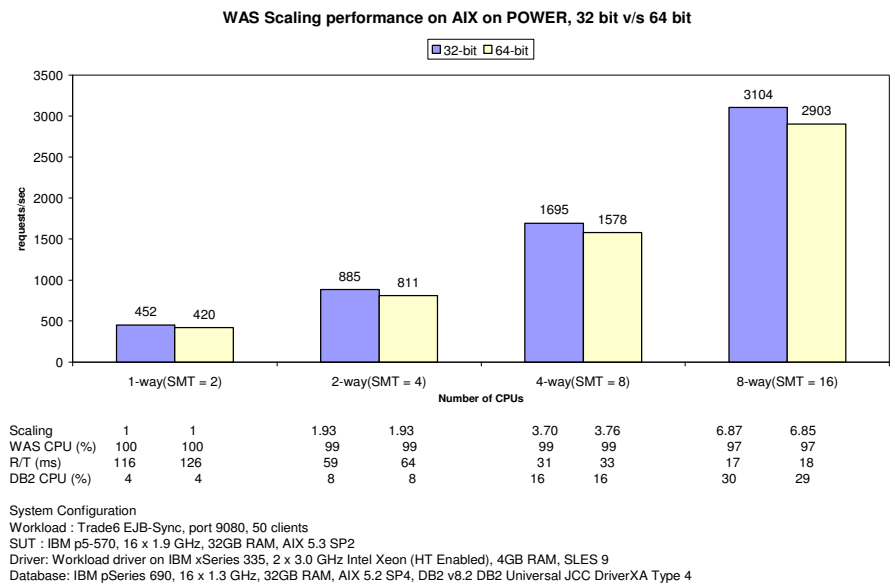
Figure 9: WAS Vertical Scalability on AIX on POWER
