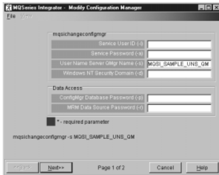
Figure 7. Modify Configuration Manager
