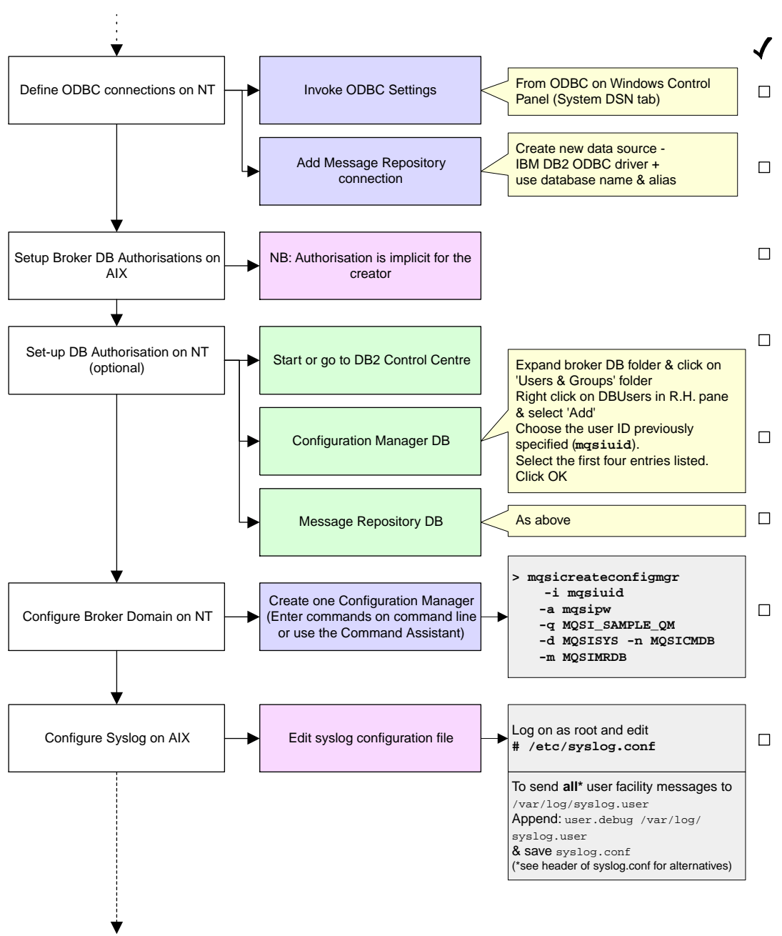
Figure 2. Configuring a simple broker domain continued
