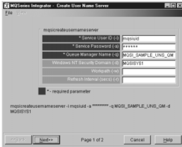
Figure 9. Create User Name Server
