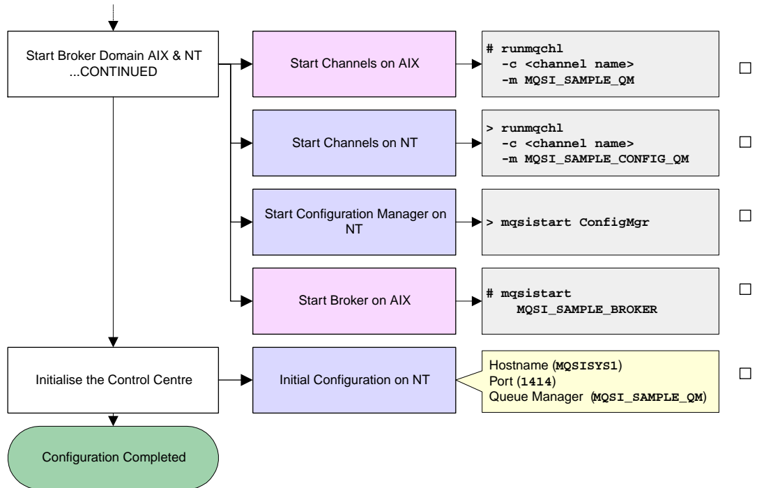
Figure 4. Configuring a simple broker domain continued
