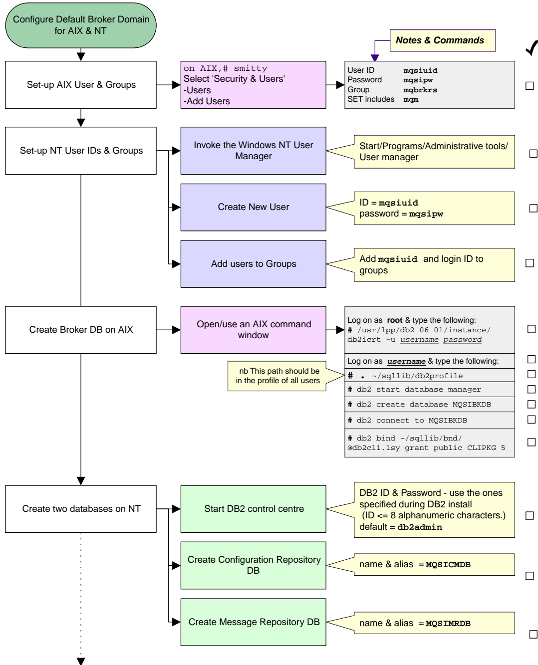
Figure 1. Configuring a simple broker domain
