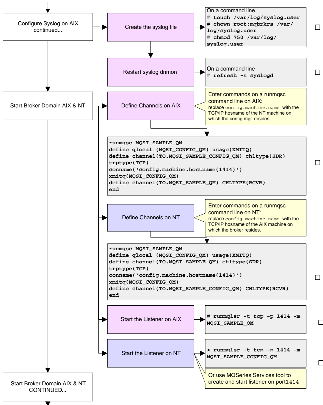
Figure 3. Configuring a simple broker domain continued
