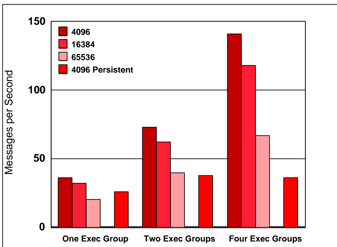
Figure 11: Additional Execution Group Throughput Results
