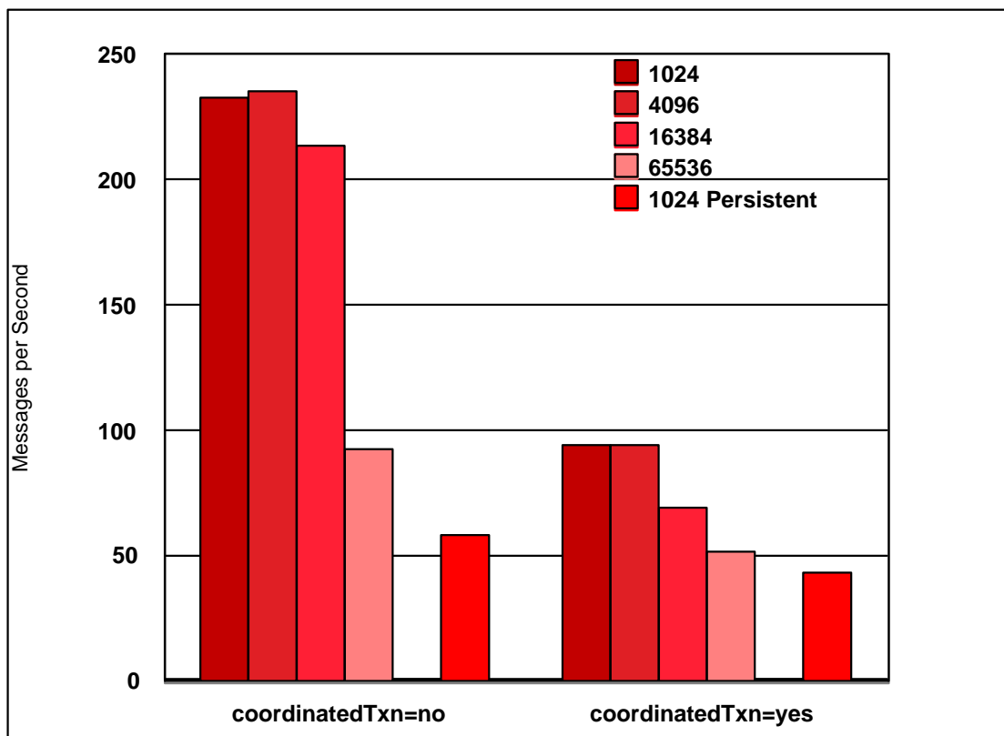
Figure 13: Database Update with XA and coordinatedTransaction=yes .
