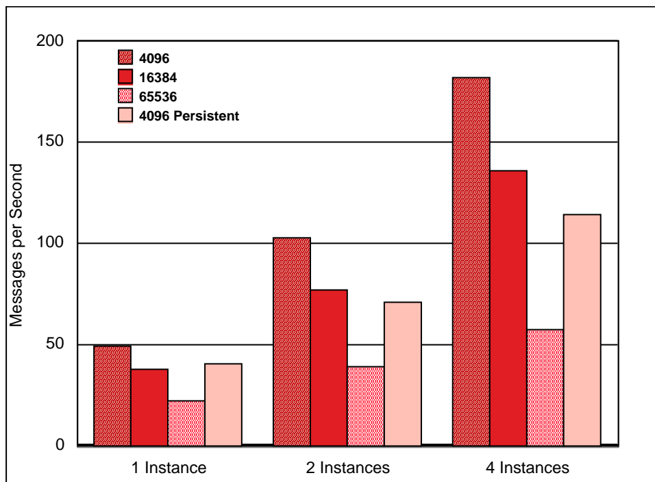
Figure 10: Additional Instances Throughput Results
