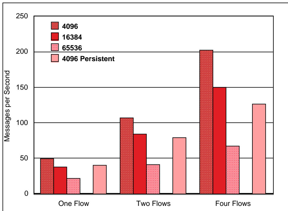
Figure 11: Multiple Copies Throughput Results
