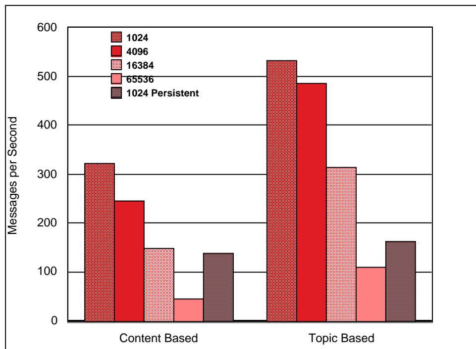
Figure 15: Content vs Topic Based PubSub
