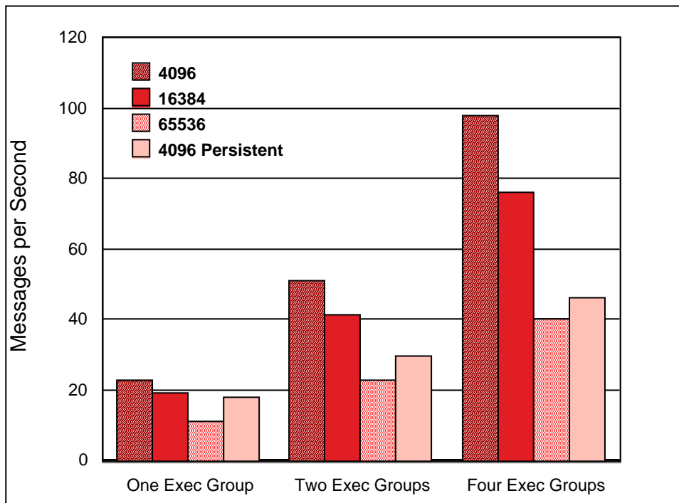
Figure 10: Additional Execution Group Throughput Results
