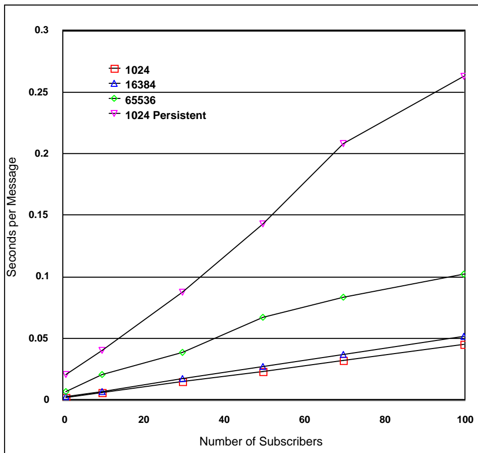
Figure 14: Varying Number of Subscribers
