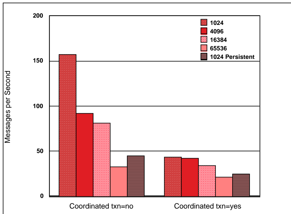
Figure 12: Database Update with XA and coordinatedTransaction=yes.
