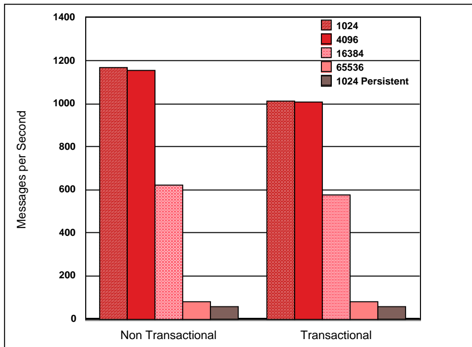
Figure 11: Making a Message Flow Transactional Throughput Results
