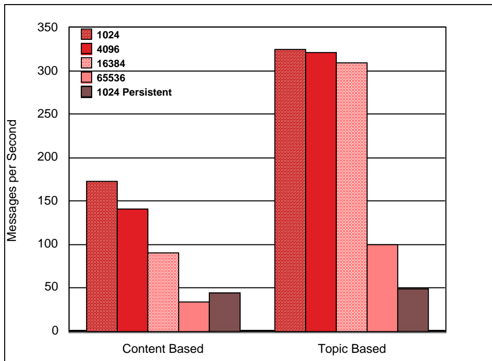
Figure 14: Content vs Topic Based PubSub
