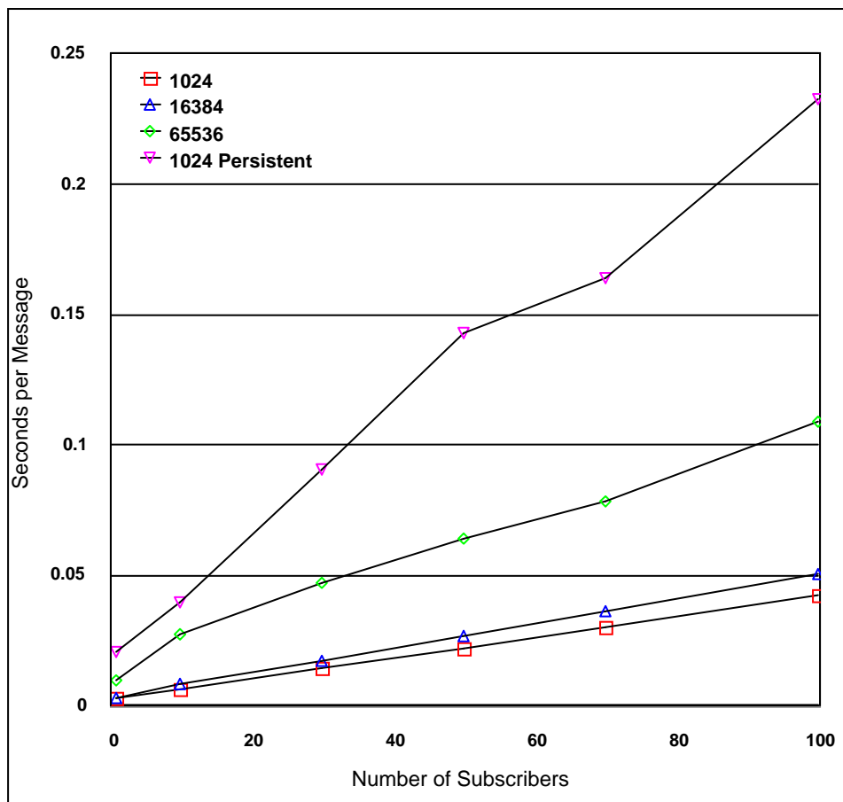
Figure 13: Varying Number of Subscribers
