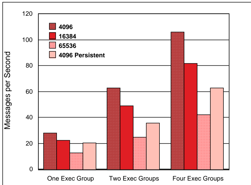
Figure 10: Additional Execution Group Throughput Results
