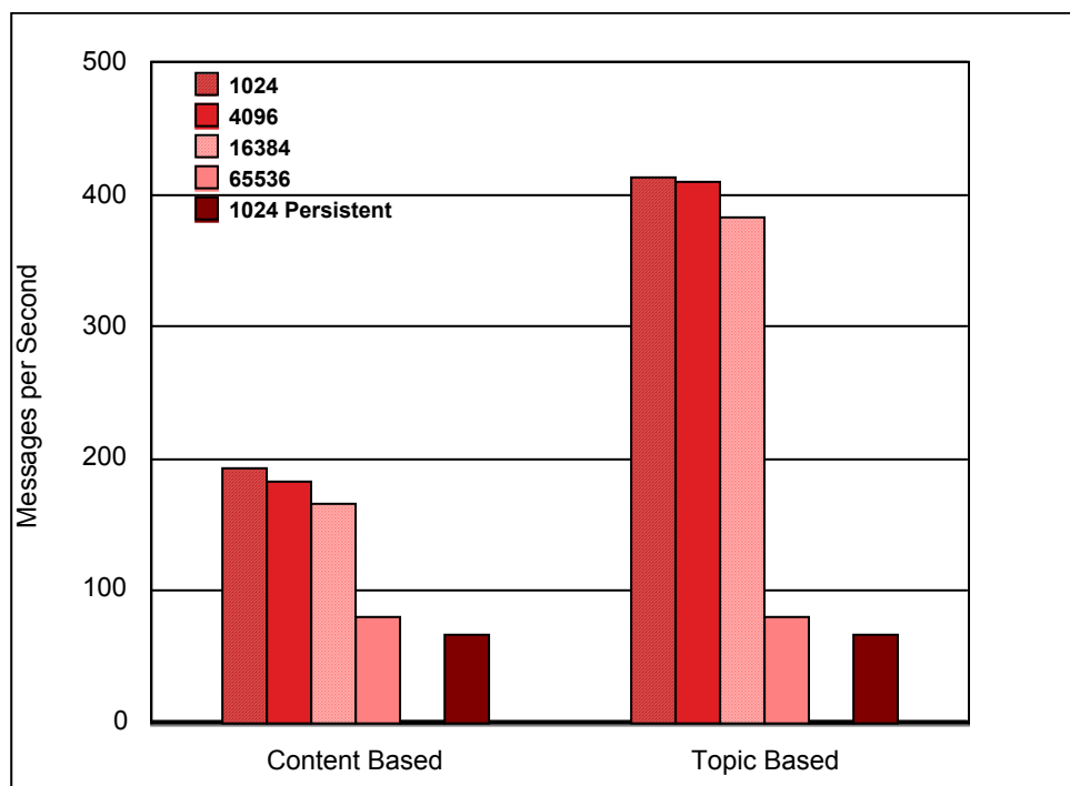
Figure 18 Content vs Topic Based PubSub
