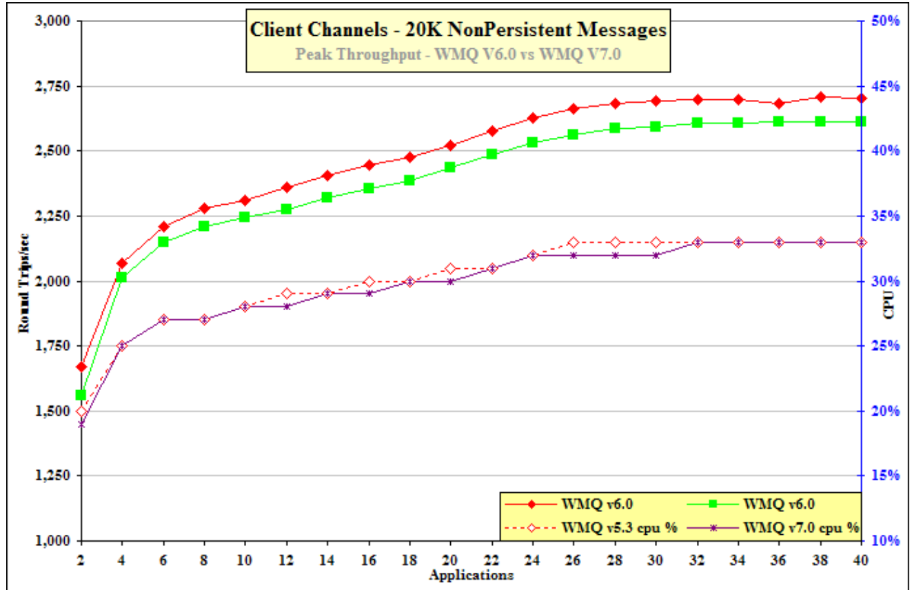
Figure 22 – 20K nonpersistent messages, client channels
