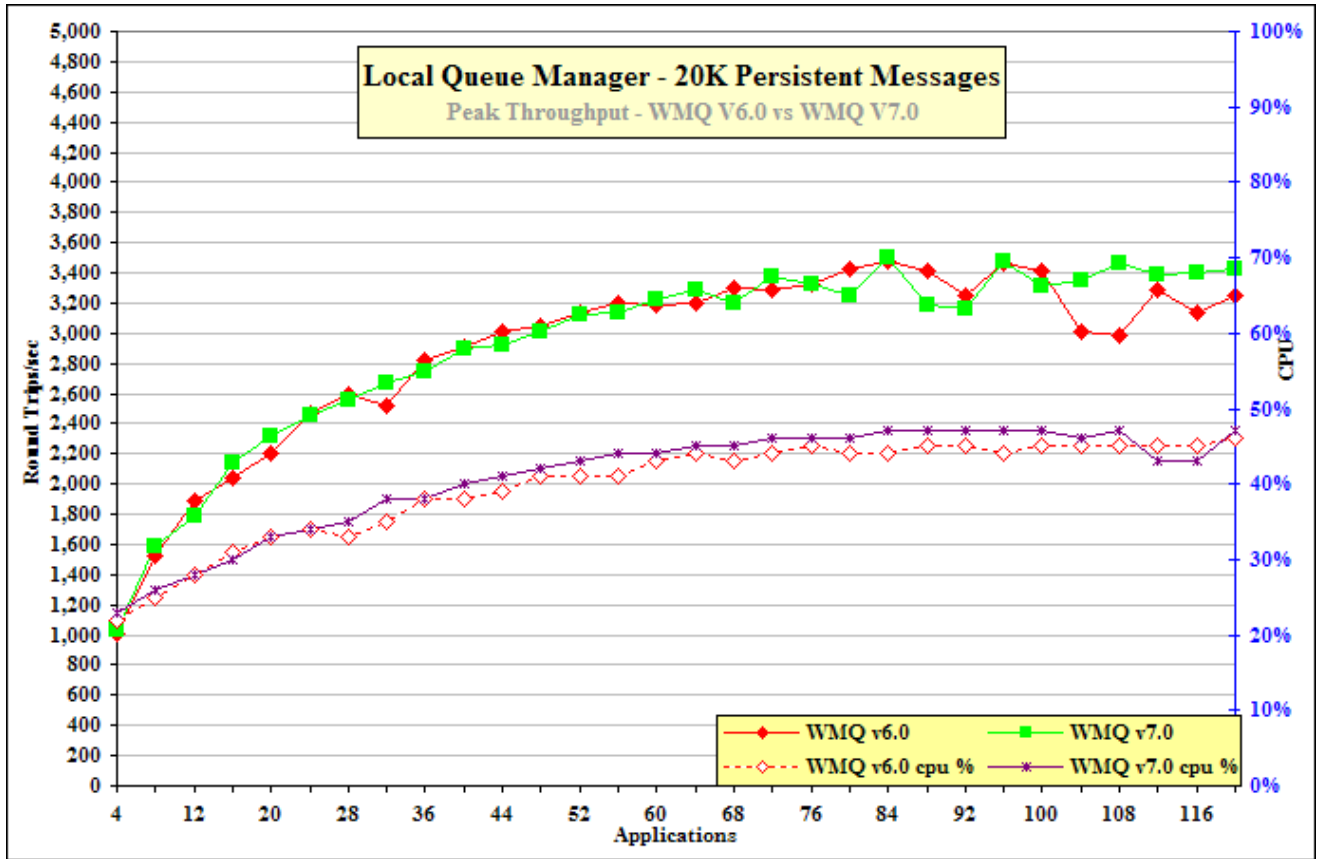
Figure 21 – 20K persistent messages, local queue manager
