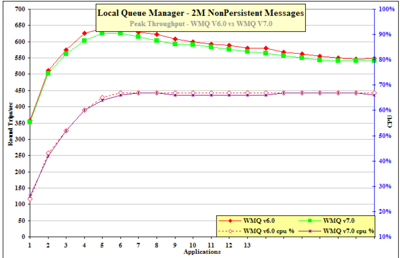
Figure 32 – 2M nonpersistent messages, local queue manager
