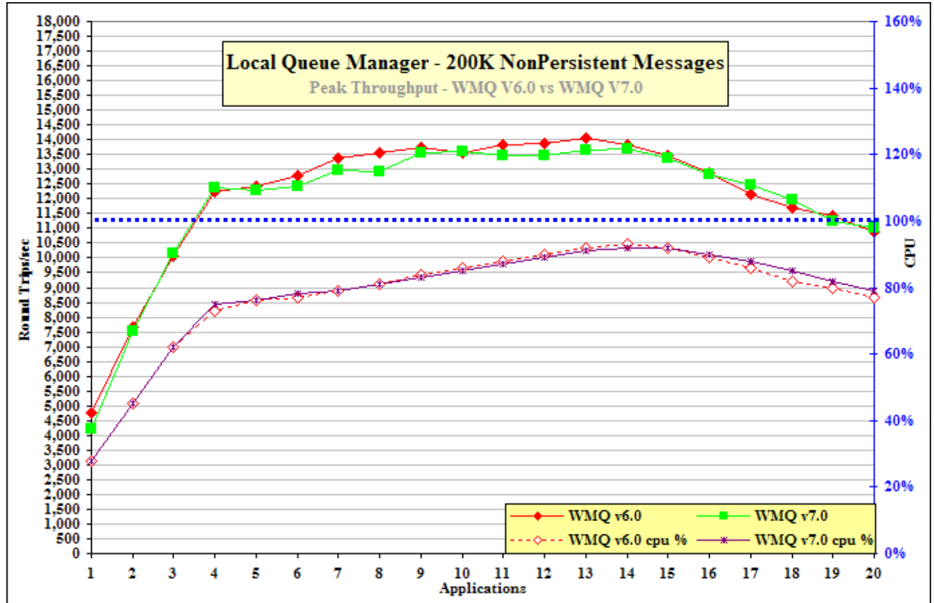
Figure 26 – 200K nonpersistent messages, local queue manager
