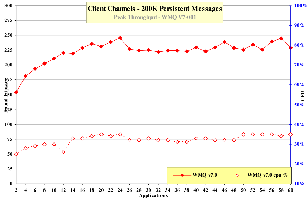
Figure 29 – 200K persistent messages, client channels
