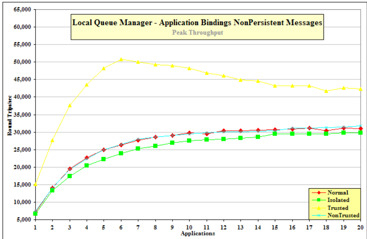
Figure 38 – Application binding, nonpersistent messages, local queue manager
