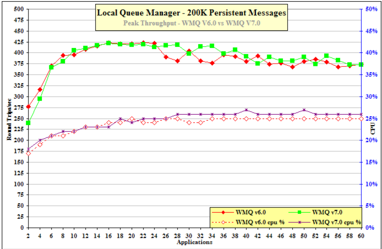
Figure 27 – 200K persistent messages, local queue manager
