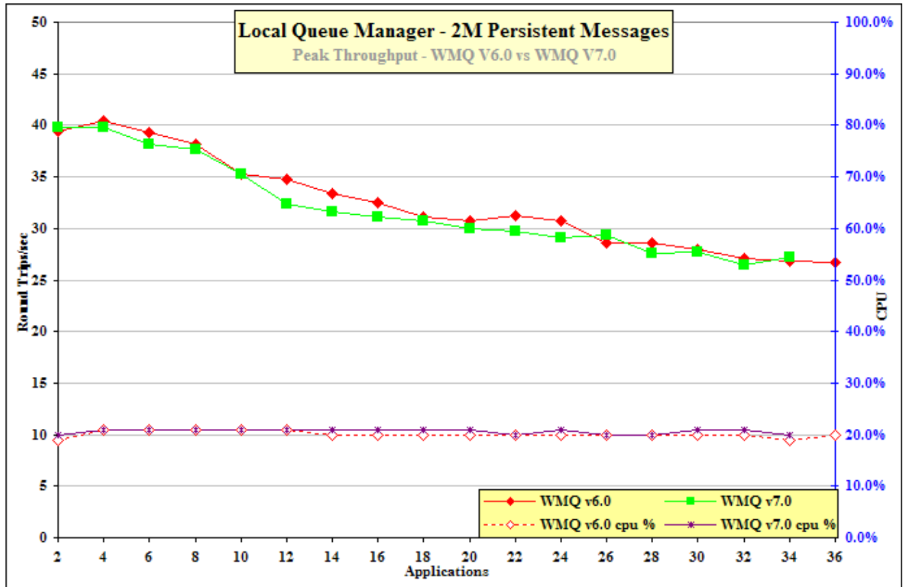
Figure 33 – 2M persistent messages, local queue manager
