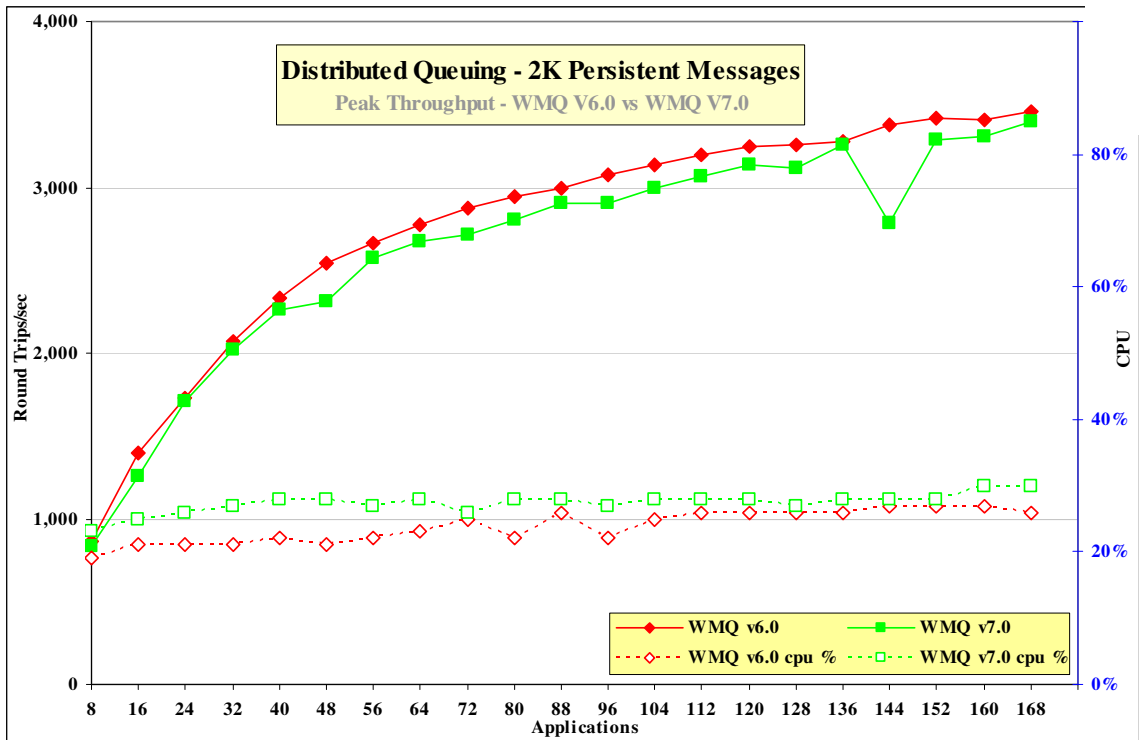
Figure 11 – Performance headline, persistent messages, server channels
