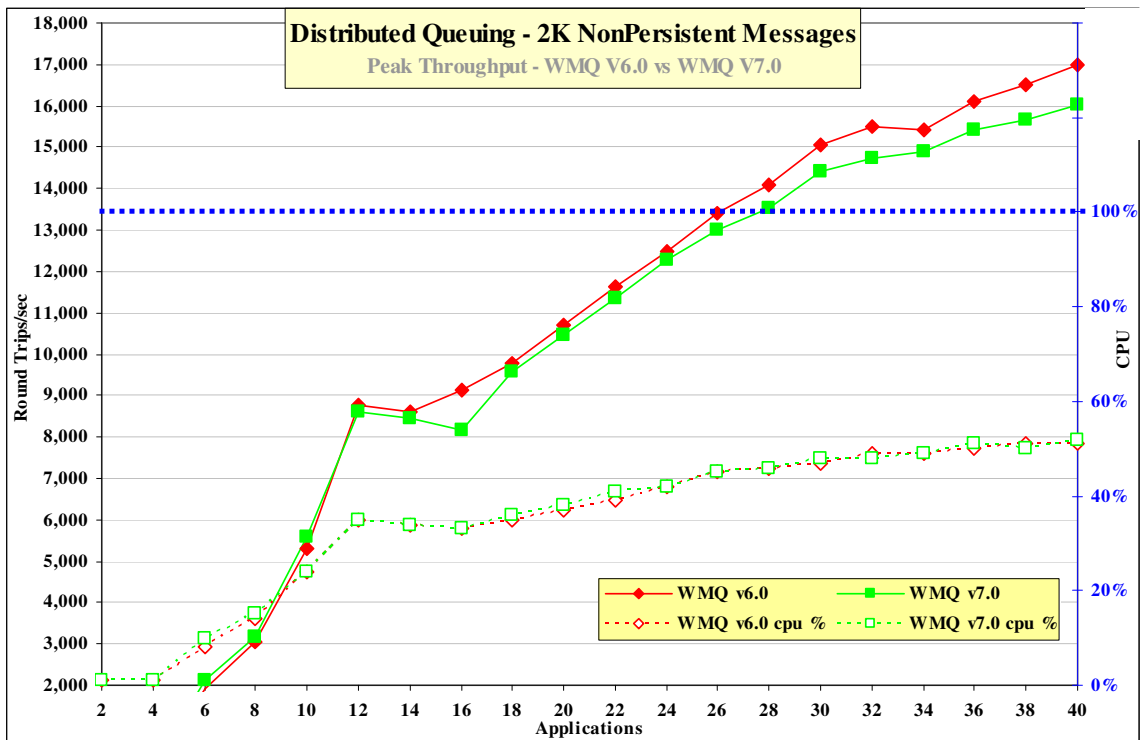
Figure 10 – Performance headline, nonpersistent messages, server channels
