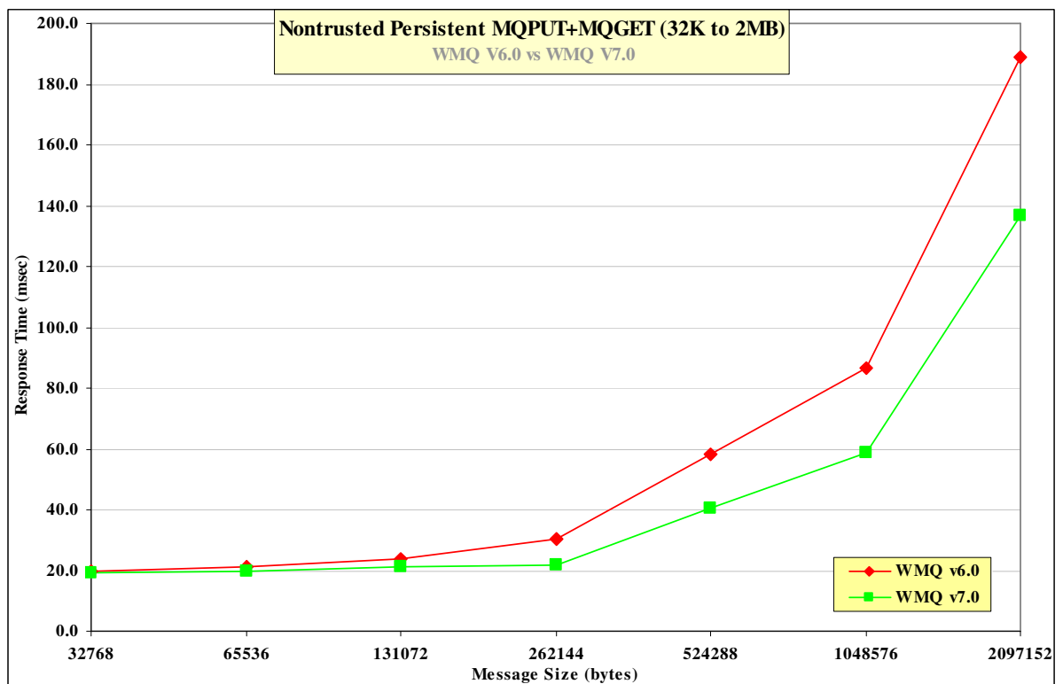
Figure 22 –The effect of persistent message size on MQI response time (32K – 2Mb)
