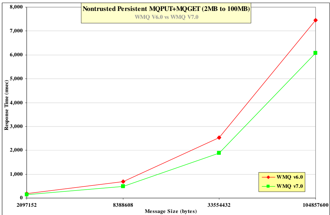
Figure 24 –The effect of persistent message size on MQI response time (2Mb – 100Mb)
