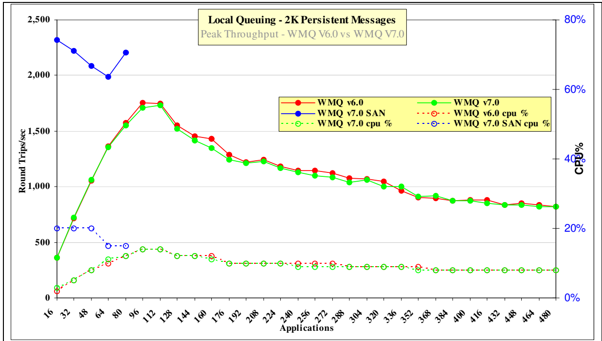
Figure 4 – Performance headline, persistent messages, local queue manager
