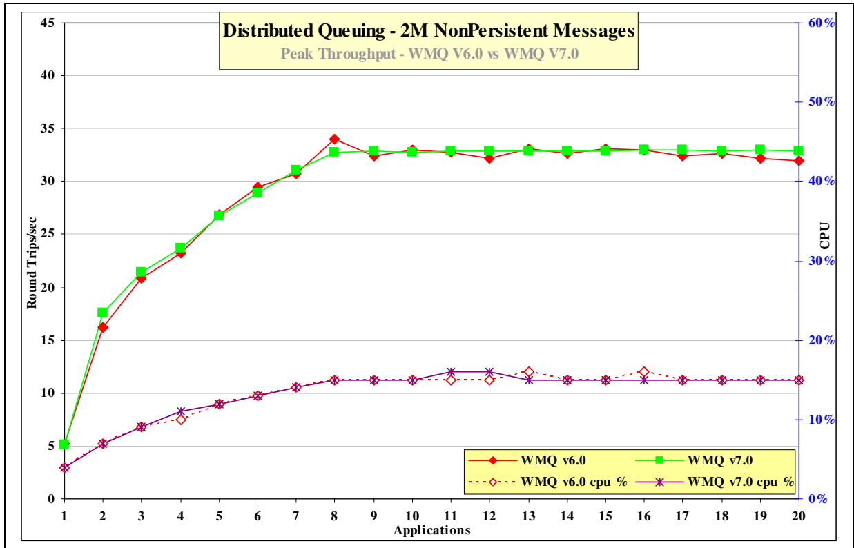
Figure 41 – 2M nonpersistent messages, distributed queuing
