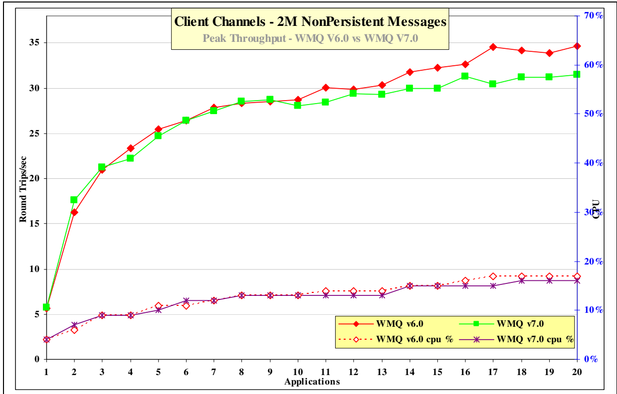
Figure 39 – 2M nonpersistent messages, client channels
