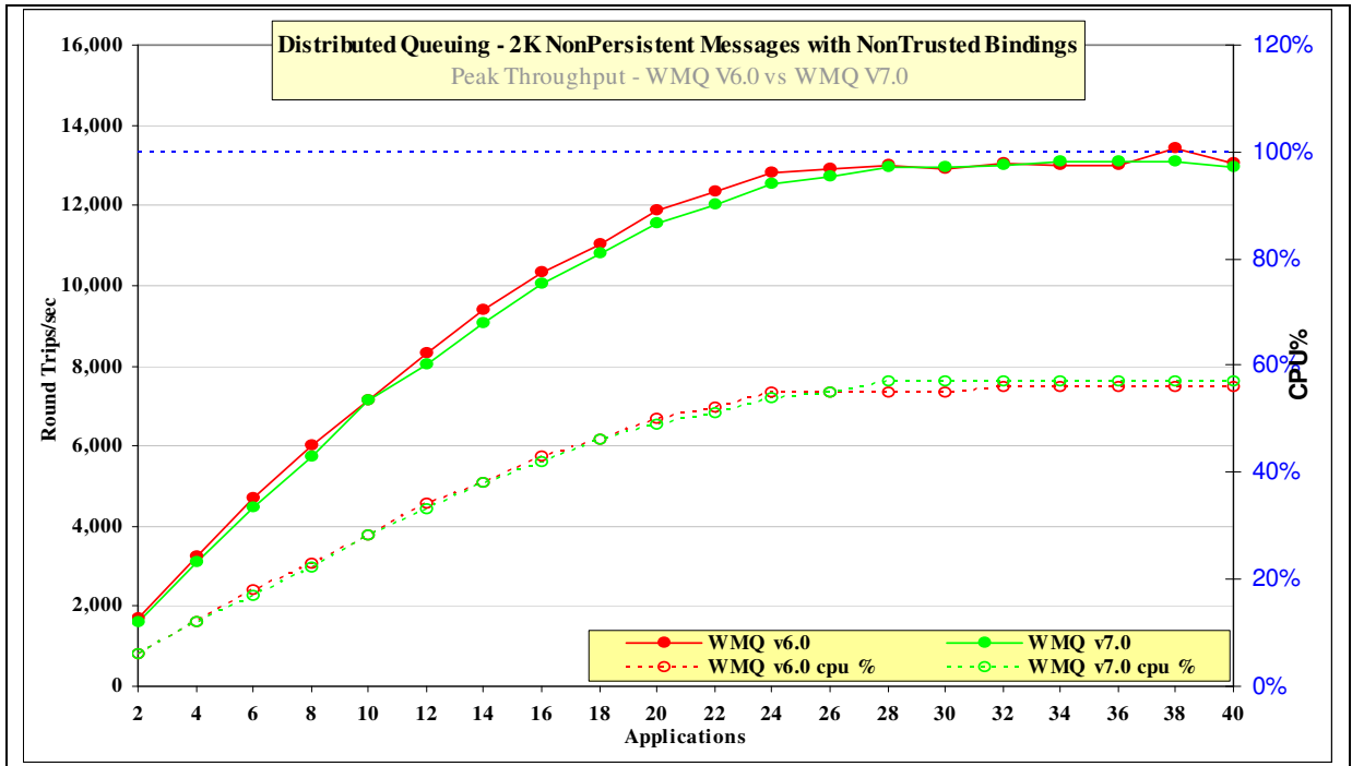
Figure 14 – Performance headline, nonpersistent messages, non-trusted, server channels
