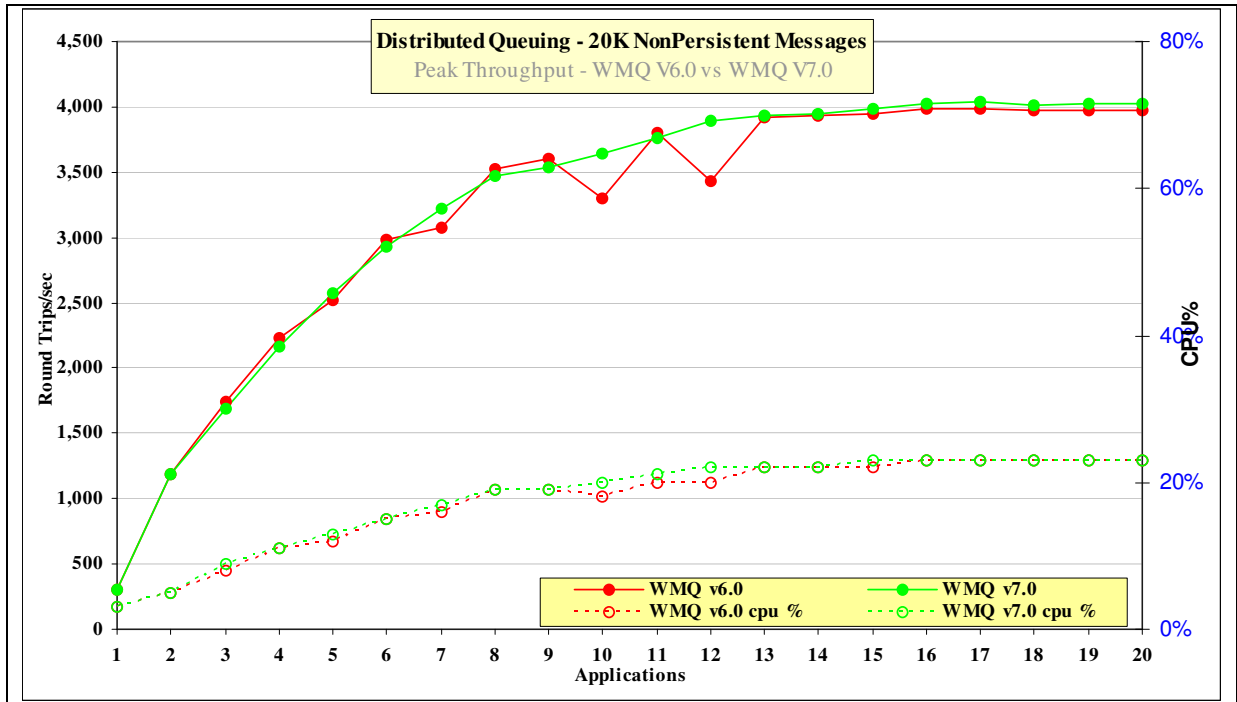
Figure 29 – 20K nonpersistent messages, distributed queuing
