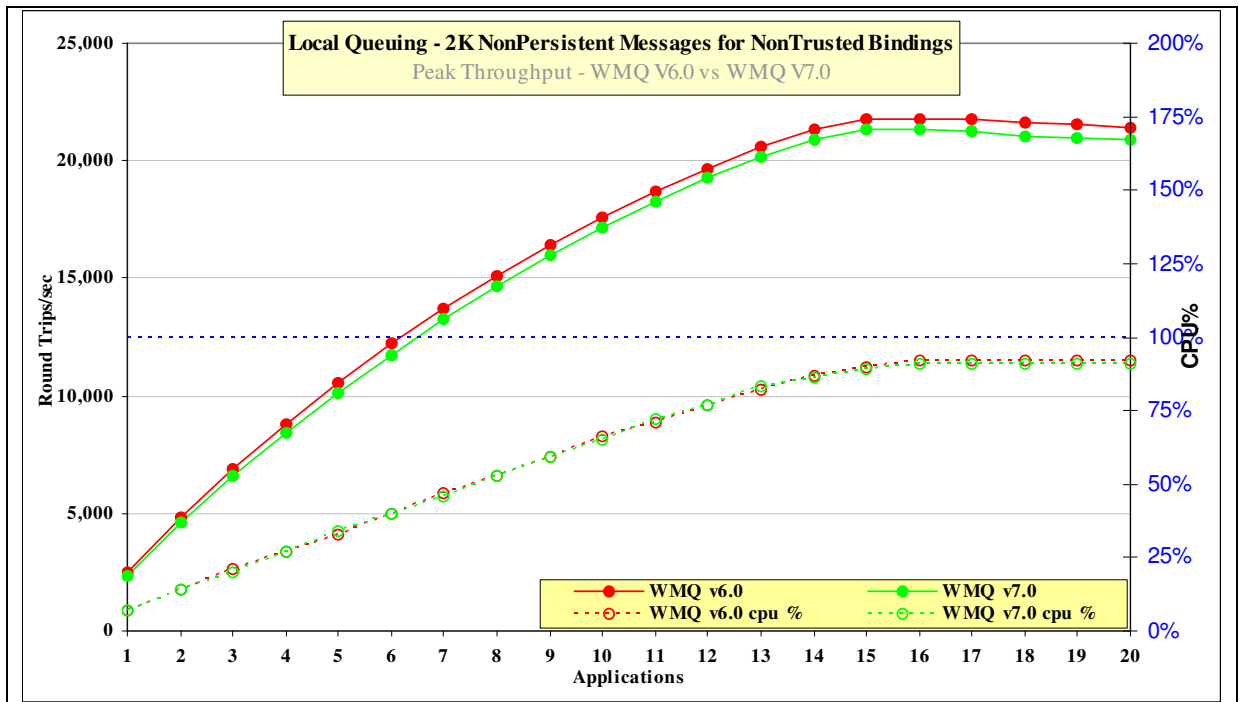
Figure 3 – Performance headline, non-persistent messages, non-trusted bindings, local queue manager
