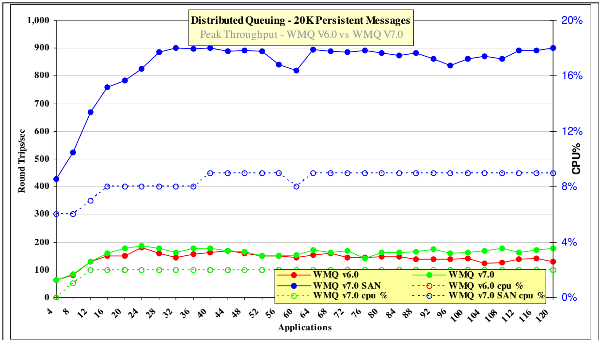
Figure 30 – 20K persistent messages, distributed queuing
