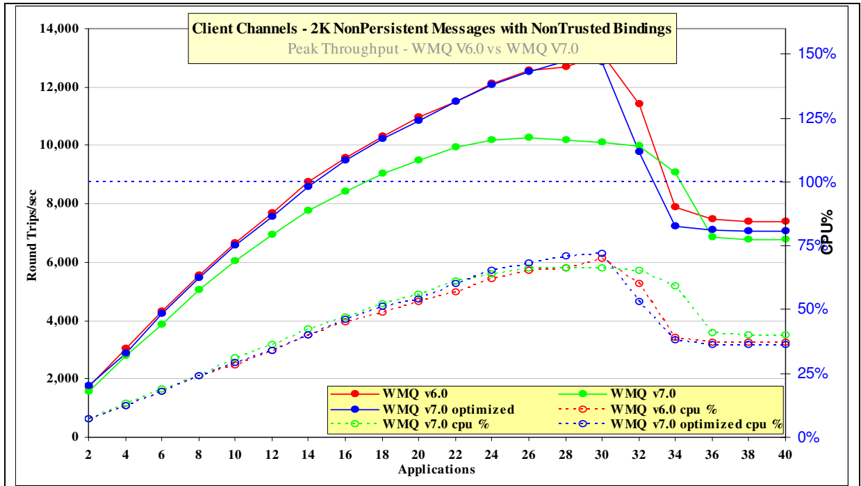
Figure 7 – Performance headline, nonpersistent messages, non-trusted client channels
