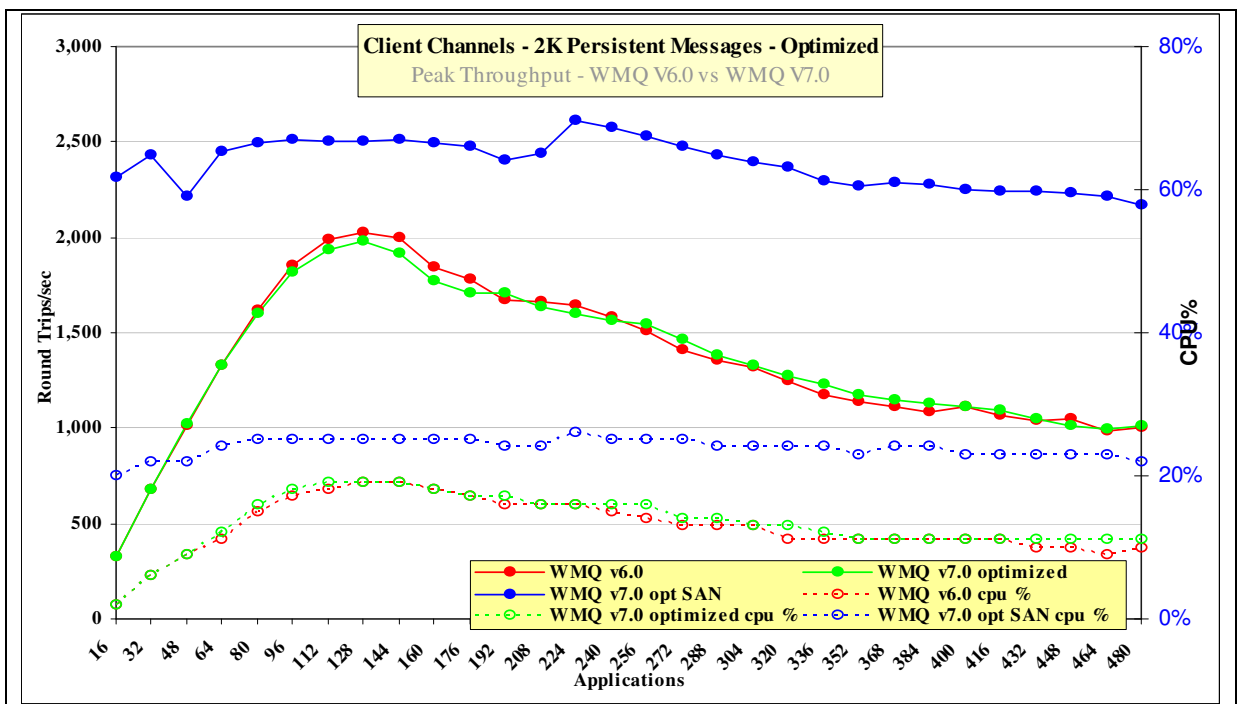
Figure 9 – Performance headline, persistent messages, client channels, optimized
