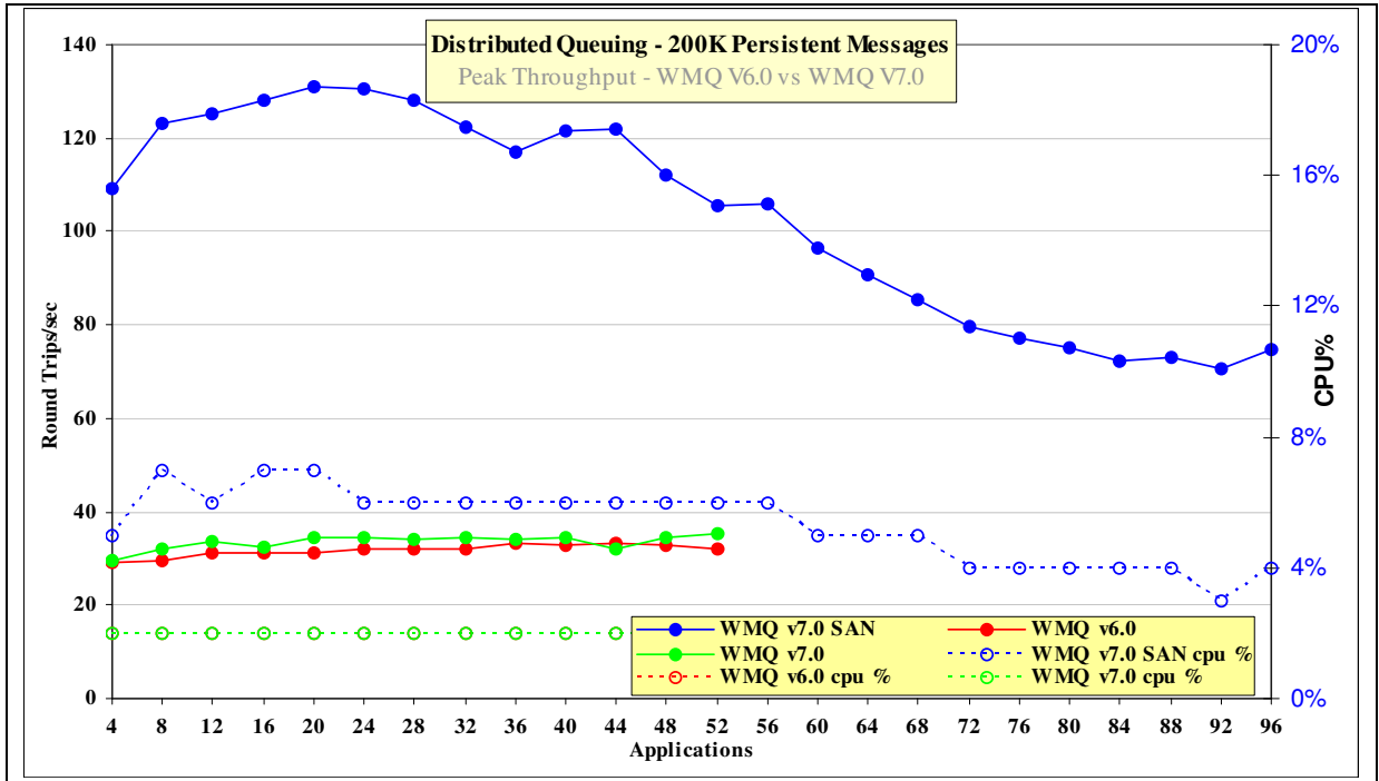
Figure 36 – 200K persistent messages, distributed queuing
