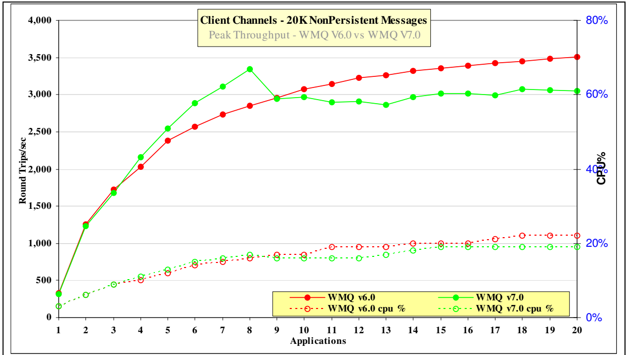
Figure 27 – 20K nonpersistent messages, client channels
