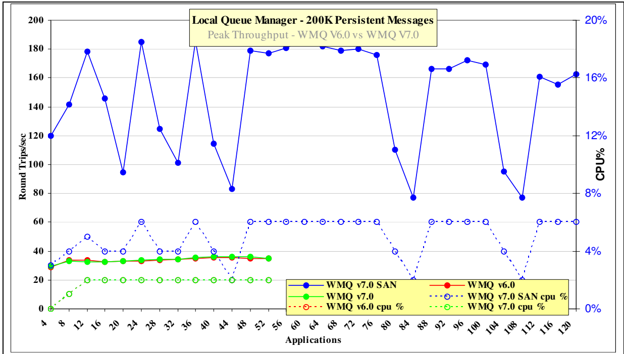
Figure 32 – 200K persistent messages, local queue manager
