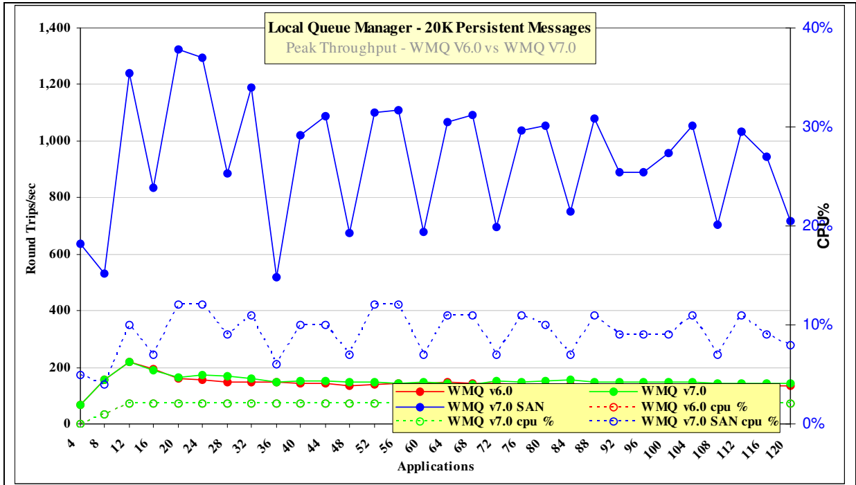
Figure 26 – 20K persistent messages, local queue manager
