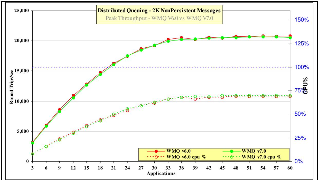
Figure 13 – Performance headline, nonpersistent messages, server channels
