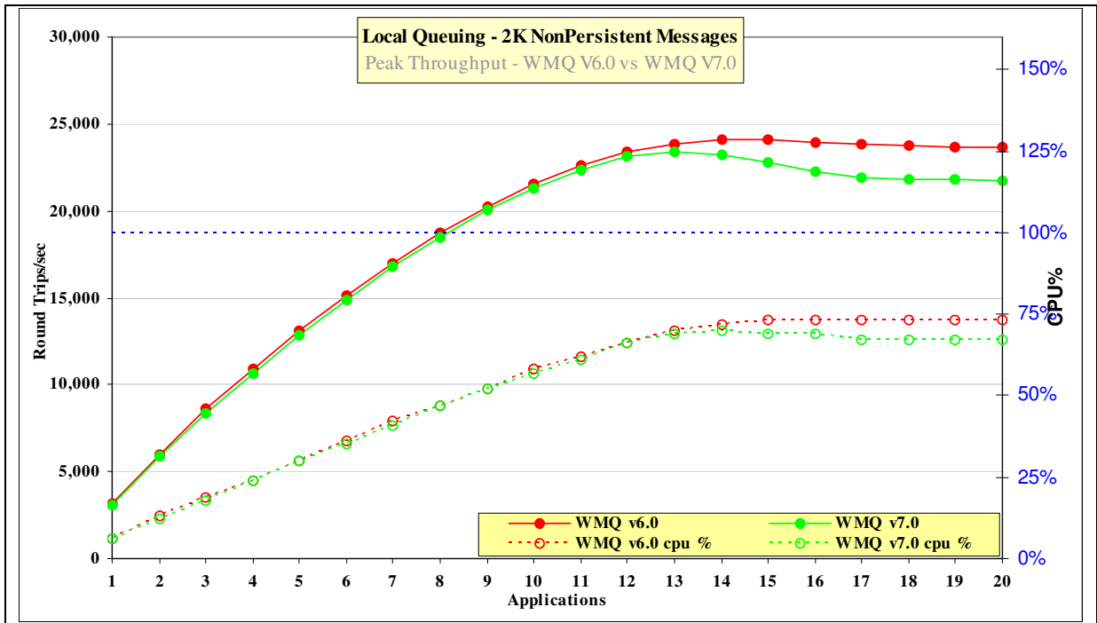
Figure 2 – Performance headline, nonpersistent messages, local queue manager
