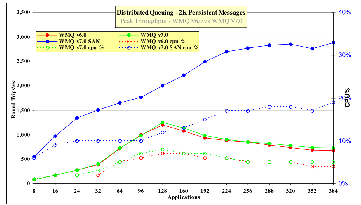
Figure 15 – Performance headline, persistent messages, server channels
