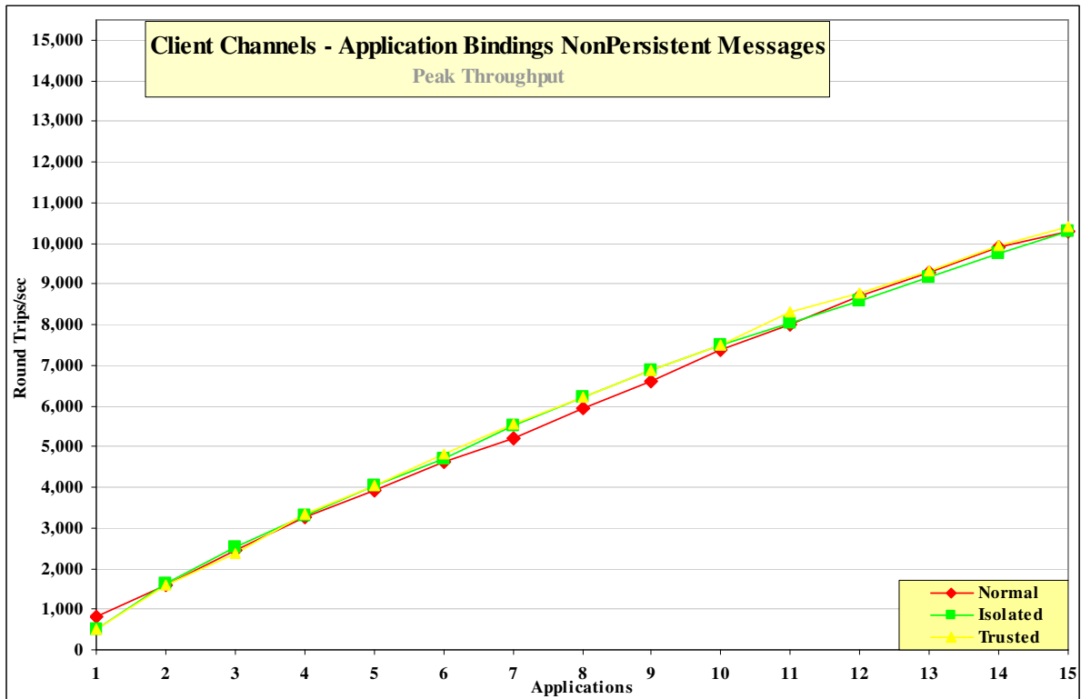
Figure 45 – Application binding, nonpersistent messages, client channels
