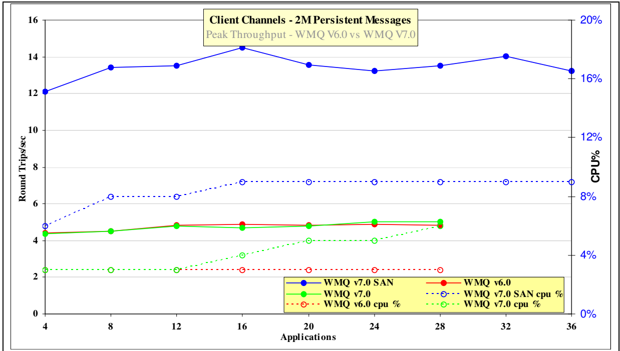
Figure 40 – 2M persistent messages, client channels
