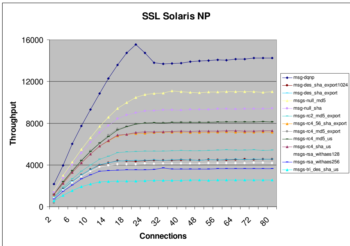
Figure 18 – effect of SSL Cipher Specifications on Throughput
