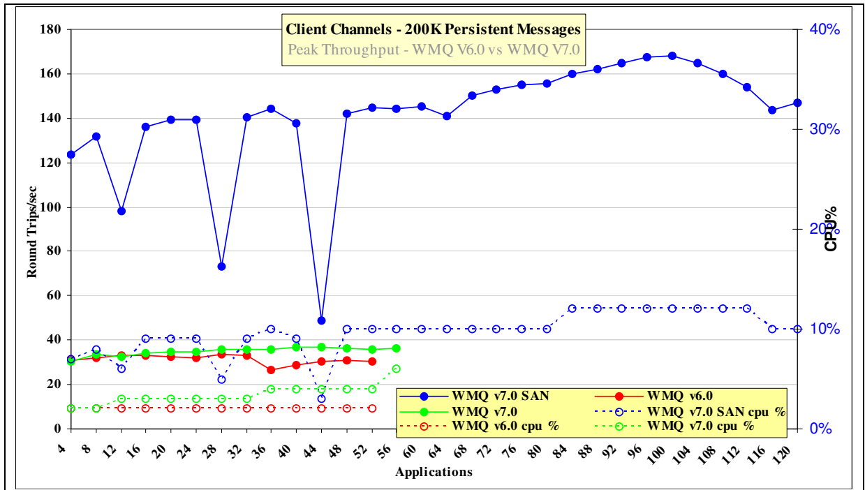
Figure 34 – 200K persistent messages, client channels
