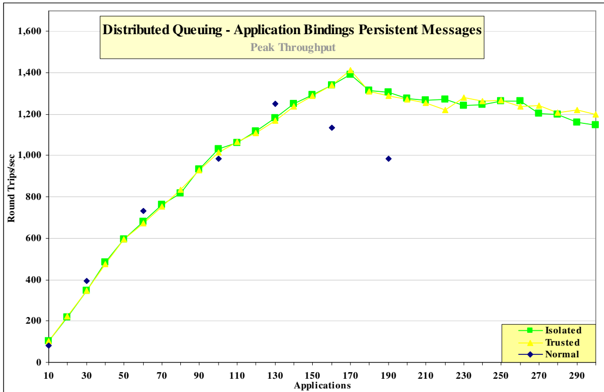
Figure 48 – Application binding, persistent messages, distributed queuing
