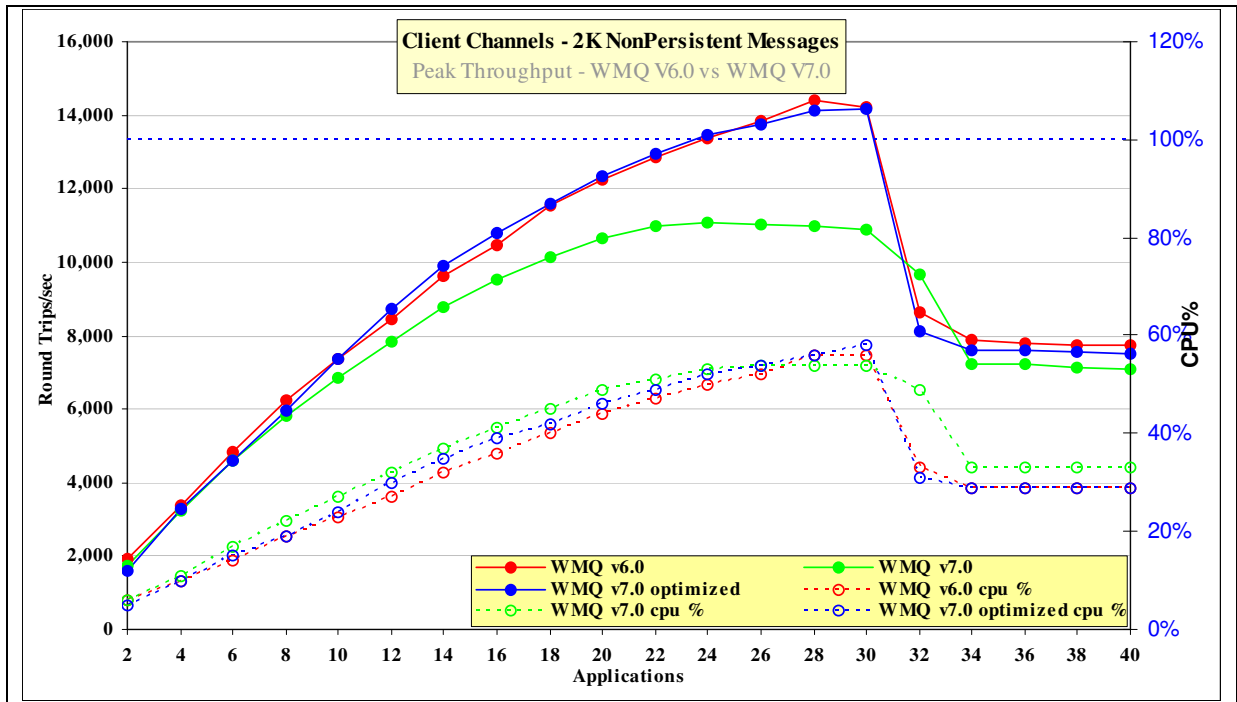
Figure 6 – Performance headline, nonpersistent messages, client channels
