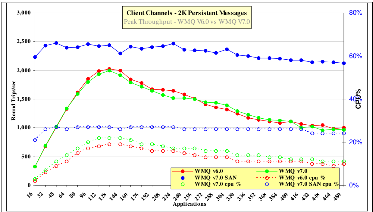
Figure 8 – Performance headline, persistent messages, client channels
