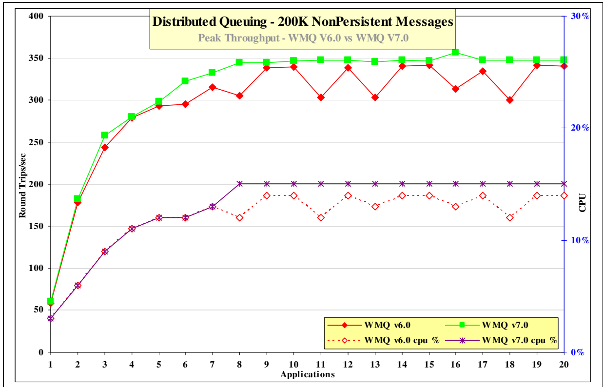
Figure 35 – 200K nonpersistent messages, distributed queuing
