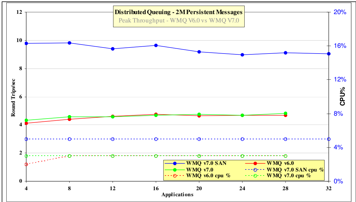
Figure 42 – 2M persistent messages, distributed queuing
