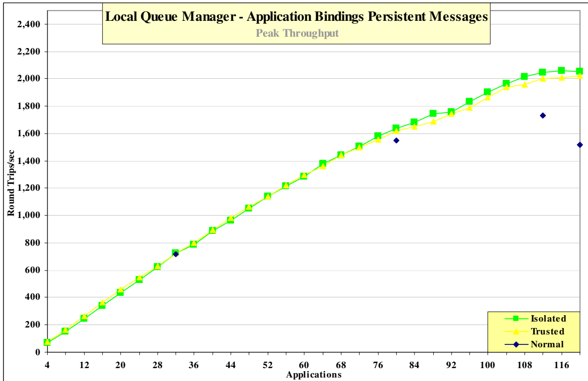
Figure 44 – Application binding, persistent messages, local queue manager
