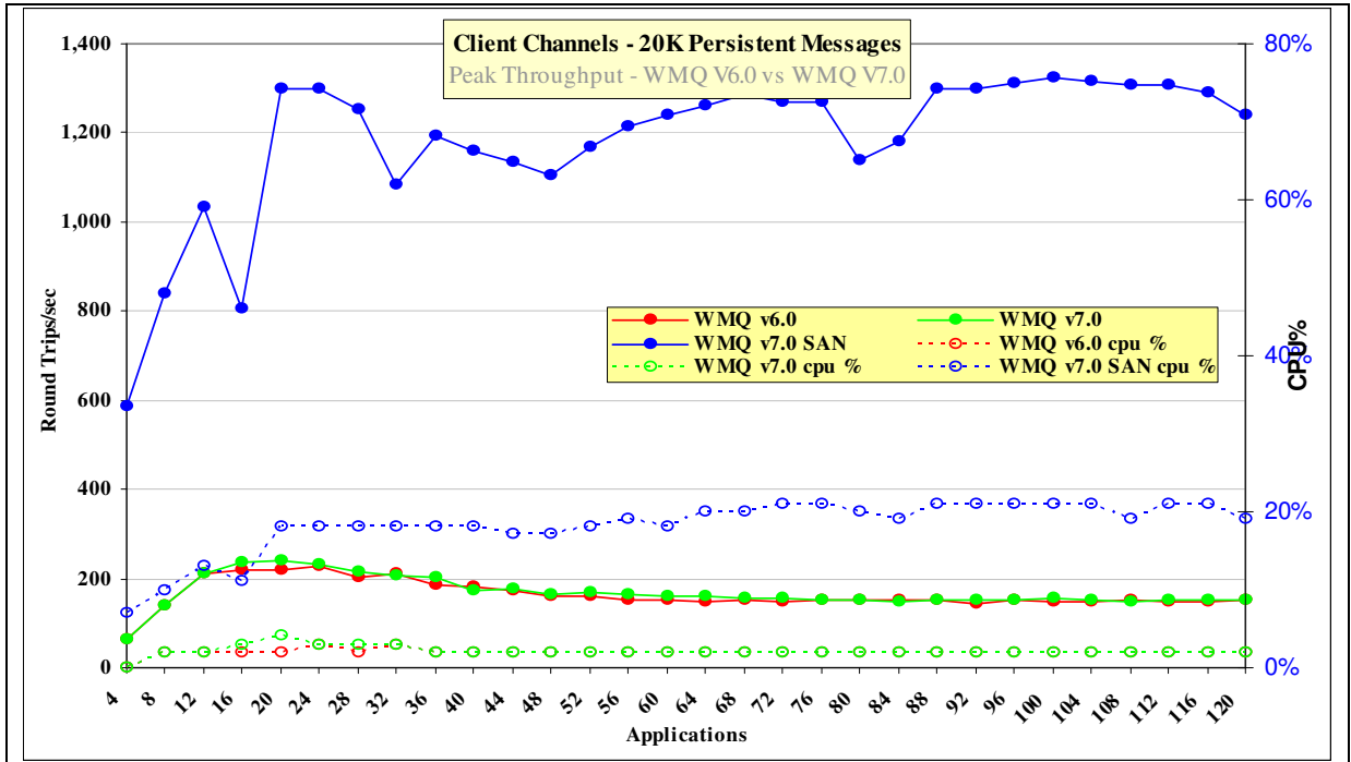
Figure 28 – 20K persistent messages, client channels
