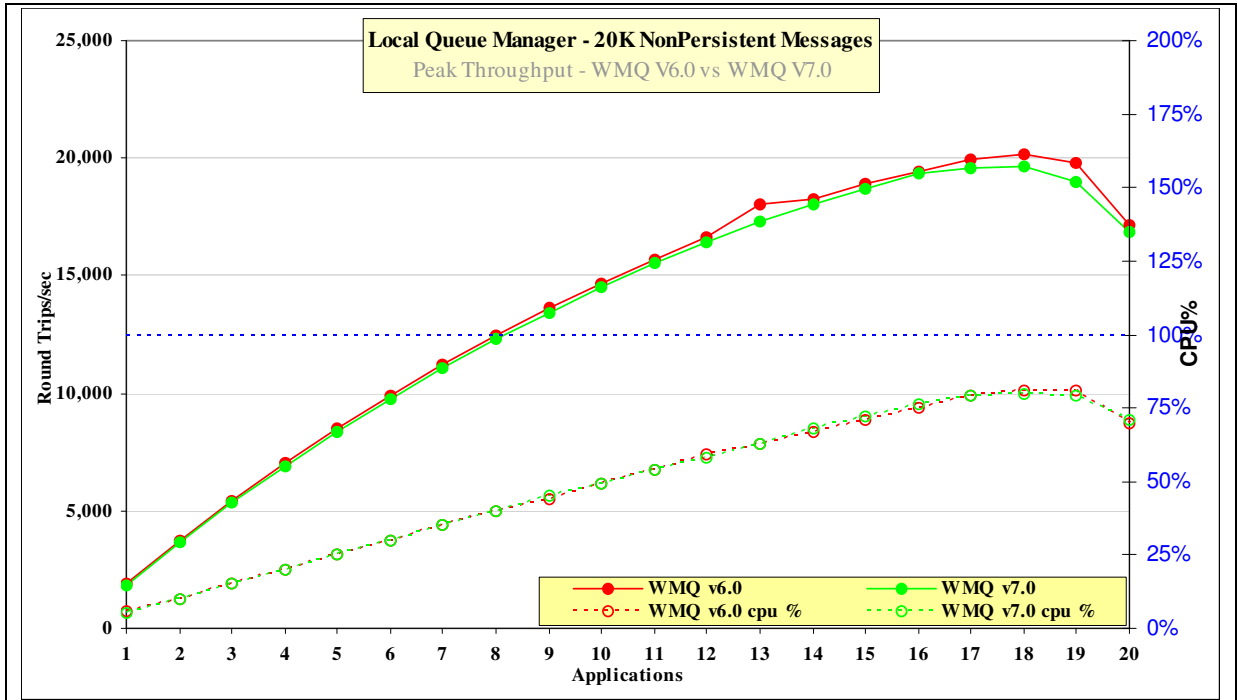
Figure 25 – 20K nonpersistent messages, local queue manager
