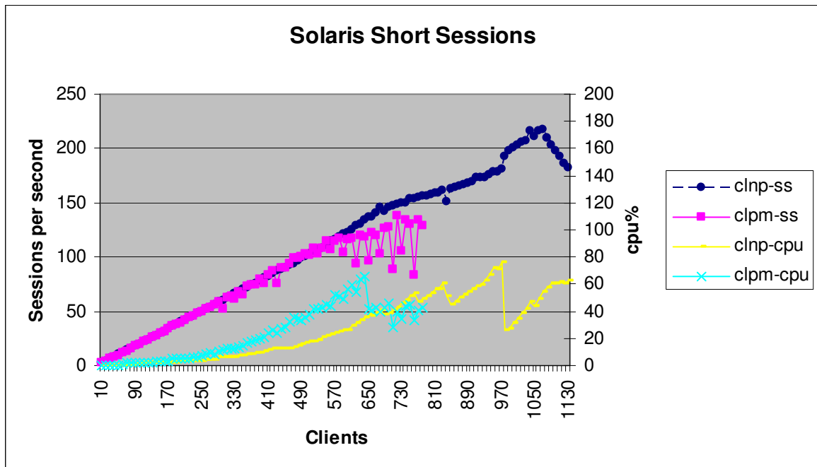
Figure 49 – Short sessions, client channels
