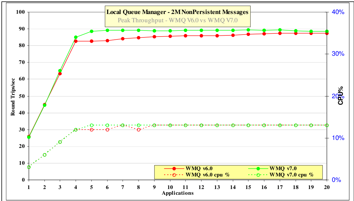
Figure 37 – 2M nonpersistent messages, local queue manager
