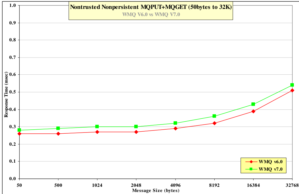
Figure 19 –The effect of nonpersistent message size on MQI response time (50byte - 32K)
