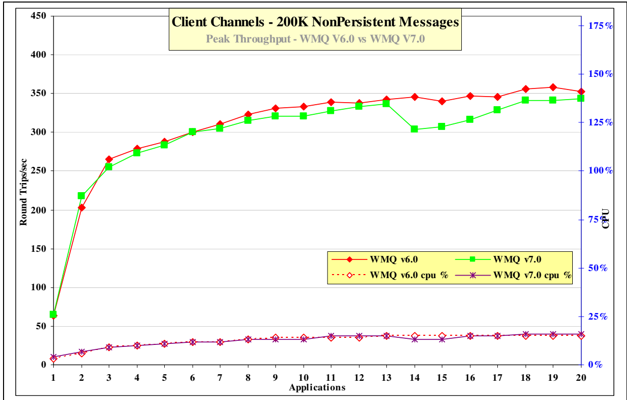
Figure 33 – 200K nonpersistent messages, client channels
