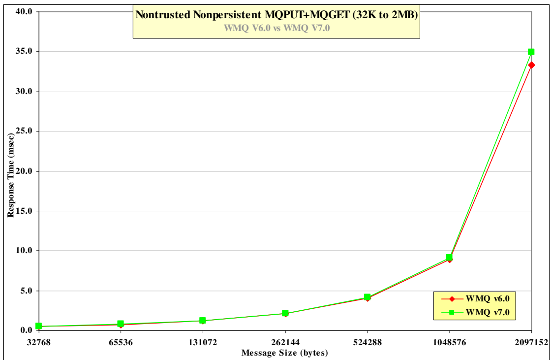
Figure 21 –The effect of nonpersistent message size on MQI response time (32K – 2Mb)
