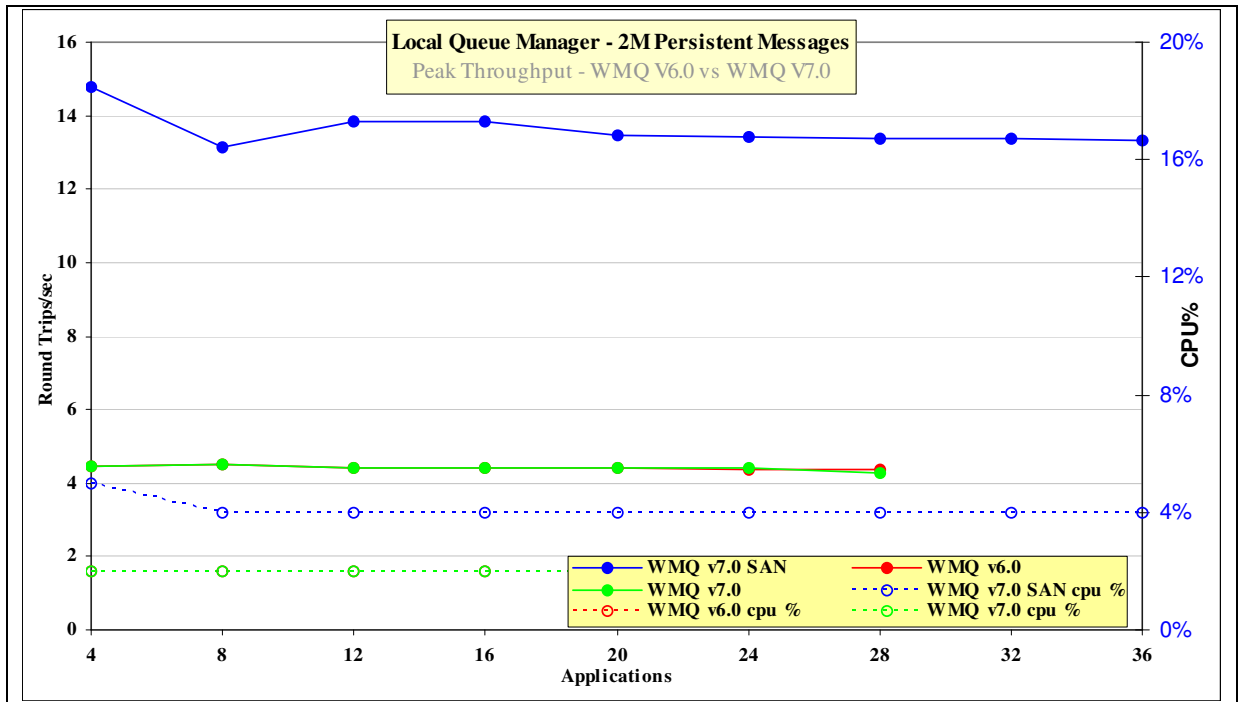
Figure 38 – 2M persistent messages, local queue manager
