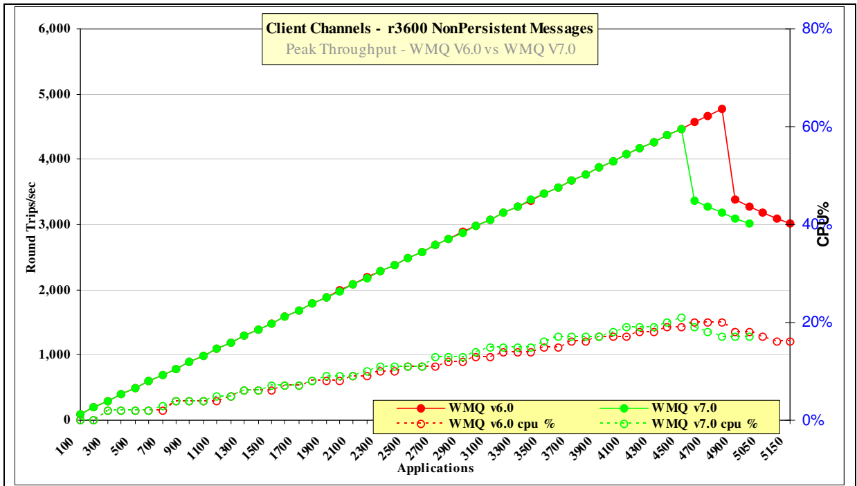
Figure 10 – 1 round trip per driving application per second, client channels, nonpersistent messages
