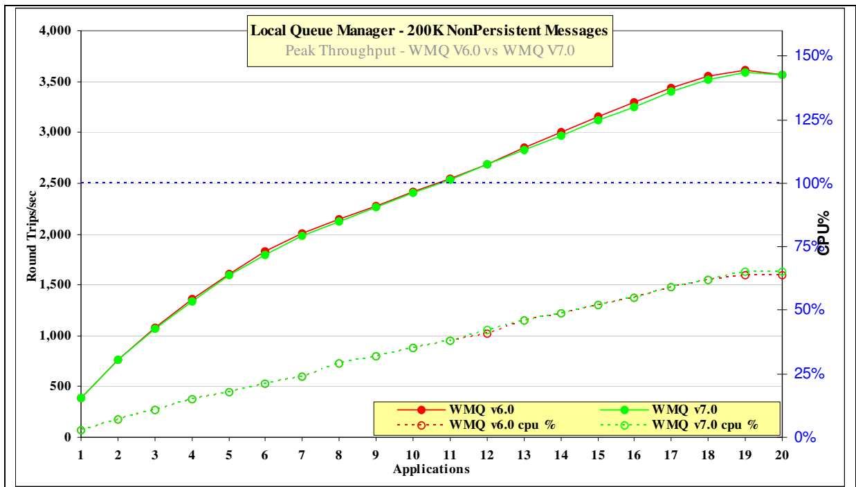
Figure 31 – 200K nonpersistent messages, local queue manager
