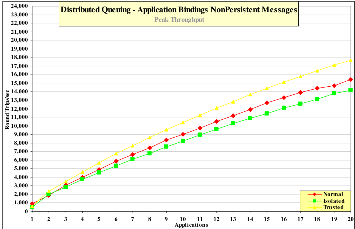
Figure 47 – Application binding, nonpersistent messages, distributed queuing
