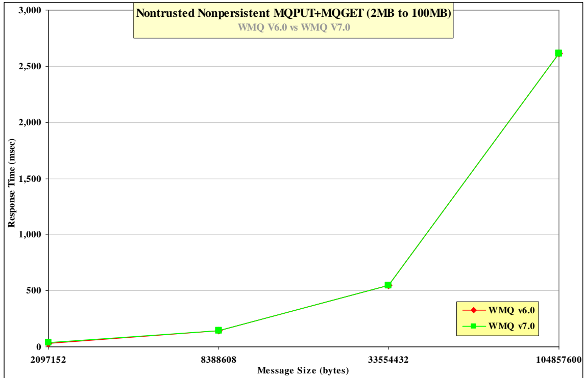
Figure 23 –The effect of nonpersistent message size on MQI response time (2Mb – 100Mb)
