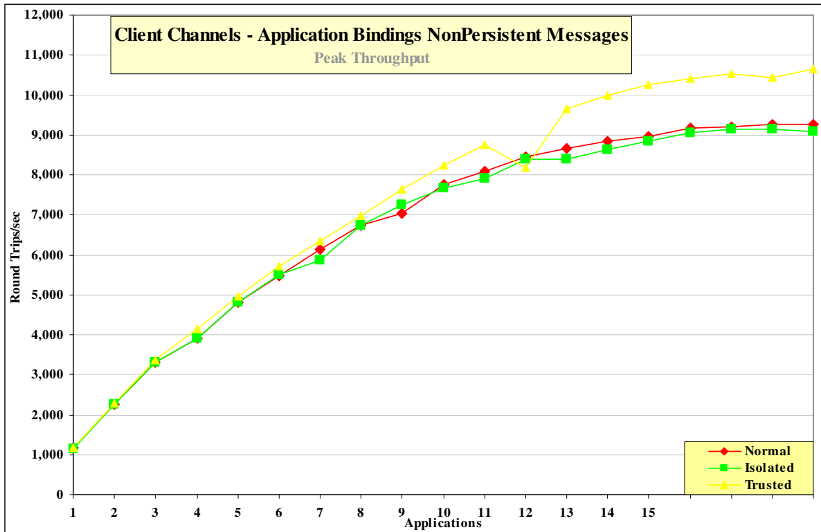
Figure 40 – Application binding, nonpersistent messages, client channels
