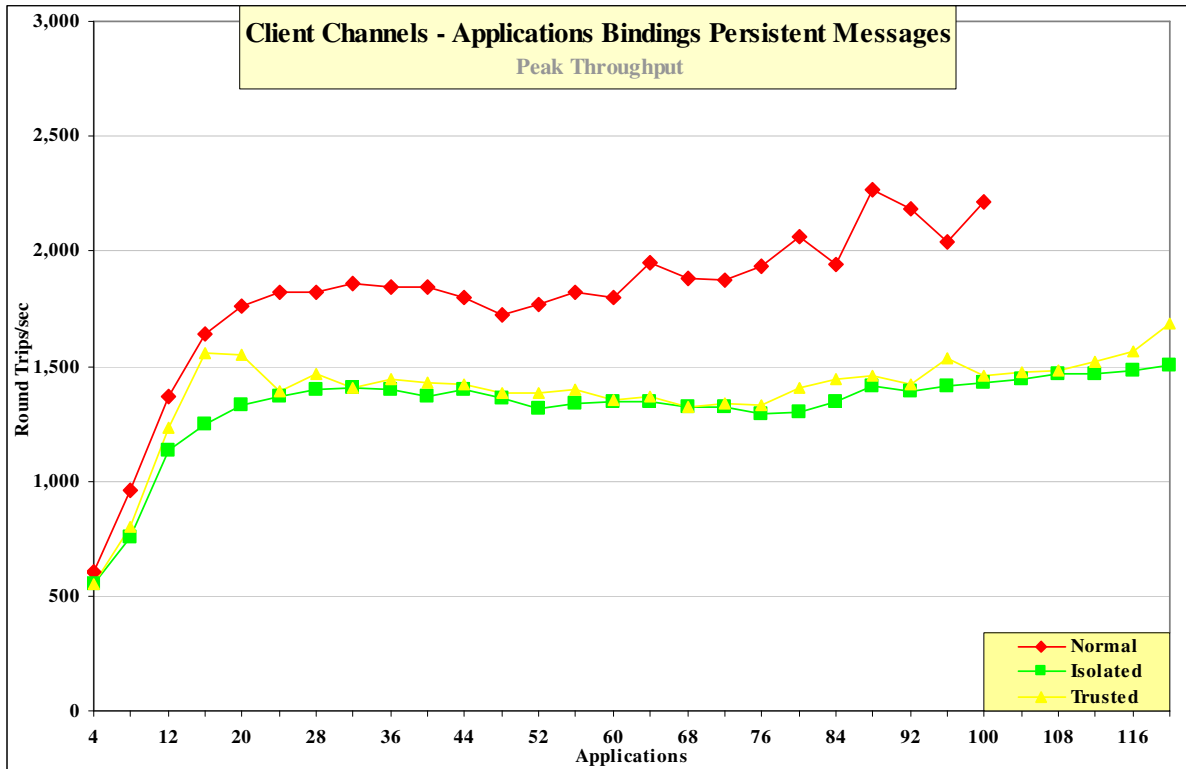
Figure 41 – Application binding, persistent messages, client channels
