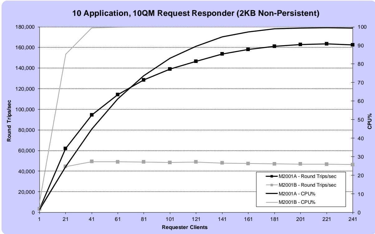
FIGURE 5 - PERFORMANCE RESULTS FOR 2KB, 10QM NON-PERSISTENT MESSAGING
