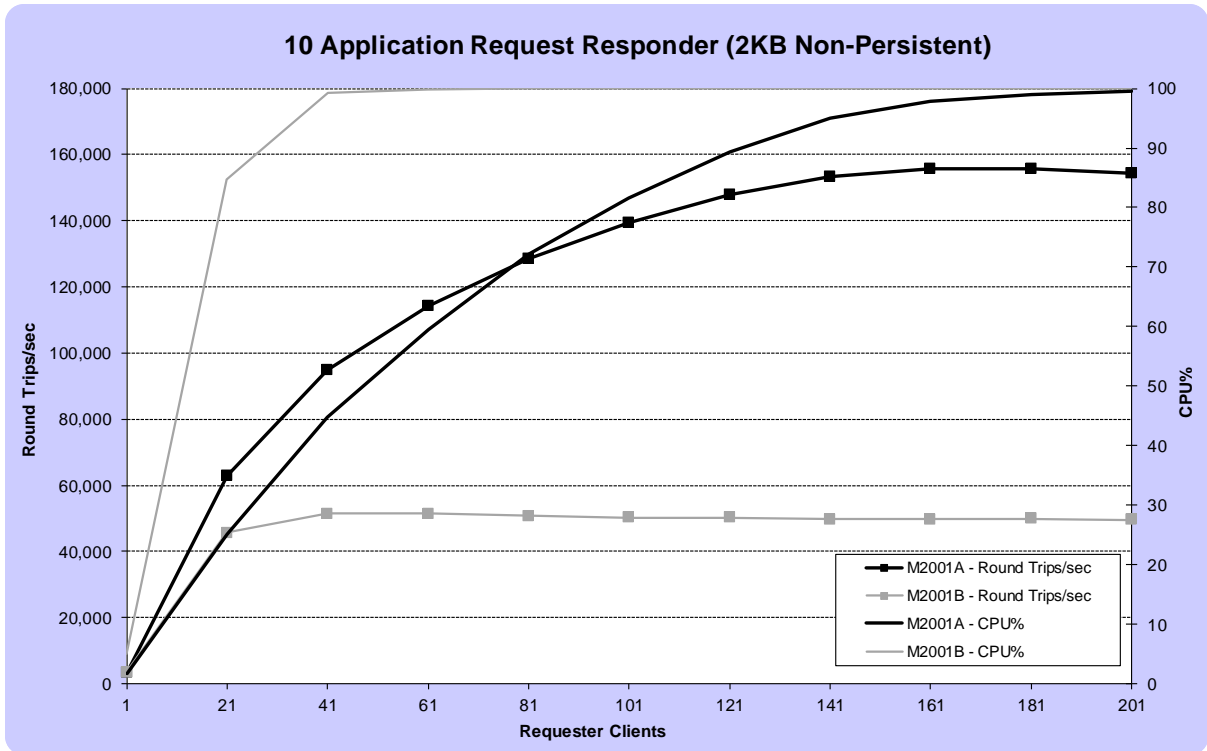
FIGURE 3 – PERFORMANCE RESULTS FOR 2KB NON-PERSISTENT MESSAGING
