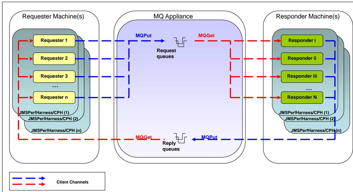
FIGURE 2 - REQUESTER-RESPONDER WITH REMOTE QUEUE MANAGER ON MQ APPLIANCE
