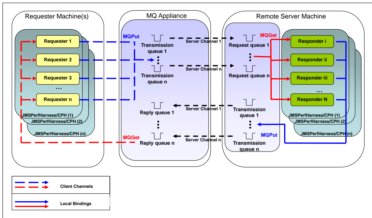
FIGURE 7 - REQUESTER-RESPONDER WITH DISTRIBUTED QUEUEING
