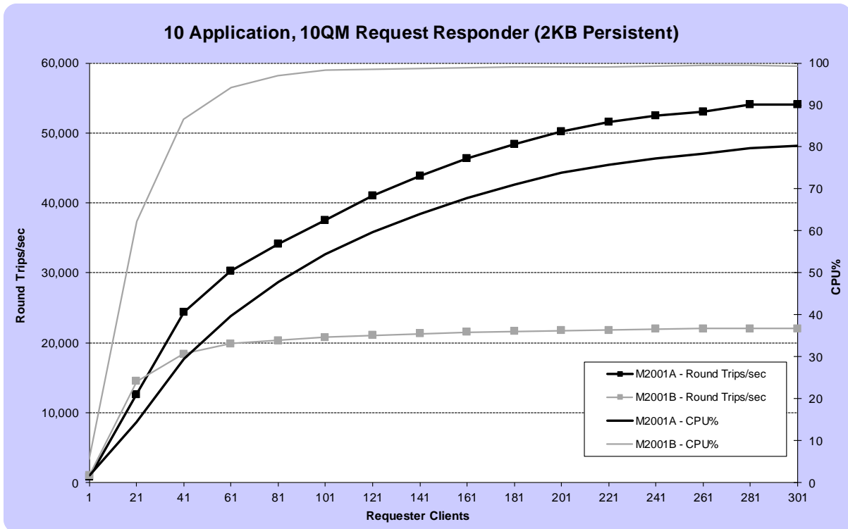
FIGURE 6 - PERFORMANCE RESULTS FOR 2KB, 10QM PERSISTENT MESSAGING
