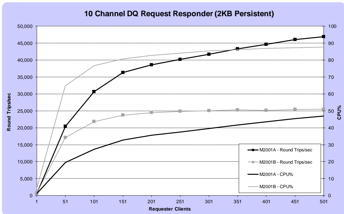
FIGURE 9 - PERFORMANCE RESULTS FOR 2KB, 10 CHANNEL DQ PERSISTENT MESSAGING
