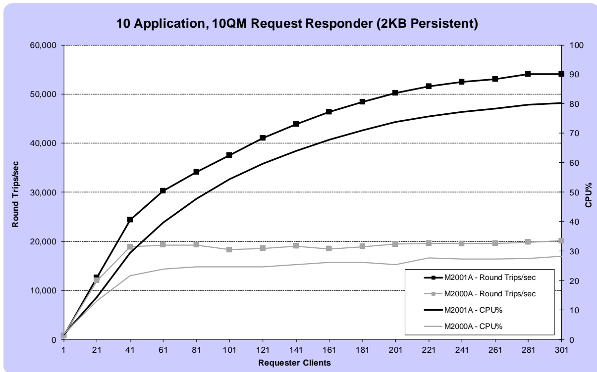
FIGURE 1 - PERFORMANCE RESULTS FOR 2KB, 10QM PERSISTENT MESSAGING, M2001A vs M2000A
