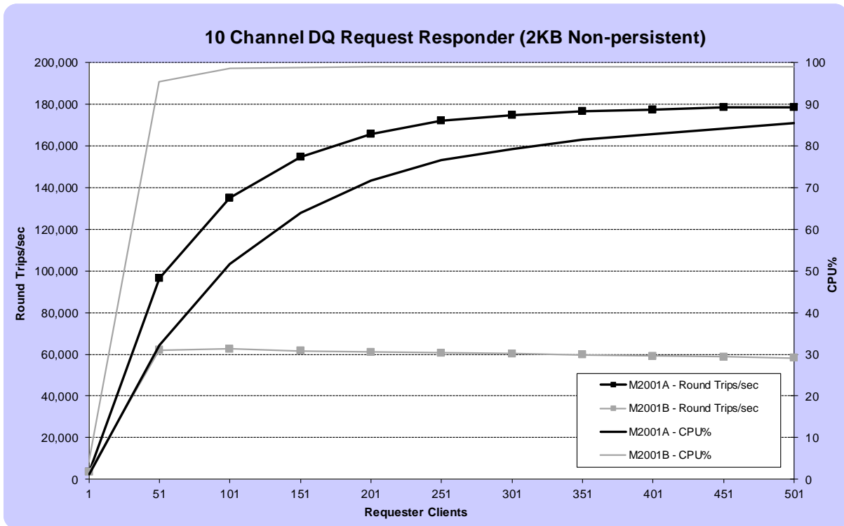
FIGURE 8 - PERFORMANCE RESULTS FOR 2KB, 10 CHANNEL DQ NON-PERSISTENT MESSAGING
