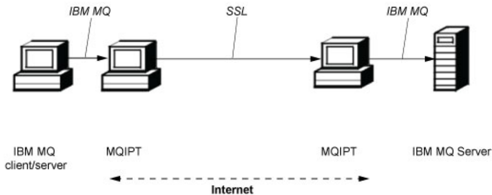
Figure 4. Example of MQIPT and SSL/TLS
