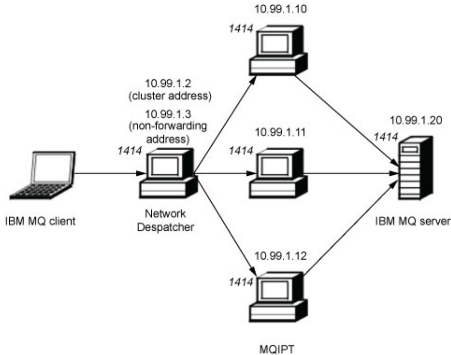
Figure 5. Using the Network Dispatcher with MQIPT
