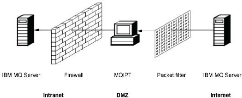
Figure 2. Example of MQIPT in a DMZ firewall
