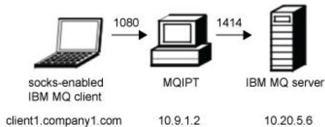
Figure 11. SOCKS proxy network diagram
