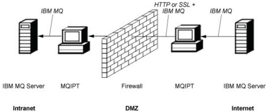
Figure 3. Example of MQIPT and HTTP tunneling
