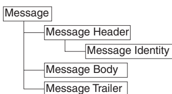
Figure 1. Multipart message structure
