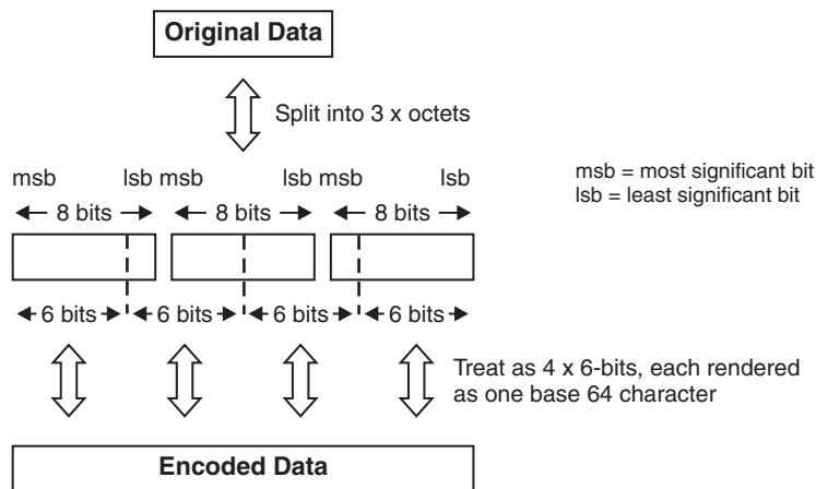
Figure 1. base64 data transformation
