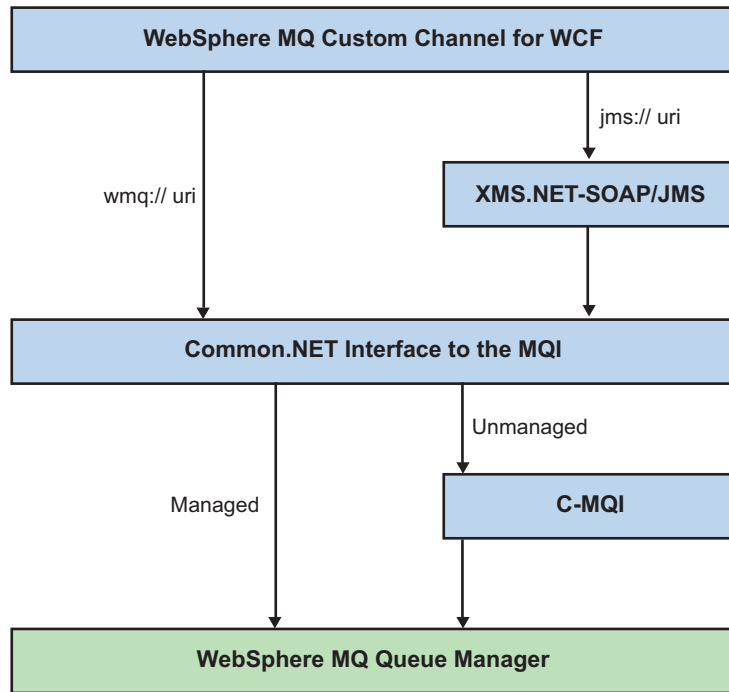
Figure 184. WCF architecture for the Non-SOAP/Non-JMS interface
