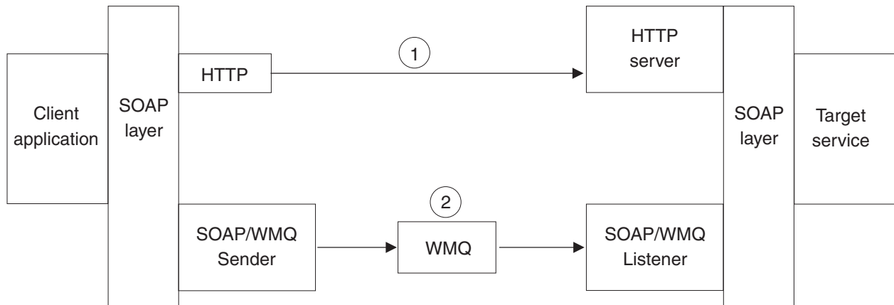
Figure 186. Overview of IBM MQ transport for SOAP
