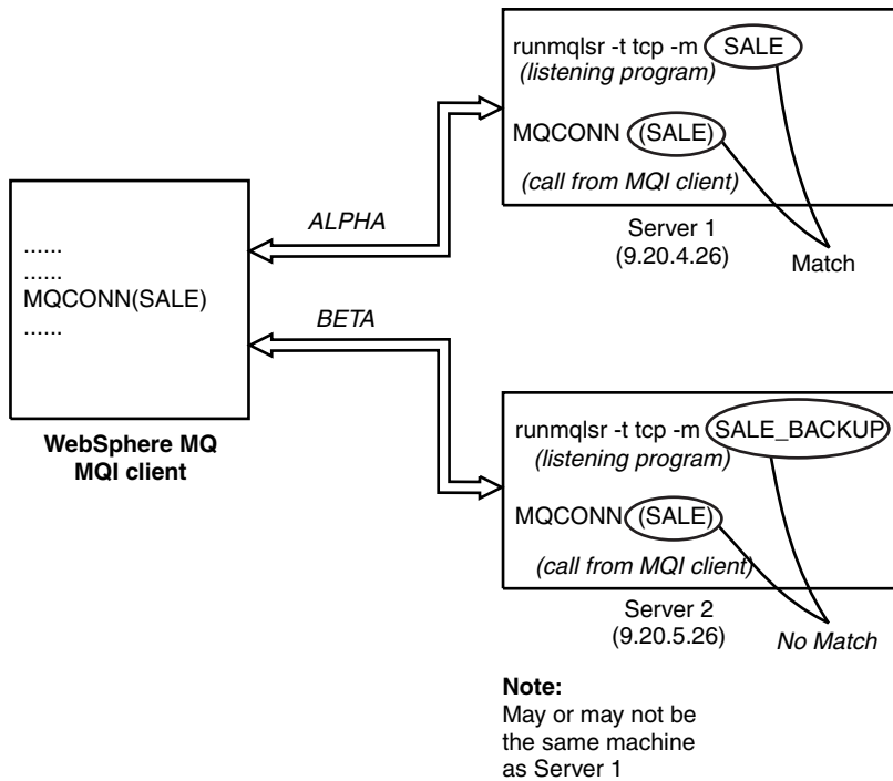
Figure 51. MQCONN example
