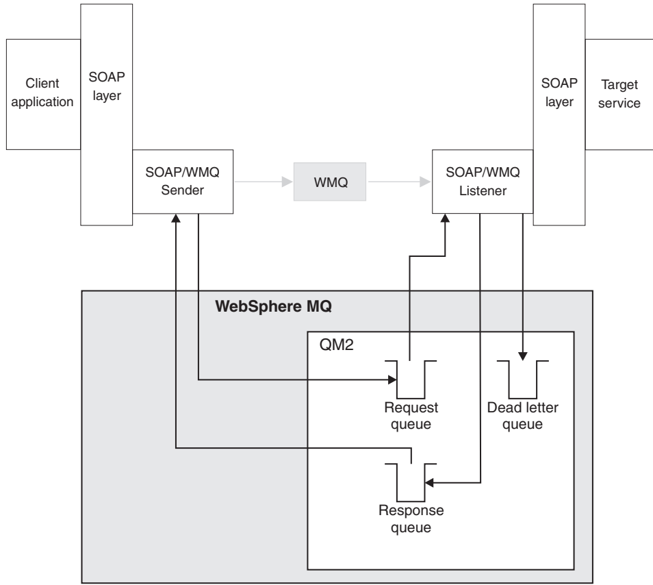
Figure 187. Queues used by SOAP/IBM MQ (single queue manager)
