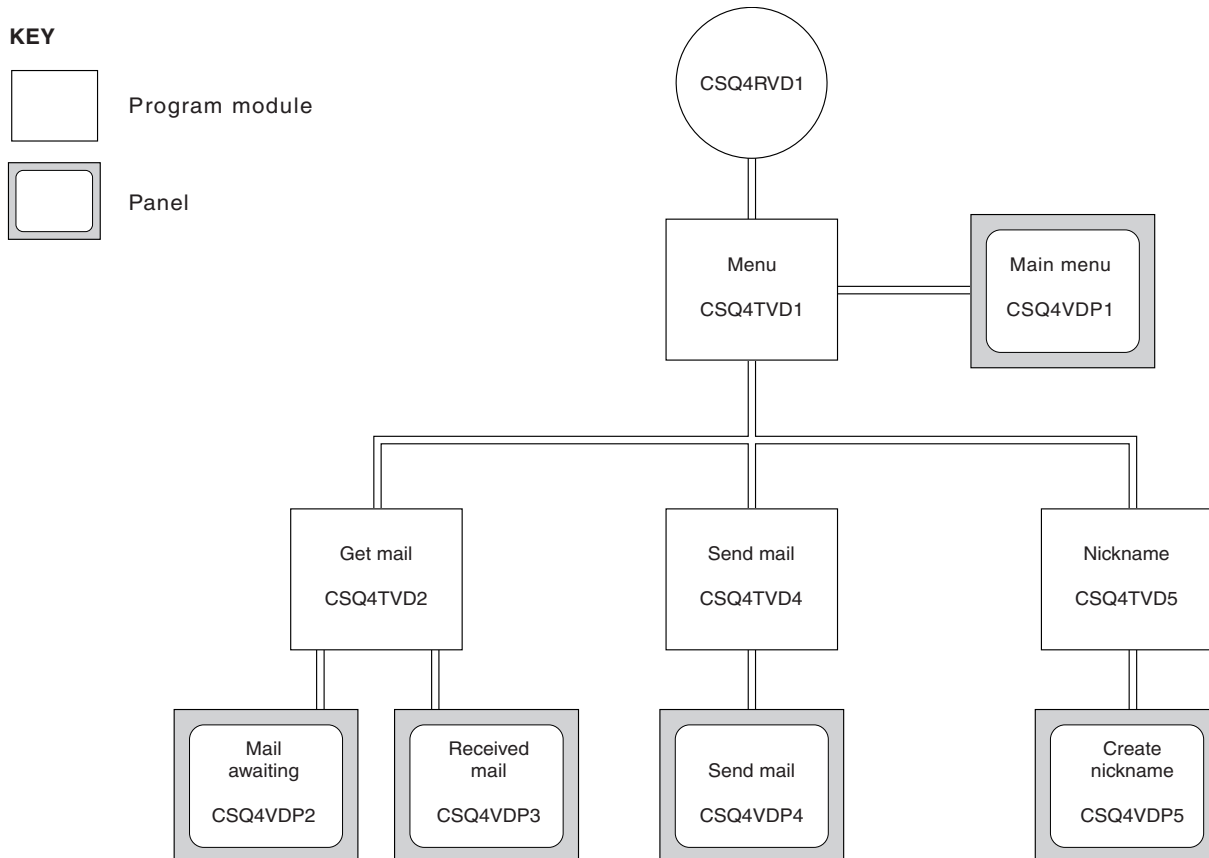
Figure 95. Programs and panels for the TSO versions of the Mail Manager. This figure shows the names for the COBOL version.
