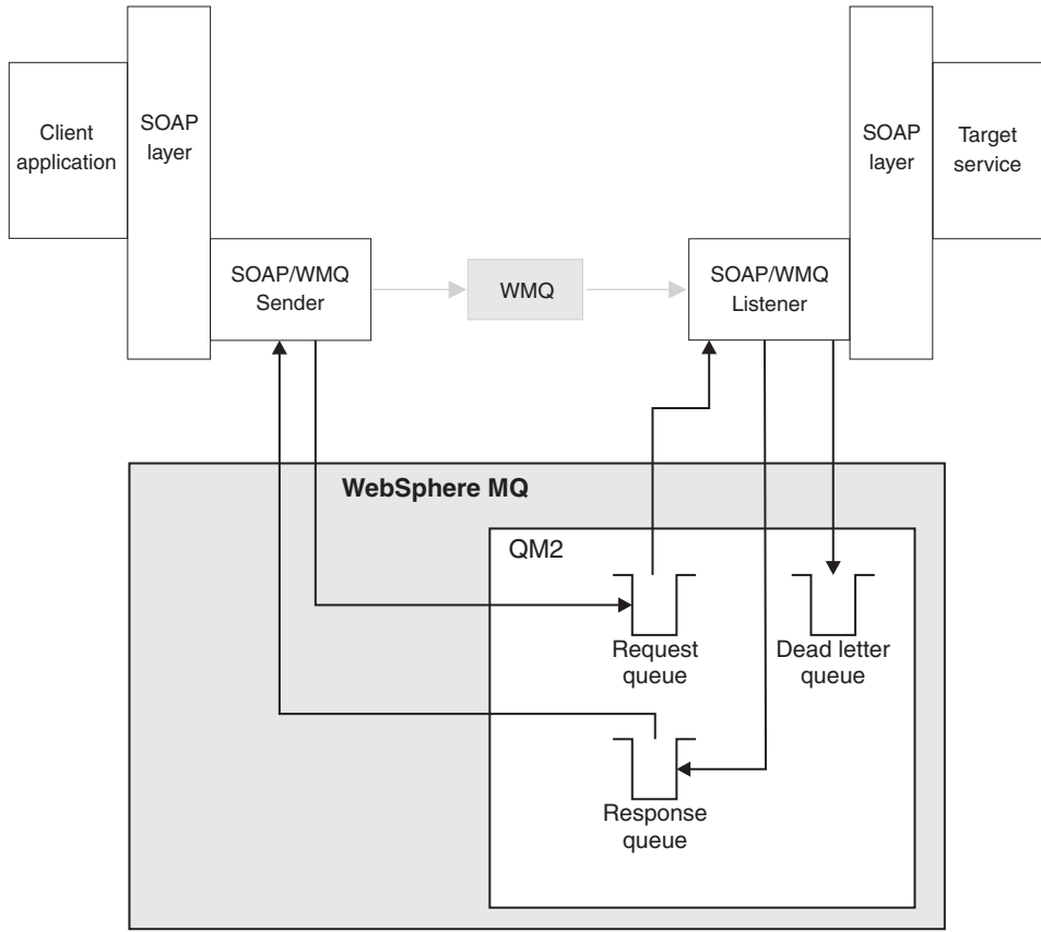
Figure 154. Queues used by SOAP/IBM MQ (single queue manager)
