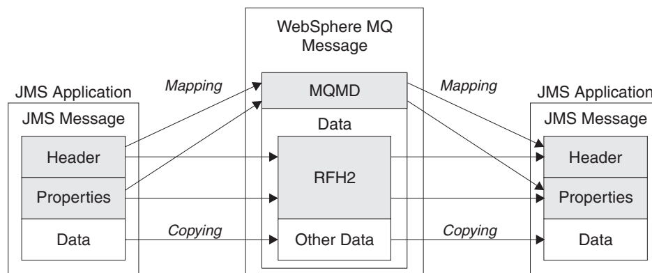
Figure 108. How messages are transformed between JMS and IBM MQ using the MQRFH2 header
