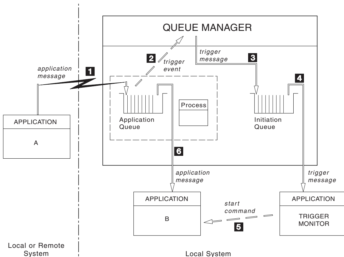
Figure 48. Flow of application and trigger messages
