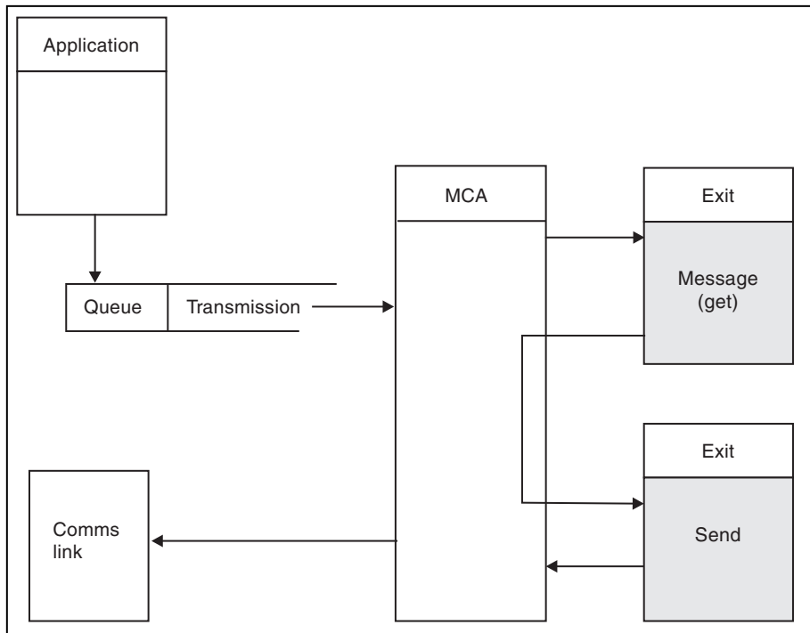
Figure 59. Example of a send exit at the sender end of message channel
