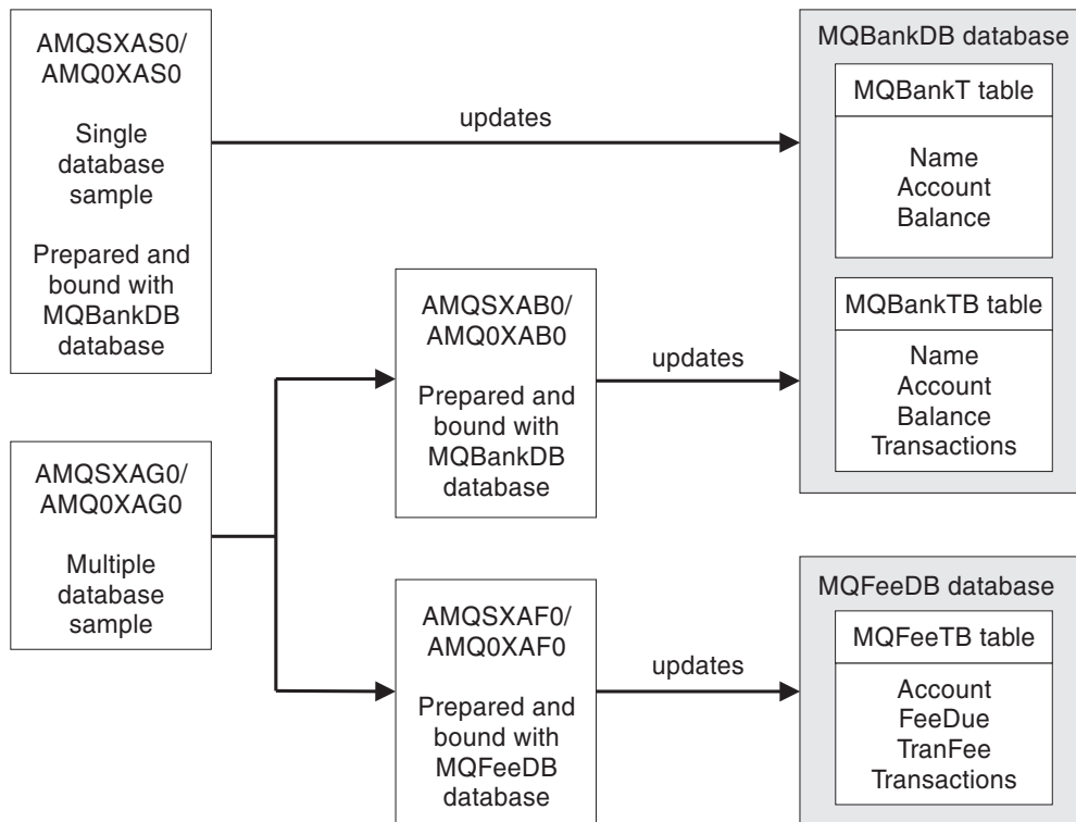
Figure 83. The database coordination samples
