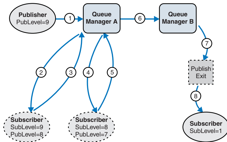
Figure 46. Interception and Publish exit in a cluster
