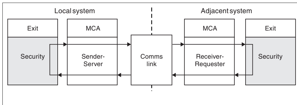
Figure 58. Security exit loop
