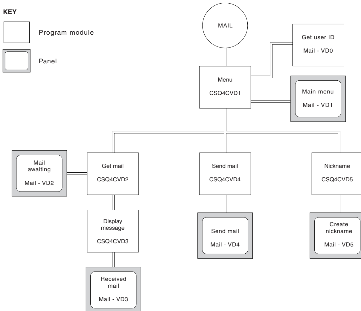
Figure 96. Programs and panels for the CICS version of the Mail Manager
