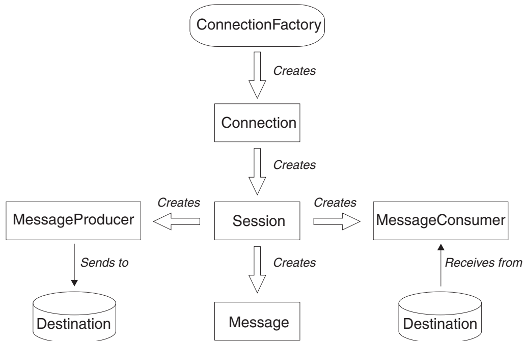
Figure 107. JMS objects and their relationships
