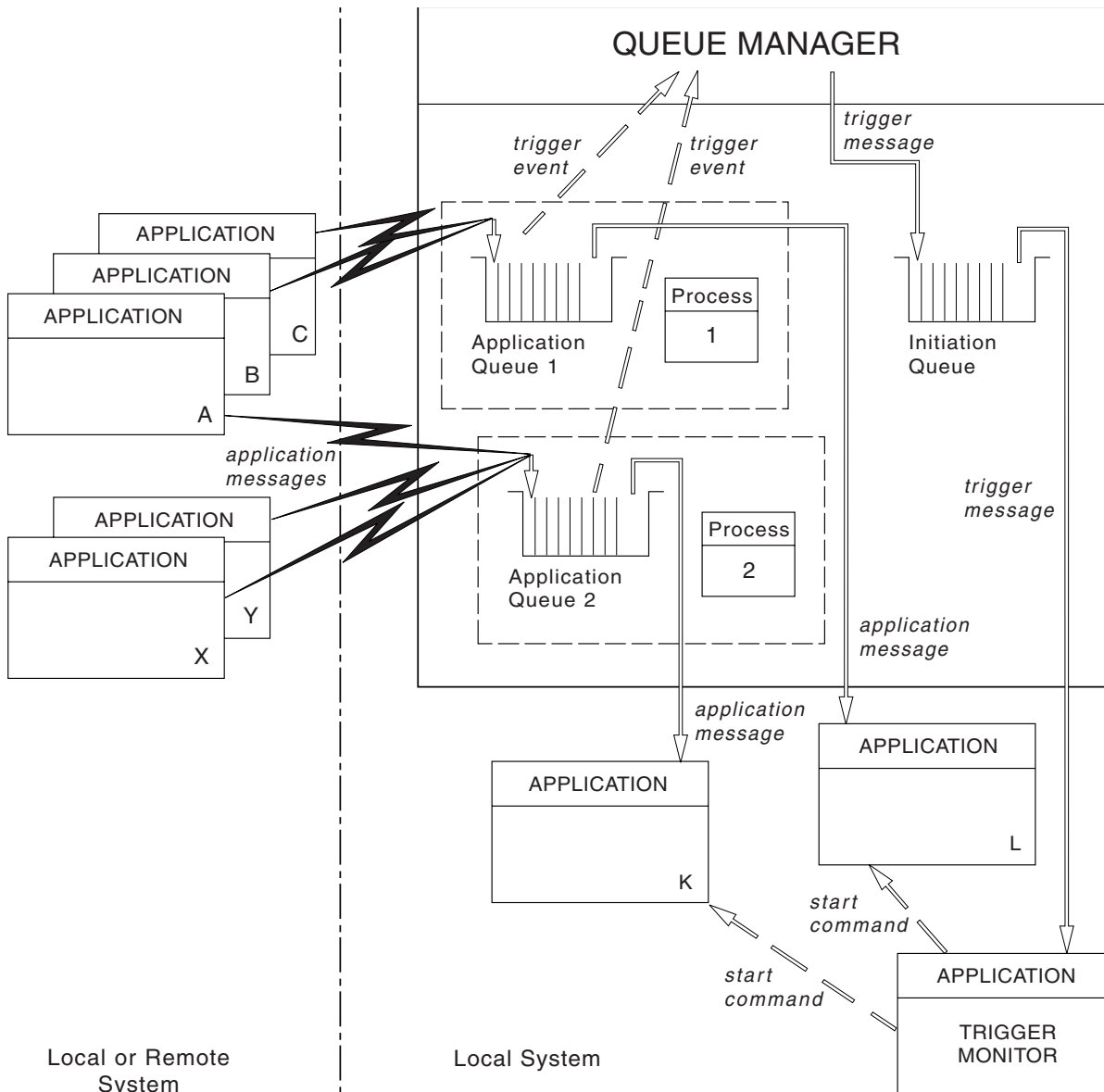
Figure 49. Relationship of queues within triggering
