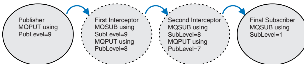
Figure 39. Sequence of intercepting subscribers
