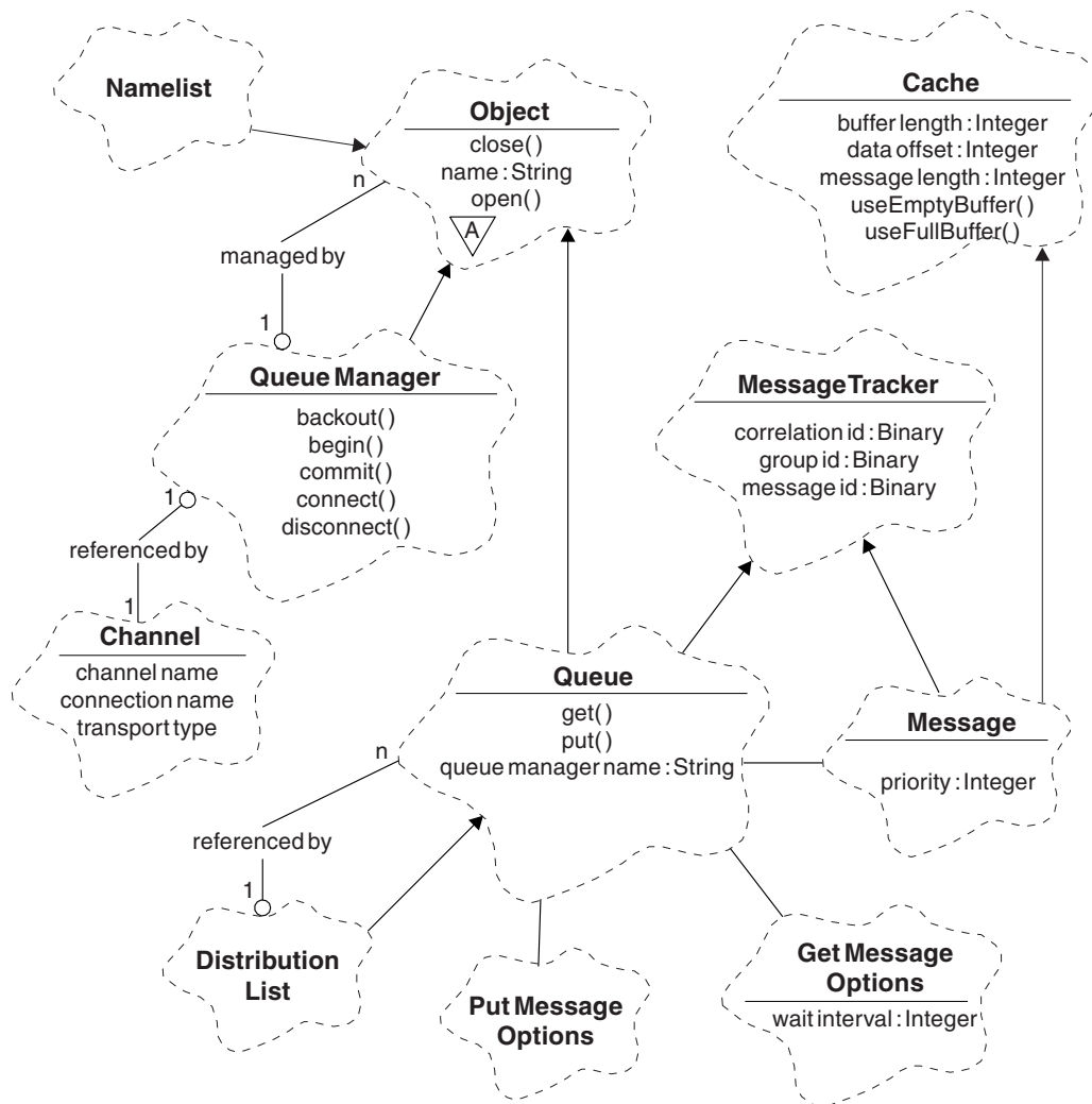
Figure 106. IBM MQ C++ classes (queue management)
