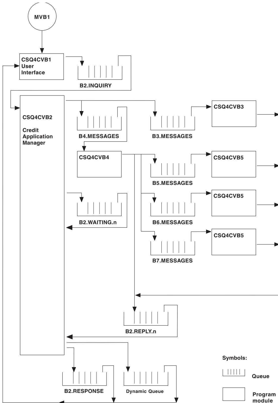
Figure 100. Programs and queues for the Credit Check sample application (COBOL programs only). In the sample application, the queue names shown in this figure have the prefix CSQ4SAMP.
