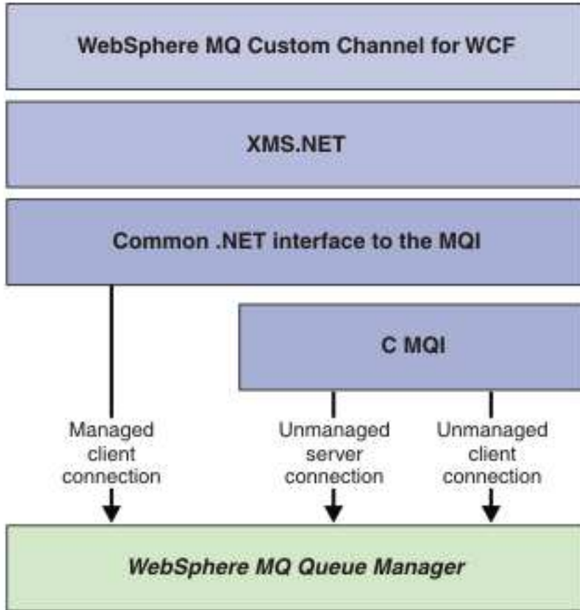
Figure 150. WCF architecture for the SOAP/JMS interface
