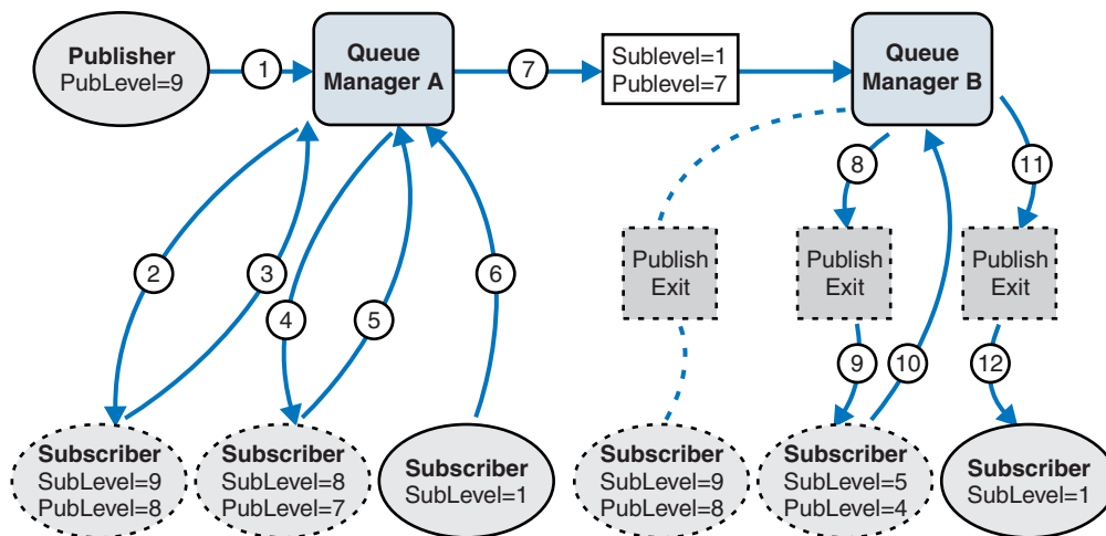
Figure 47. Complex deployment of intercepting subscribers
