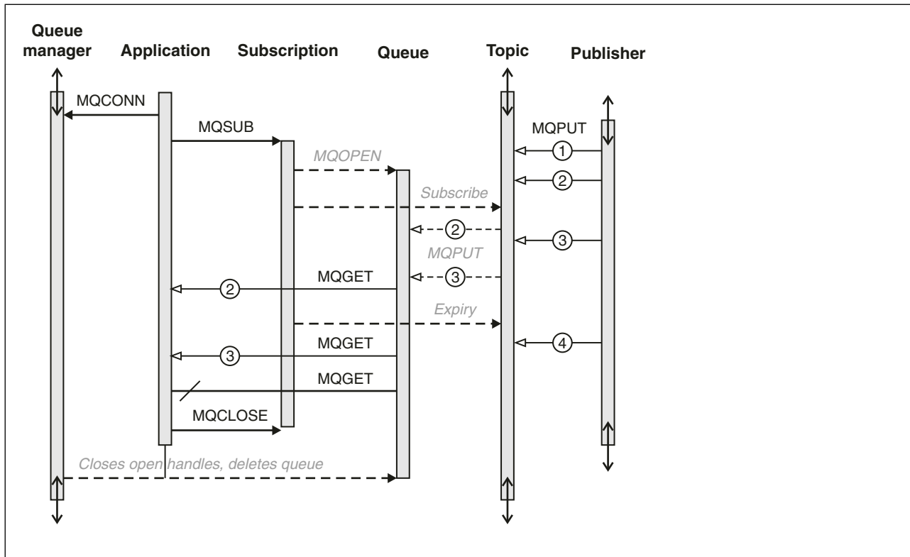
Figure 36. Managed non-durable subscriber lifelines
