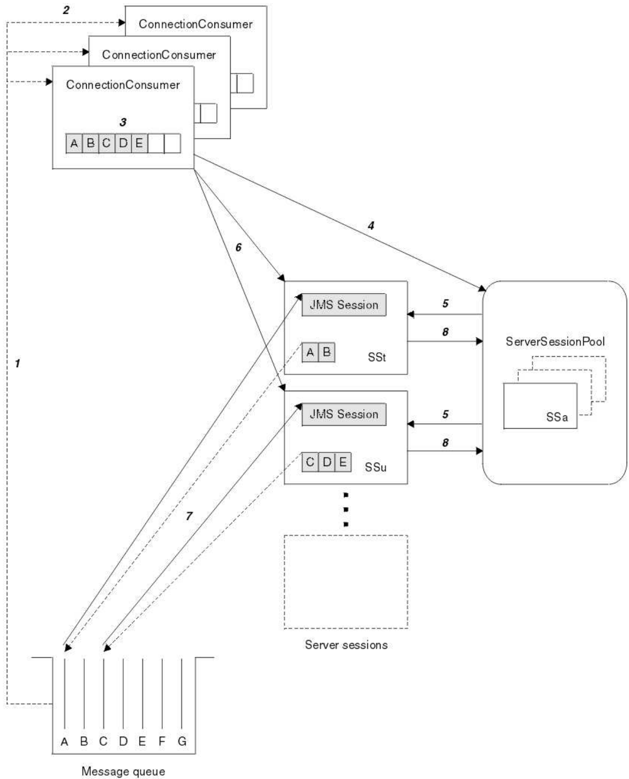
Figure 145. ServerSessionPool and ServerSession functionality
