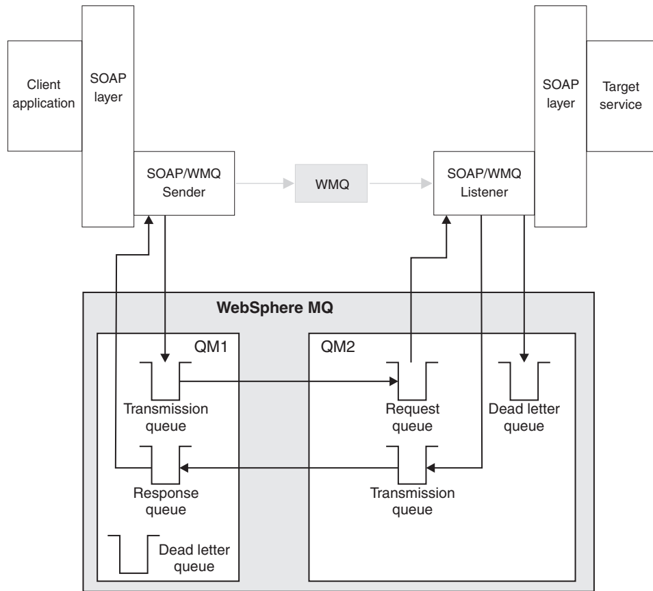
Figure 155. Queues used by SOAP/IBM MQ (separate queue managers)
