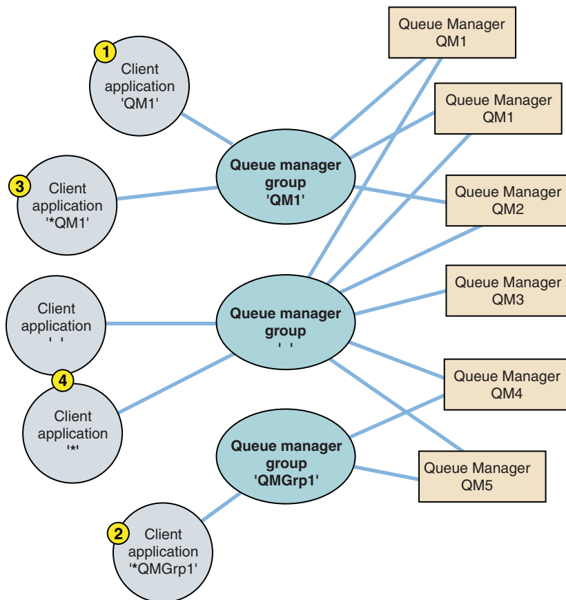
Figure 50. Queue manager groups
