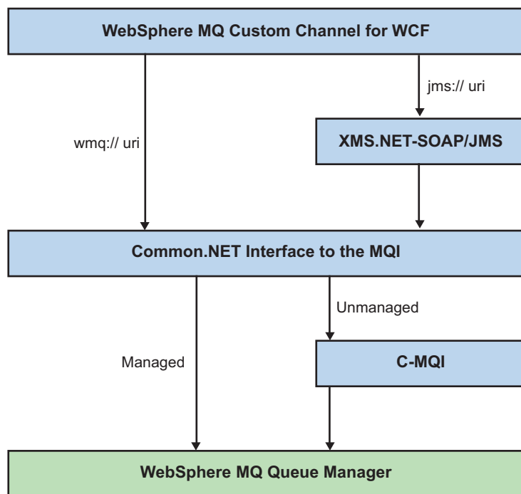
Figure 151. WCF architecture for the Non-SOAP/Non-JMS interface
