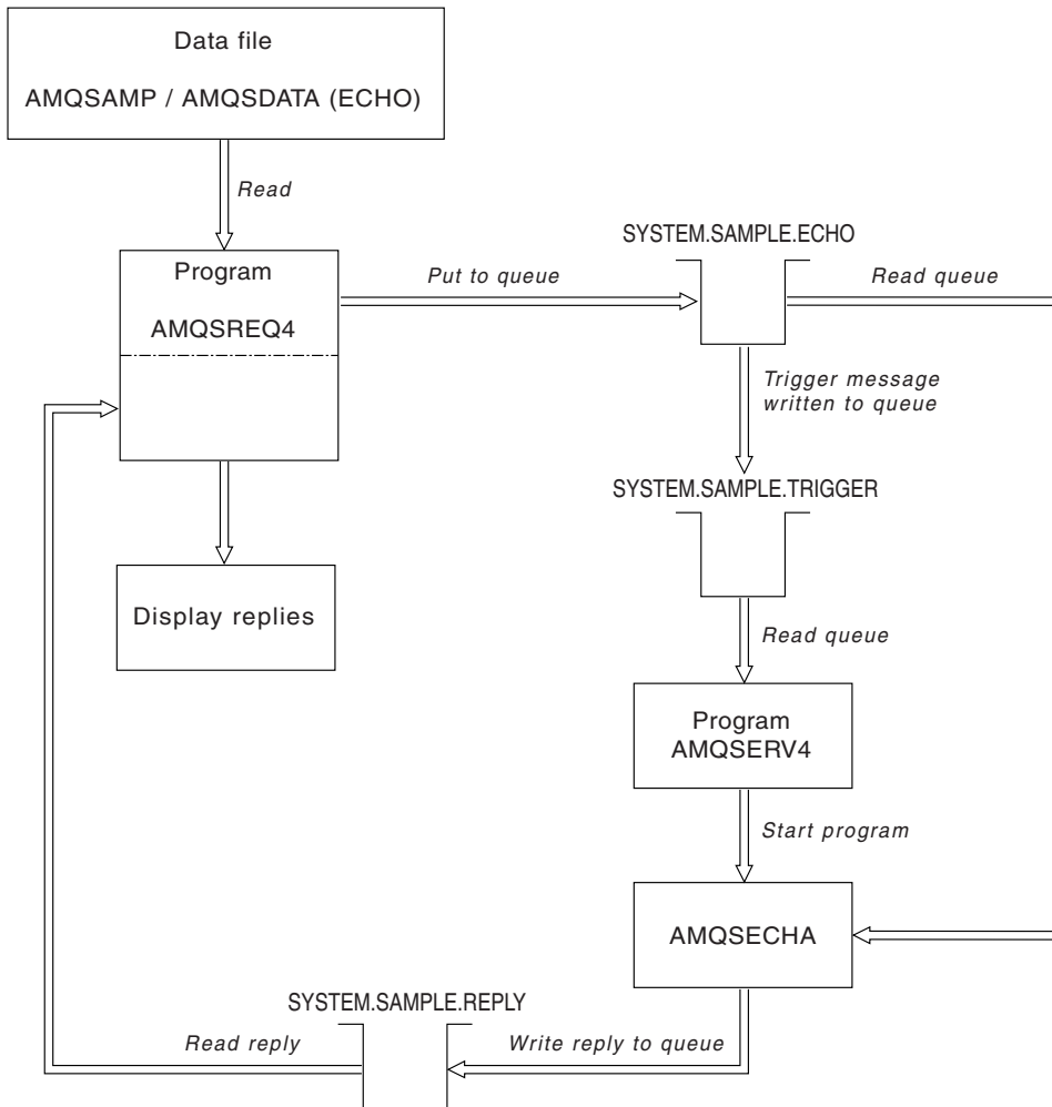
Figure 88. Sample IBM i Client/Server (Echo) program flowchart
