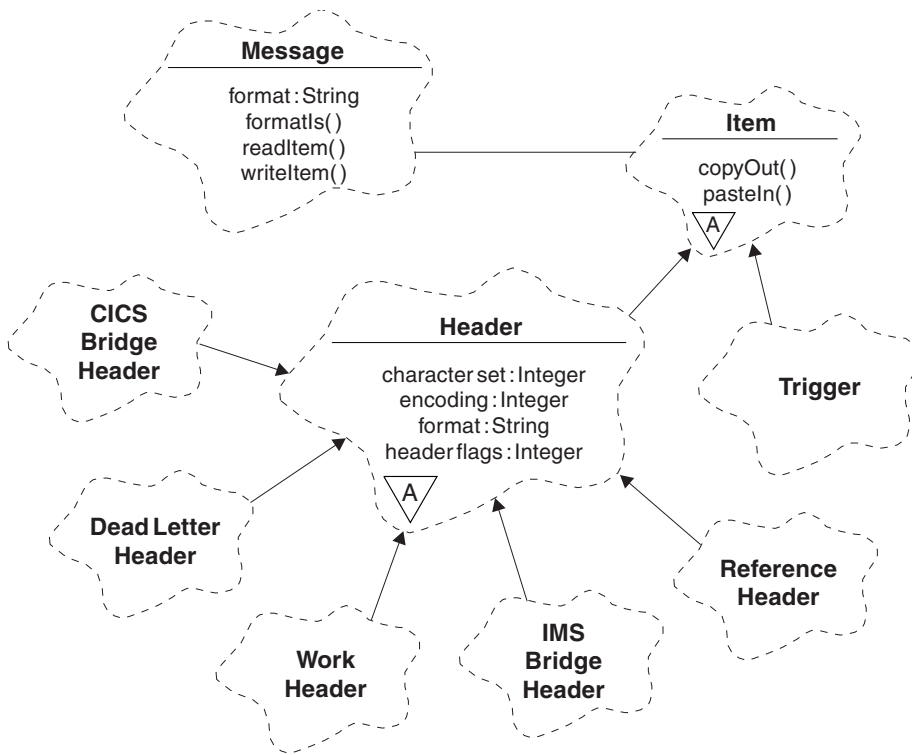
Figure 105. IBM MQ C++ classes (item handling)
