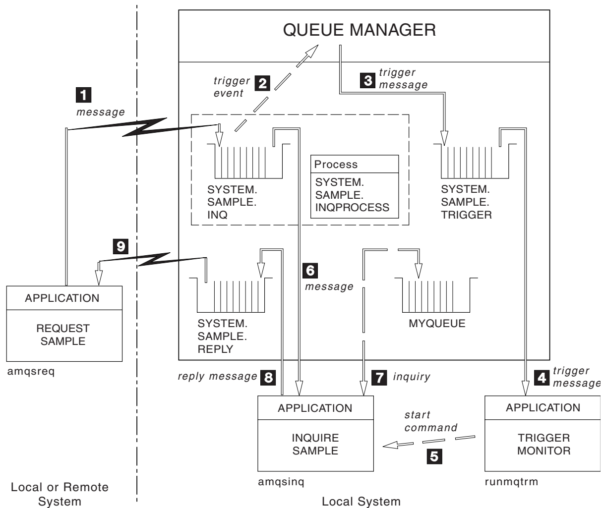
Figure 87. Request and Inquire samples using triggering
