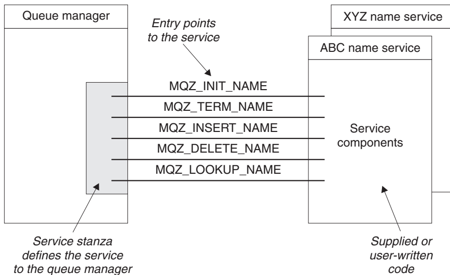
Figure 52. Understanding services, components, and entry points
