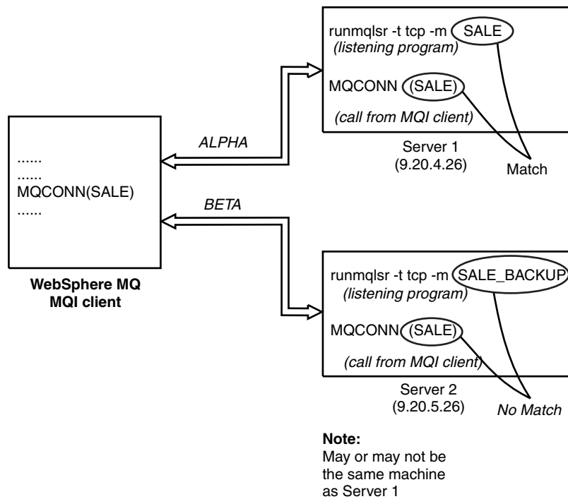
Figure 51. MQCONN example
