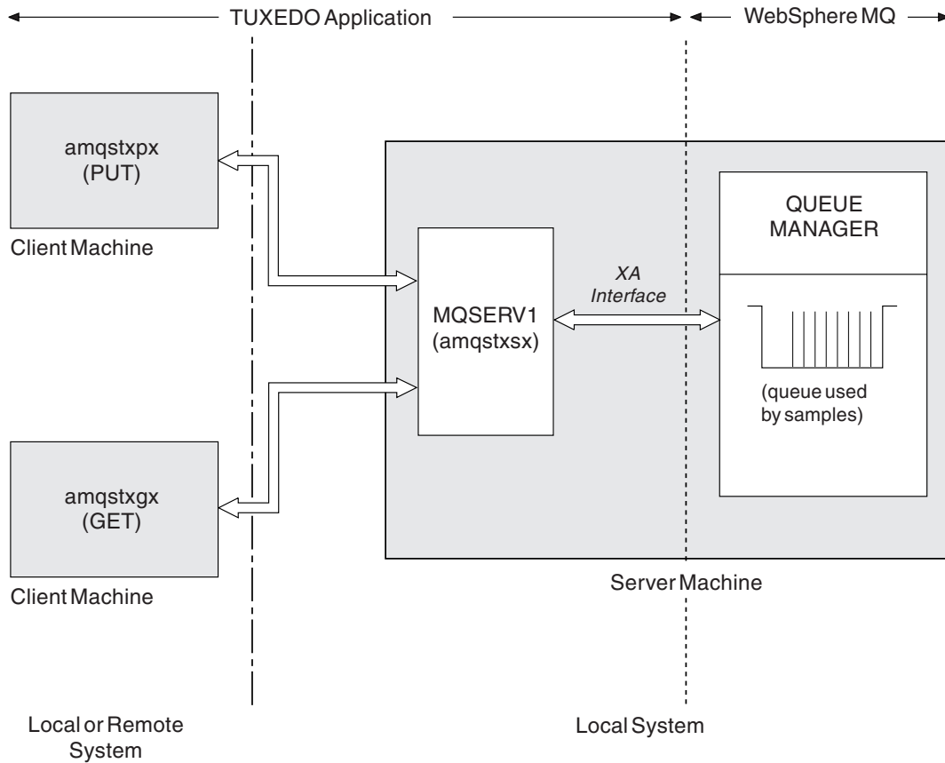
Figure 93. How TUXEDO samples work together
