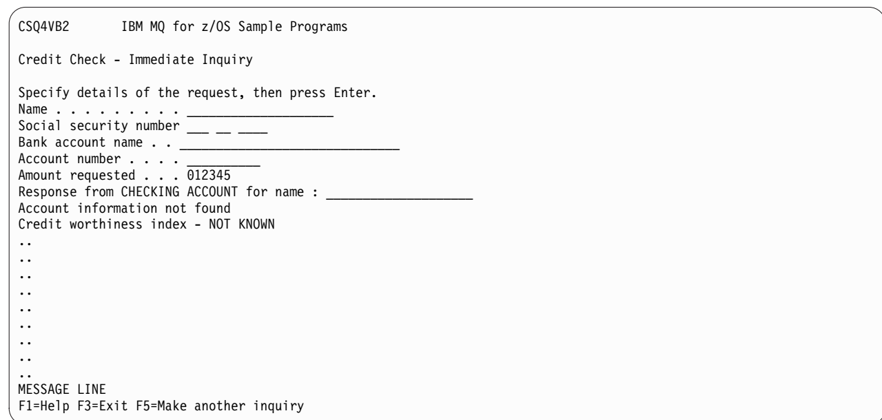
Figure 99. Immediate Inquiry panel for the Credit Check sample application
