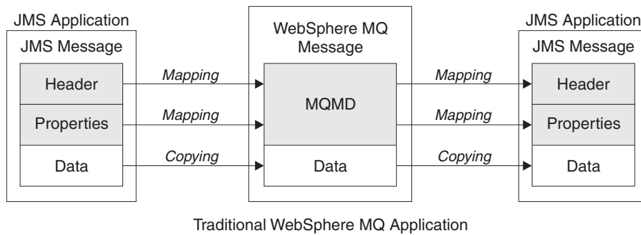
Figure 109. How JMS messages are transformed to IBM MQ messages with no MQRFH2 header
