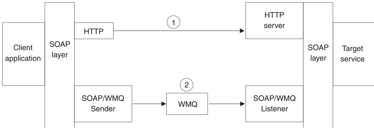
Figure 153. Overview of IBM MQ transport for SOAP
