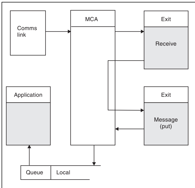
Figure 60. Example of a receive exit at the receiver end of message channel
