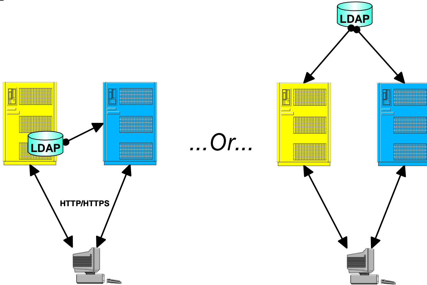
Domino as LDAP
