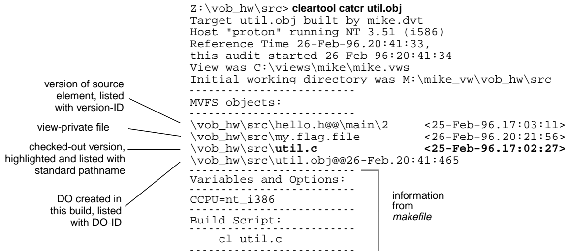
Figure 3 Kinds of Information in a Configuration Record
