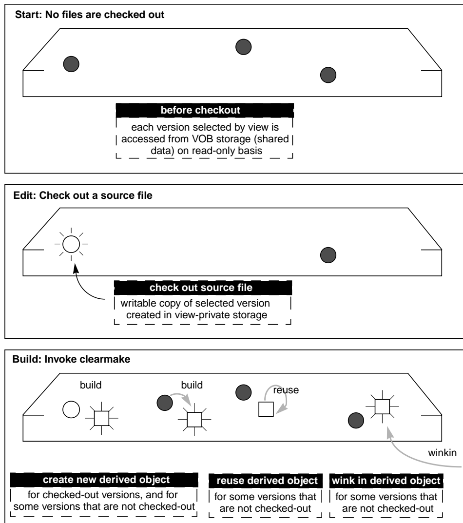
Figure 7 clearmake Build Scenario
