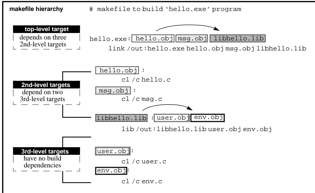
Figure 4 Configuration Record Hierarchy
