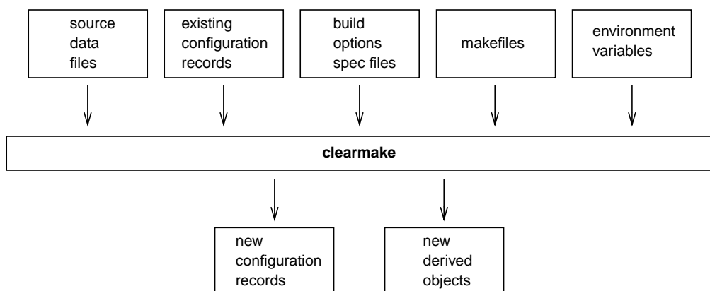
Figure 6 Data Flow in a clearmake Build
