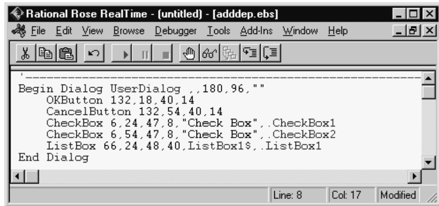
Figure 16 Sample dialog in Basic Script
