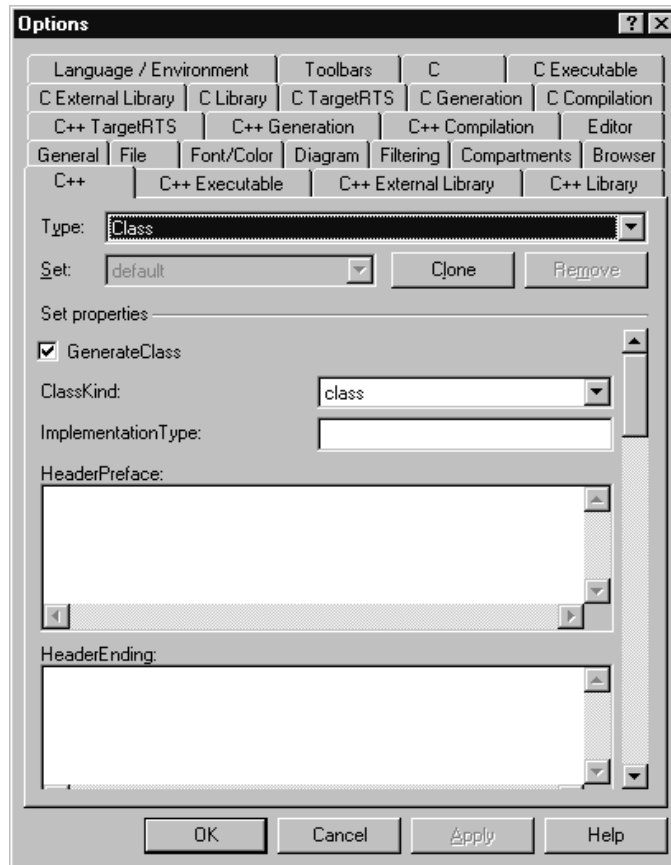
Figure 4 Specification Editor
