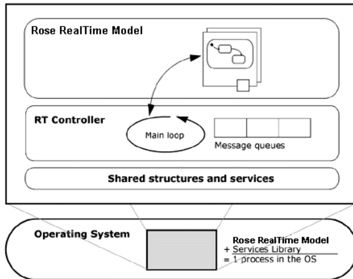
Figure 5 Single-Threaded Services Library
