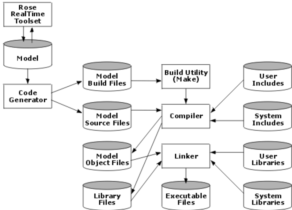
Figure 3 Compilation Paradigm for Producing C Executable
