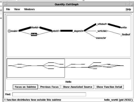
CALL GRAPH
