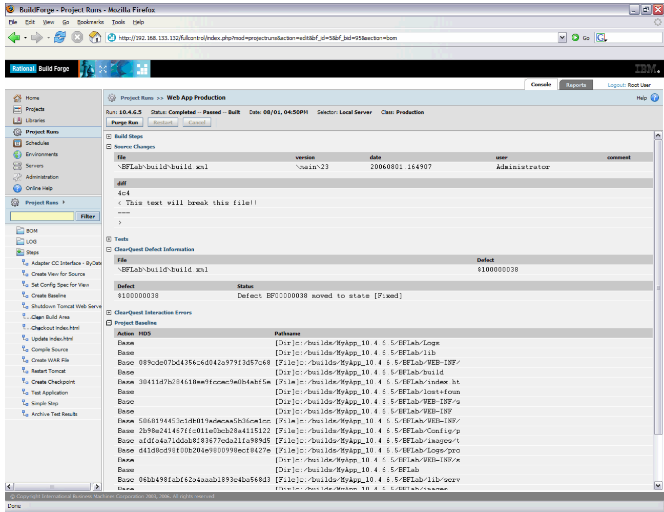
Figure 2: Build Forge bill-of-materials provides an automated, detailed record of release components
