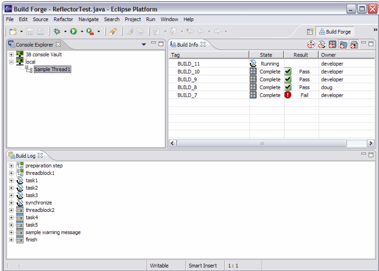
Figure 3: Build Forge plug-ins for Eclipse and VisualStudio .NET let developers run pre-configured CM processes to validate code changes and get real-time feedback.
