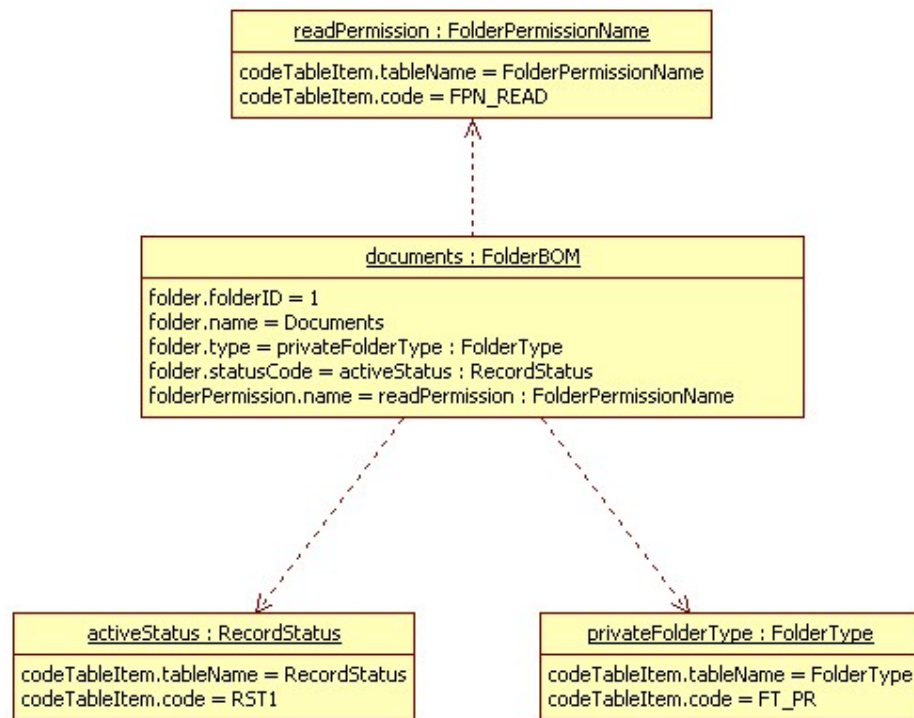
Figure 3.5 Instance-level relationships between Folder BOM and CodeTable BOM
