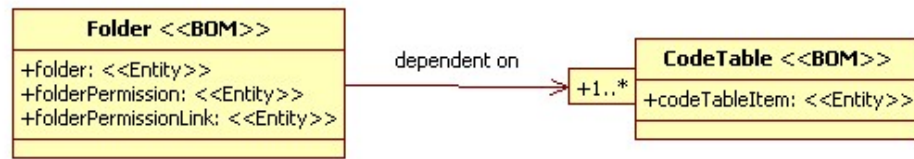
Figure 3.3 Type-level relationship between Folder BOM and CodeTable BOM
