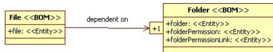
Figure 3.4 Type-level relationship between File BOM and Folder BOM
