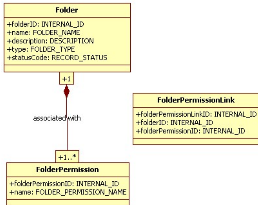
Figure 3.1 UML representation for folder screen entities
