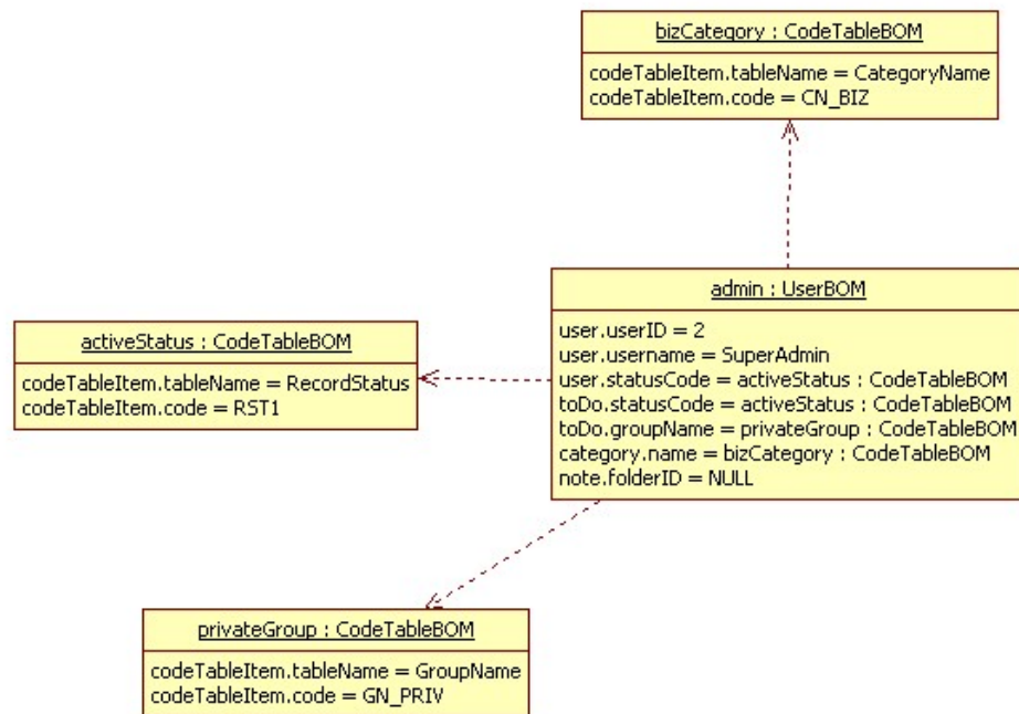
Figure 3.9 Instance-level relationships for User BOM
