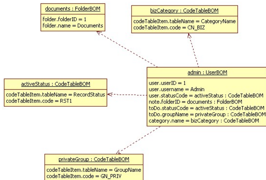
Figure 3.8 Instance-level relationships for User BOM
