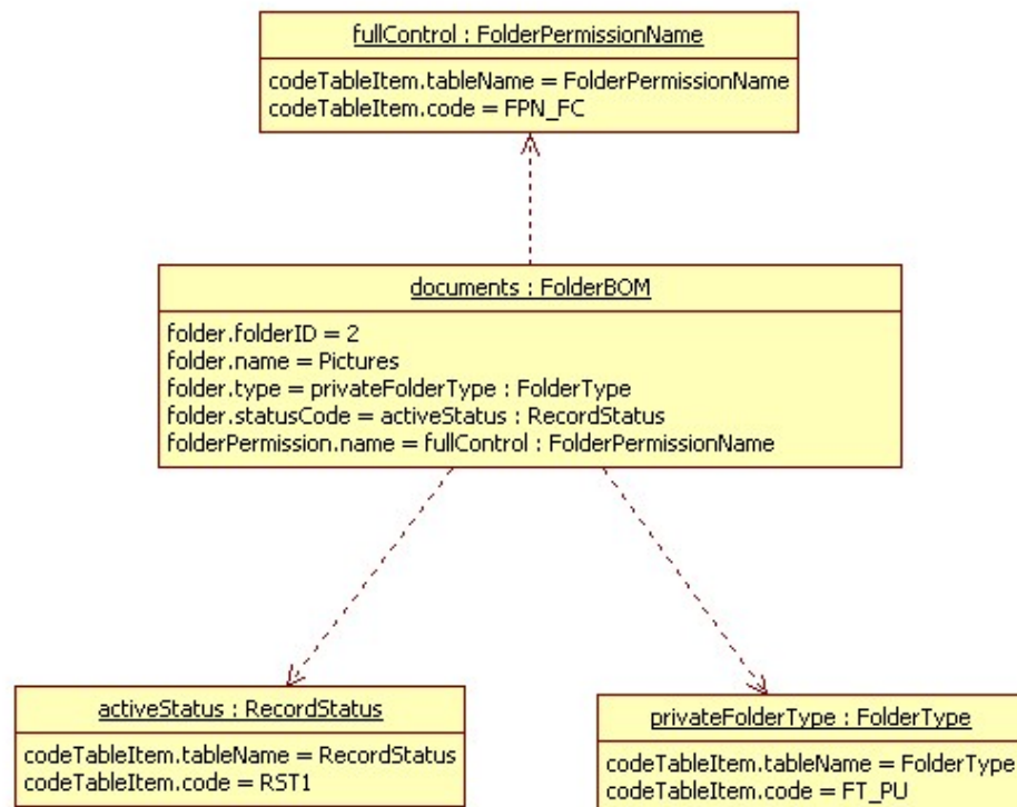
Figure 3.6 Instance-level relationships between Folder BOM and CodeTable BOM
