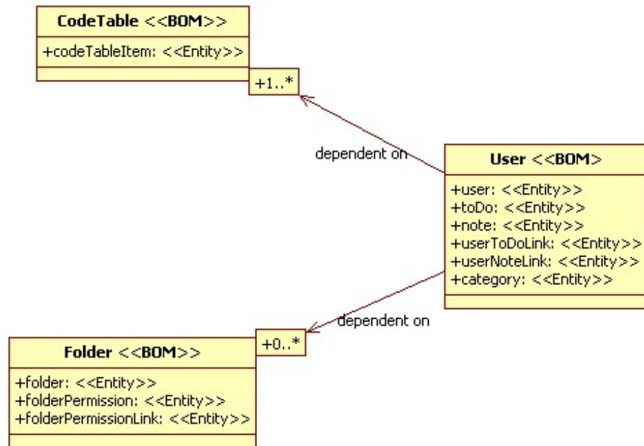
Figure 3.7 Type-level relationships for User BOM
