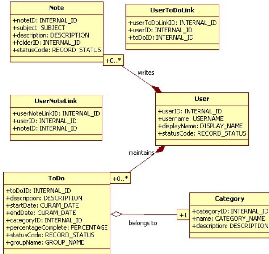
Figure 3.2 UML representation for user screen entities
