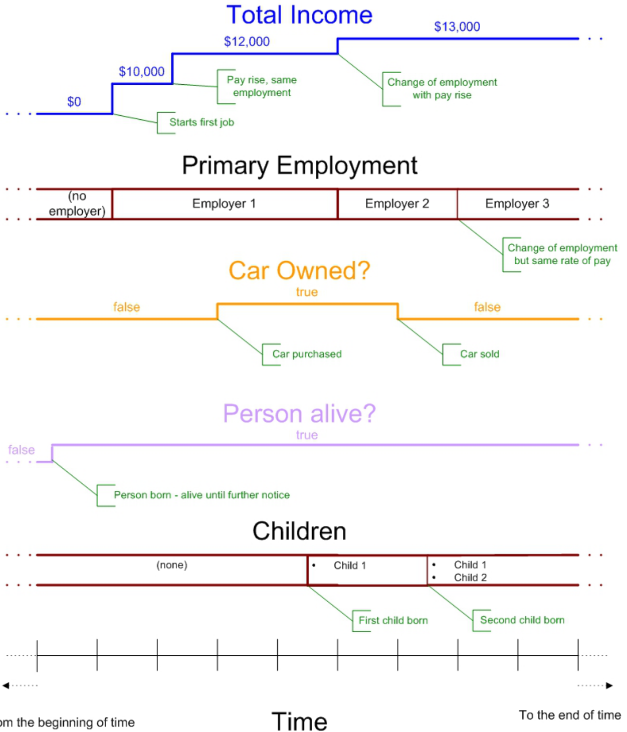
Figure 19. Examples of Timeline Data
