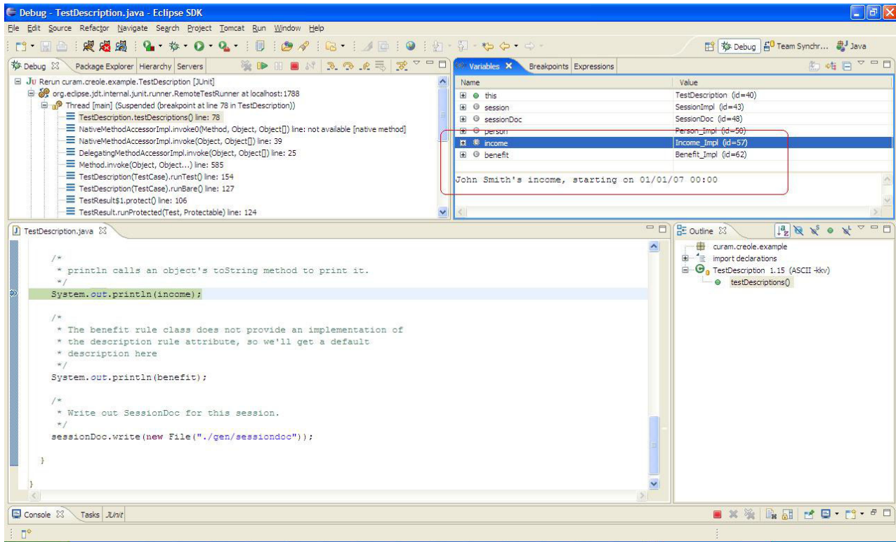
Figure 34. Use of description in an integrated development environment
