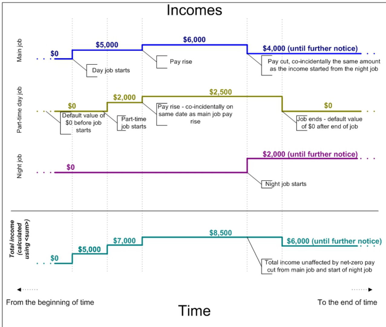
Figure 24. A Total Income Timeline, Calculated using sum
