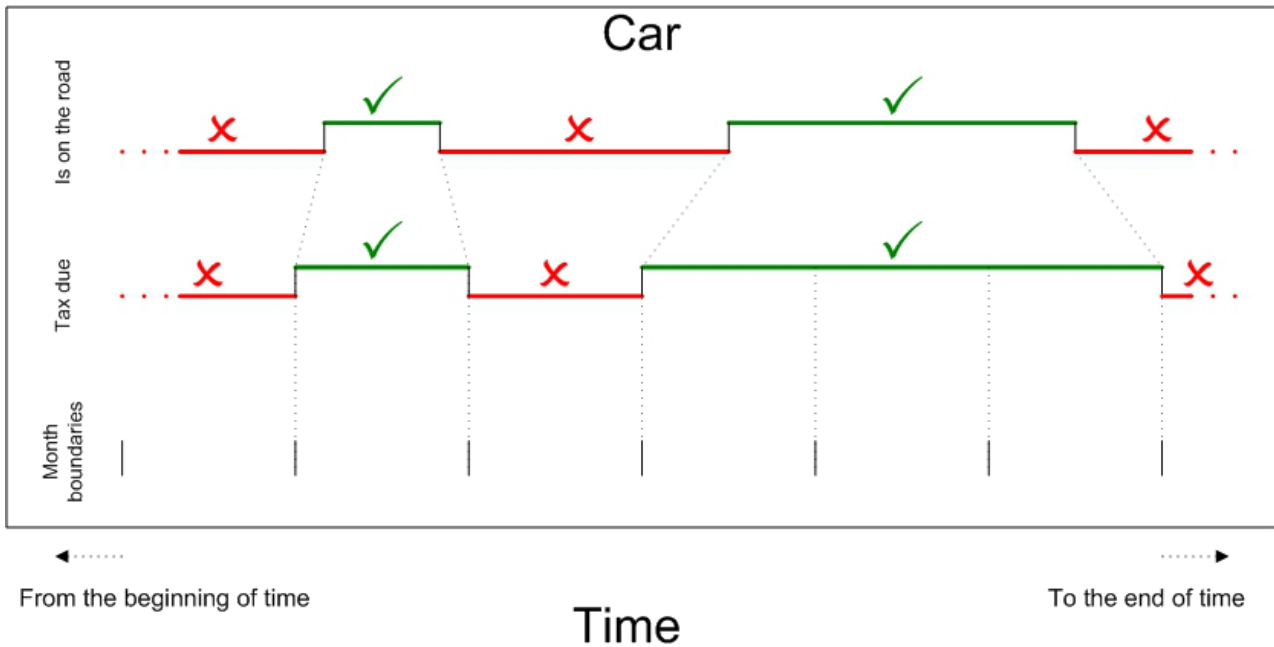
Figure 26. A Requirement for a Date-Spreading Timeline
