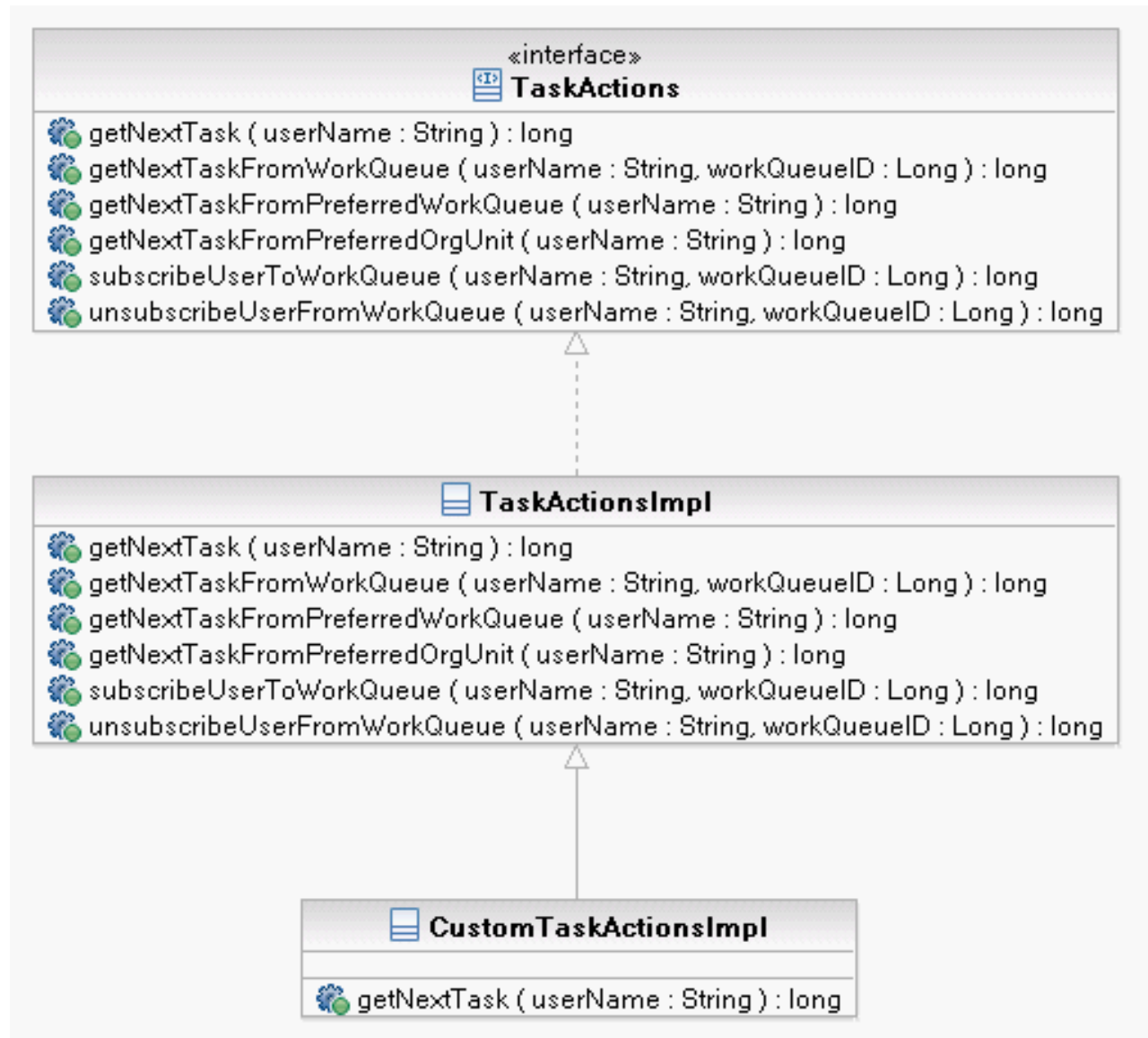
Figure 5. Customization Class Diagram
