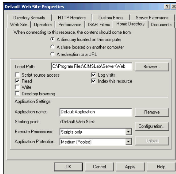
Figure 2-21 • Default Web Site Properties Dialog Box—Home Directory Tab
