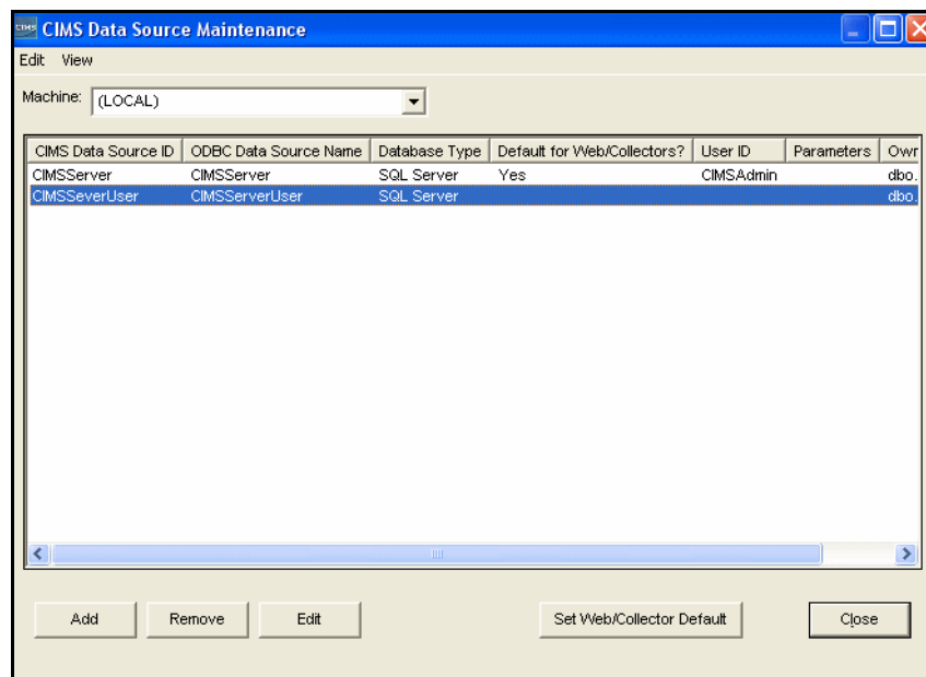
Figure 2-8 • CIMS Data Source Maintenance Dialog Box—SQL Server Example 3
