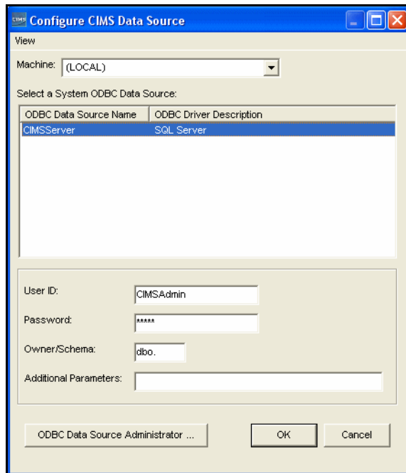
Figure 2-3 • Configure CIMS Data Source Dialog Box—SQL Server Example 1
