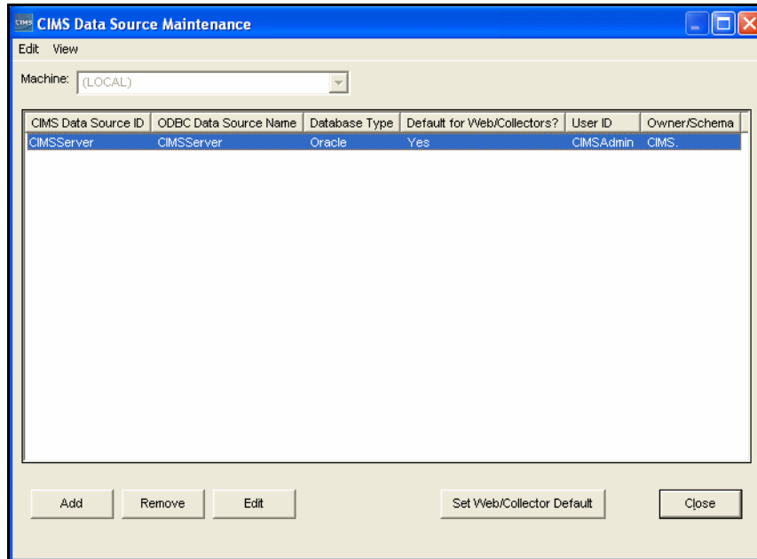
Figure 2-12 • CIMS Data Source Maintenance Dialog Box—Oracle Example 1
