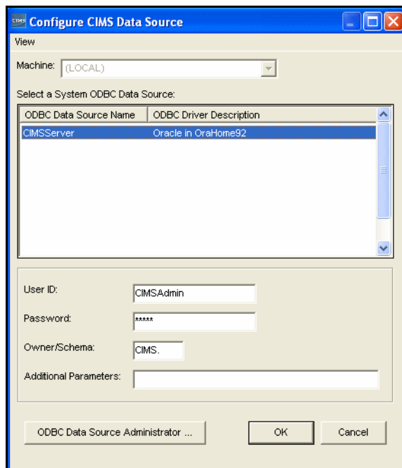
Figure 2-11 • Configure CIMS Data Source Dialog Box—Oracle Example 1
