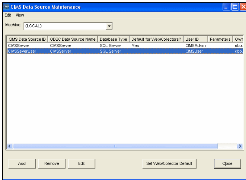
Figure 2-6 • CIMS Data Source Maintenance Dialog Box—SQL Server Example 2
