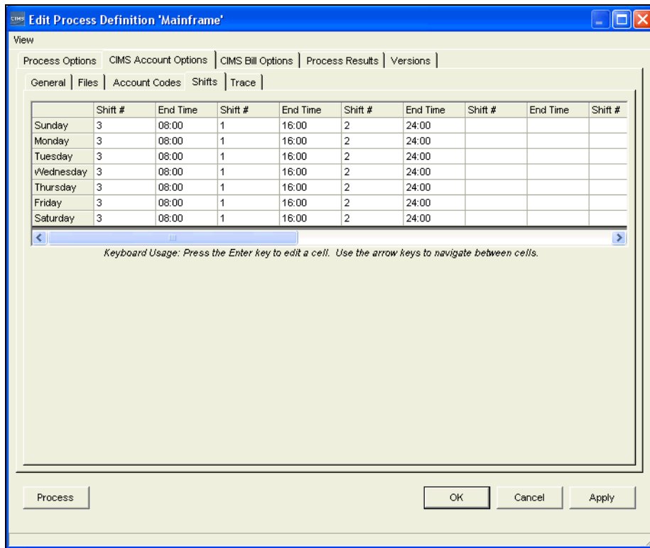
Figure 6-2 • Shifts Subtab
