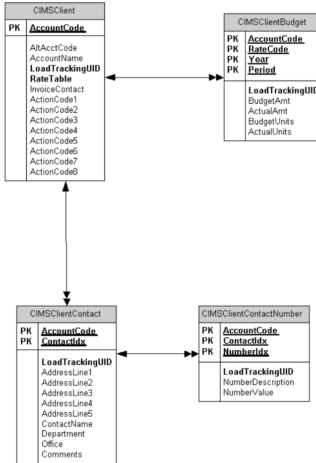
Figure A-2 • Client Tables ERD
