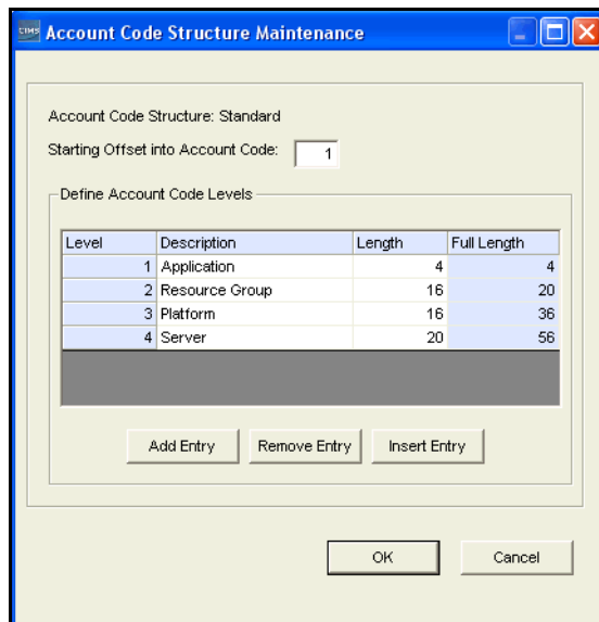
Figure 2-19 • Account Code Structure Maintenance Dialog Box
