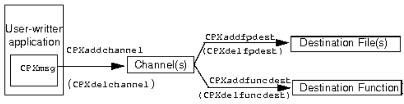
CPLEX message handling routines
