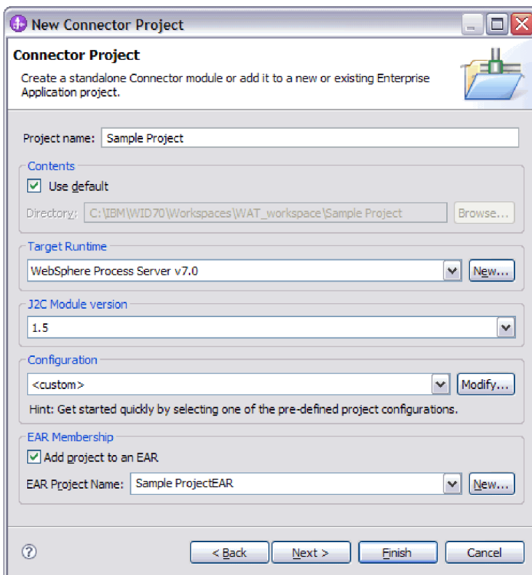
Figure 4. New Connector Project wizard
