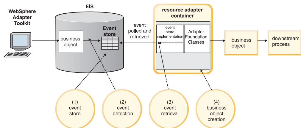
Inbound event notification
