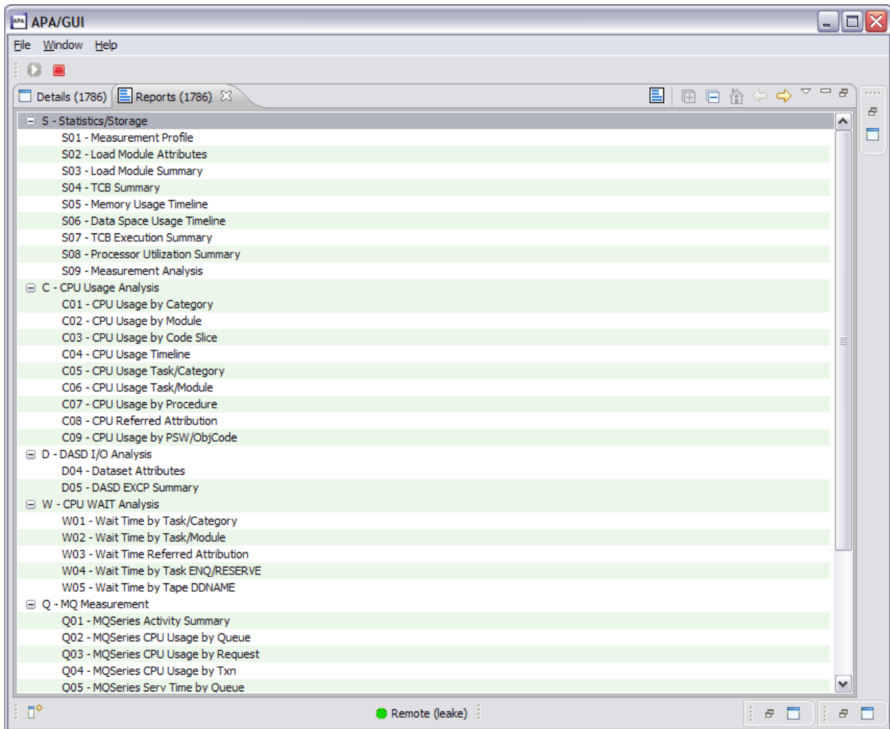
Figure 39. Observation Reports List view
