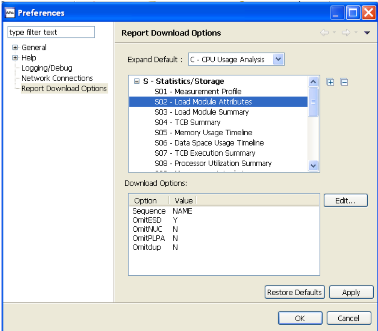
Figure 15. Report download options dialog
