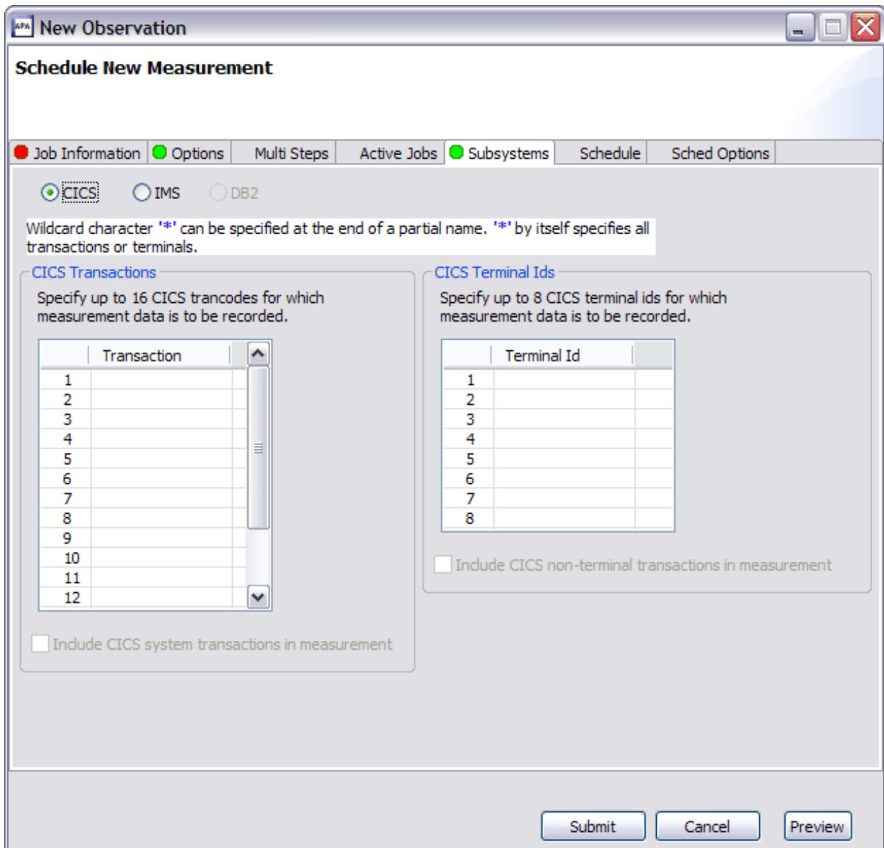
Figure 28. Subsystems tab - CICS option
