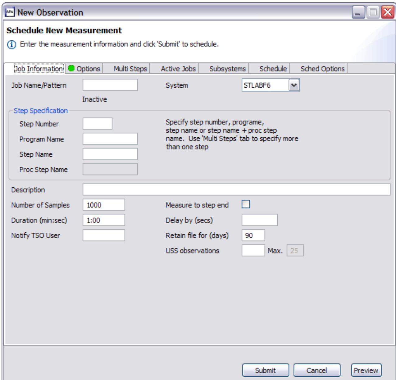
Figure 23. Job Information tab
