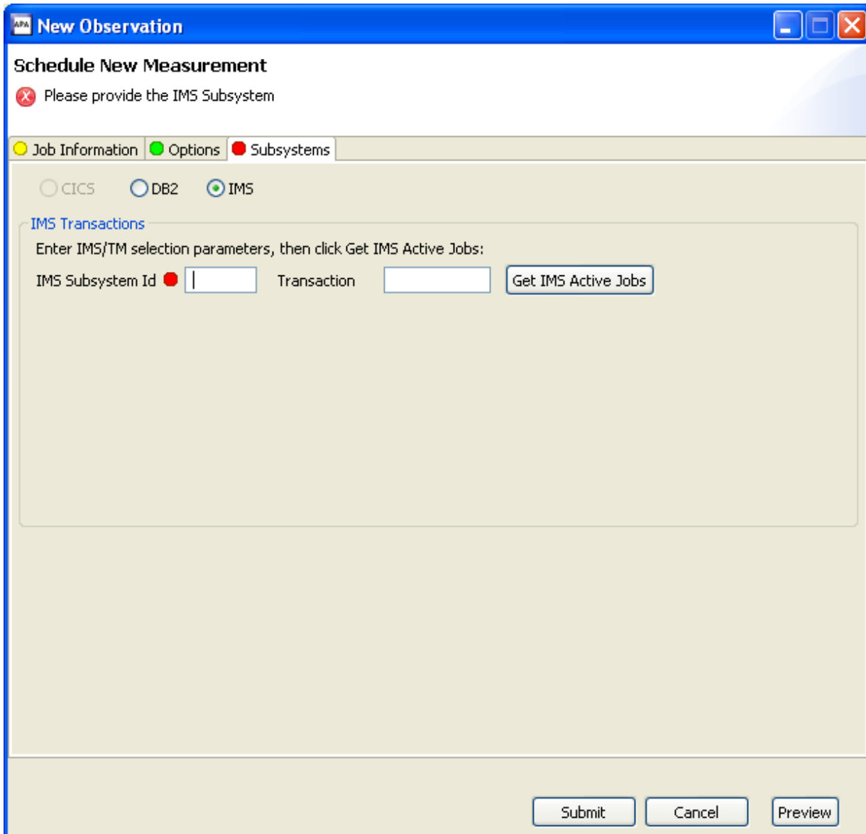
Figure 31. Subsystems tab - IMS Multiple Address Space option
