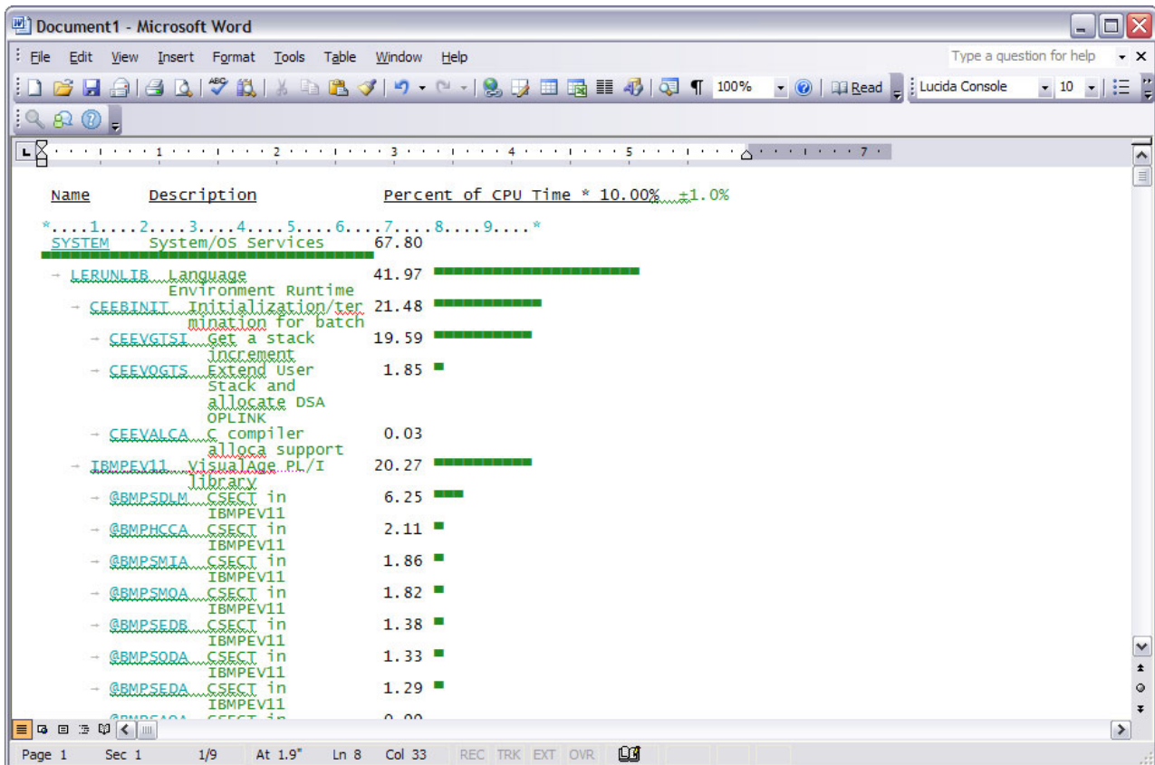
Figure 45. Copy/Paste report to Word sample
