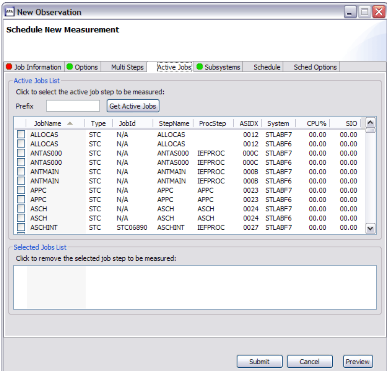
Figure 27. Active Jobs tab
