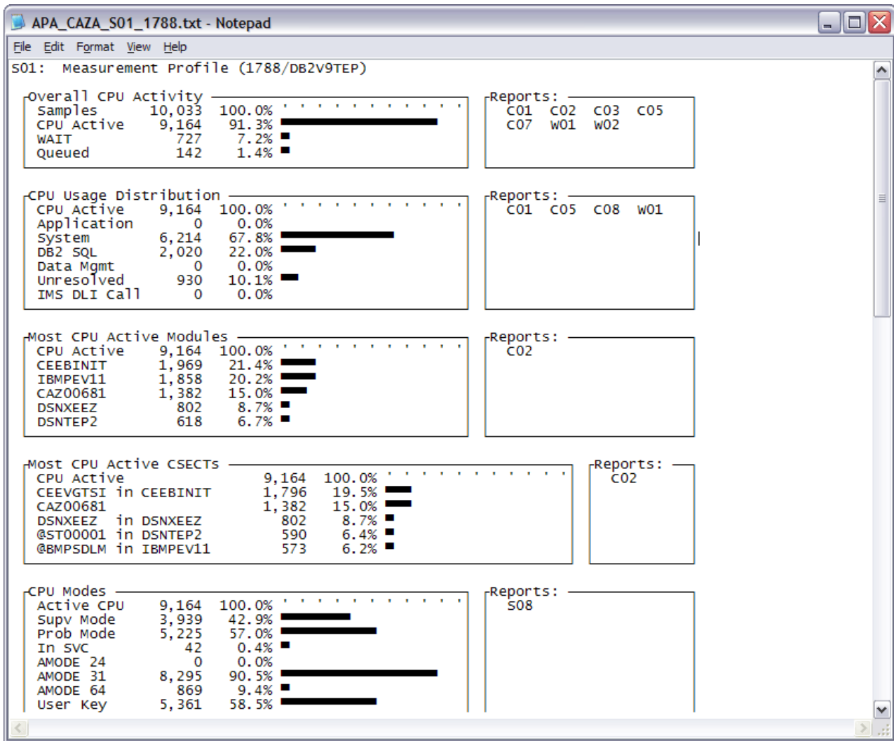
Figure 43. Saved Application Performance Analyzer GUI report sample
