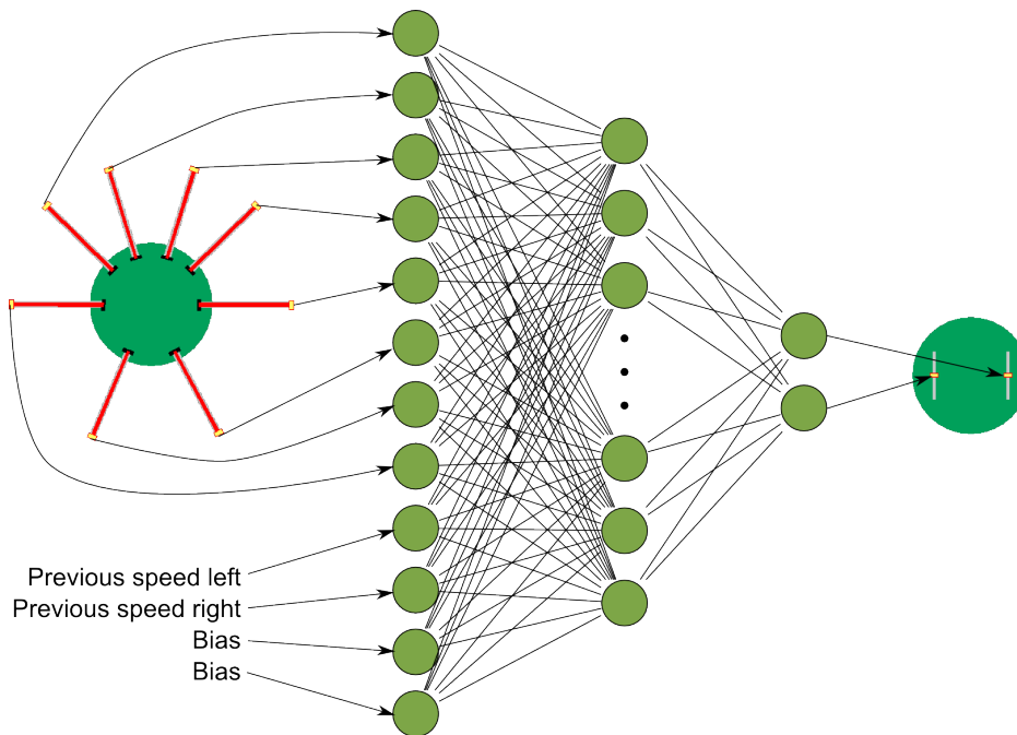
Figure 9.12: Neural network used for this exercise
