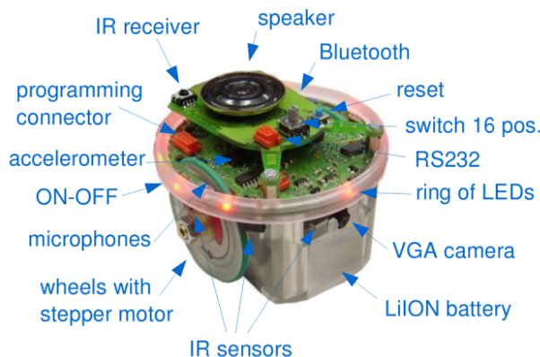
Figure 4.4: Model of an e-puck robot in Webots
