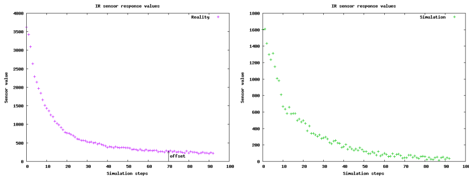
Figure 7.2: An e-puck is in front of a wall, and moves backwards. This figure plots the front right distance sensor value in function of the simulation steps. The left plot depicts the real values and the right plot depicts the simulated values.
