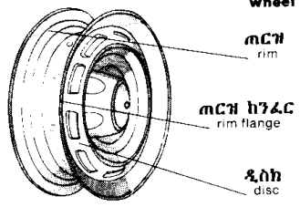
ሽከርካሪ wheel
