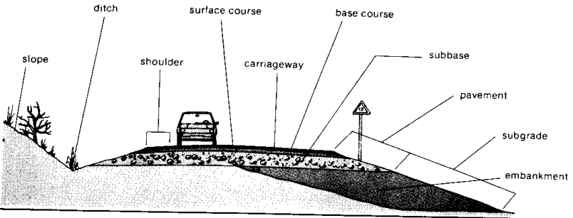
cross section of a road
