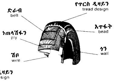
ሽከርካሪ wheel
