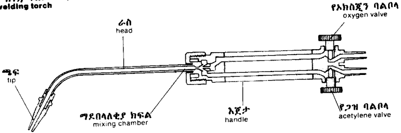
መቁረጫ ነበልባል cutting torch
