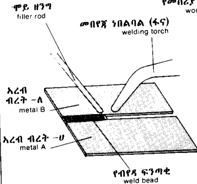
ገጣሚ ብዩዳ butt welding
