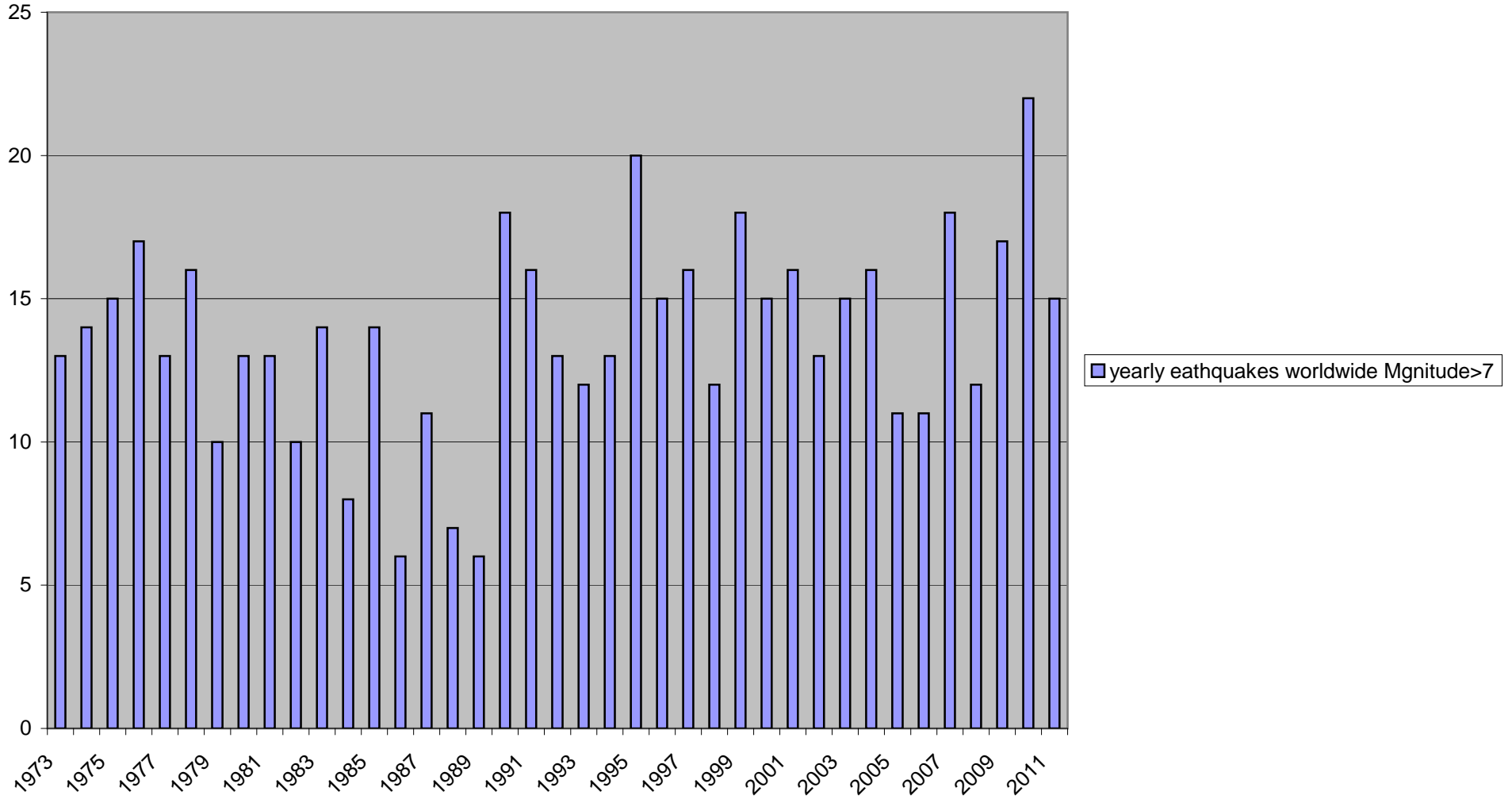
yearly eathquakes worldwide Magnitude>7 Source USGS/NEIC Database
